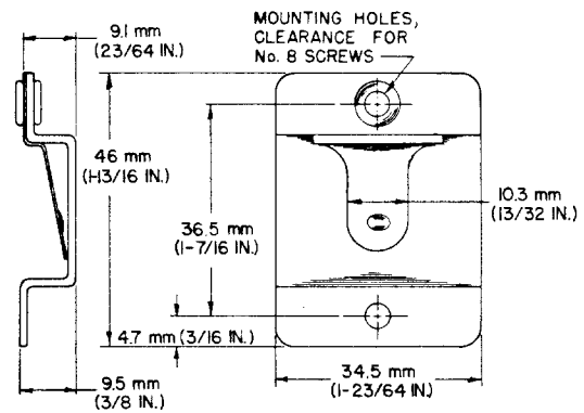
MOUNTING BRACKET FIGURE 3
