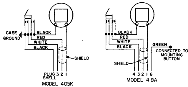
INTERNAL CONNECTIONS
