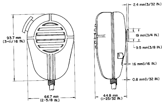
OVERALL DIMENSIONS
