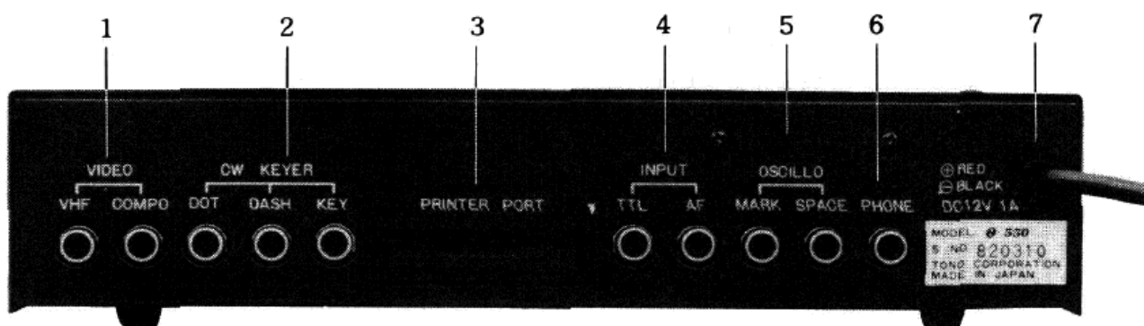
Figure 2. Rear Panel
