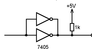
OUTPUT CIRCUIT (DATA STROBE)
