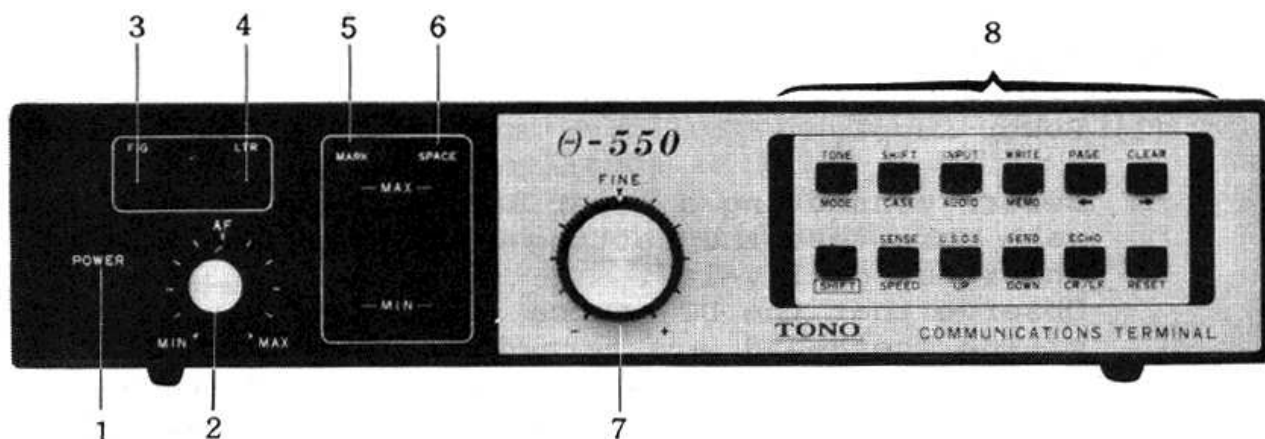
Figure 1. Front Panel
