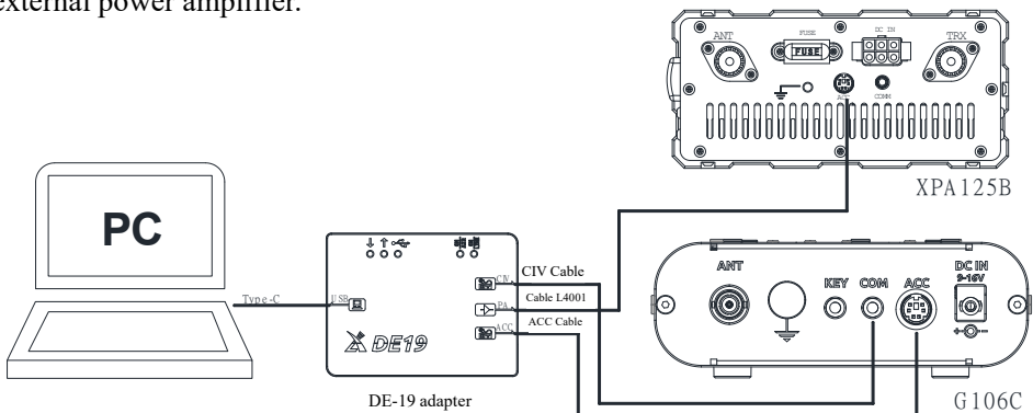
Fig. 2 Schematic Diagram of Connection Between DE-19 and G106C\XPA125B
