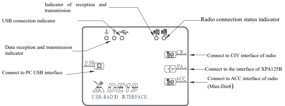
Fig. 1 Description of DE-19 Interface
