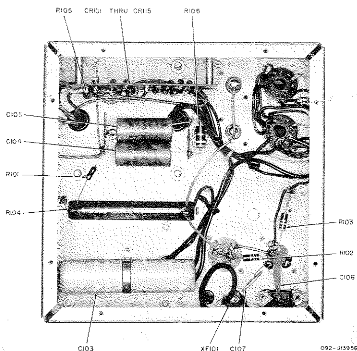
Bottom View P-26 Power Supply.
