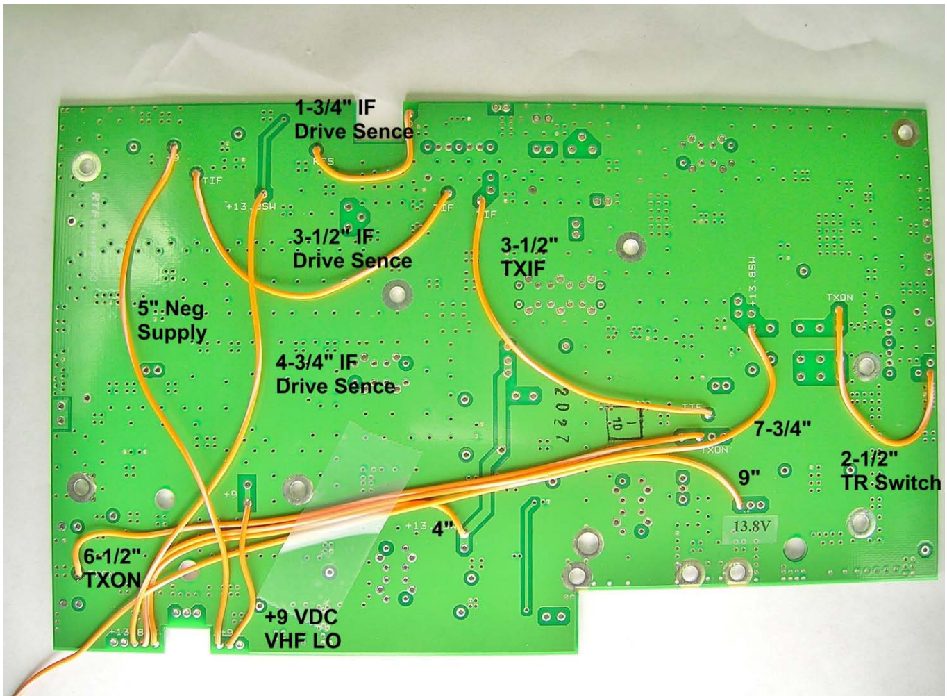
Bottom Side Board Wiring
