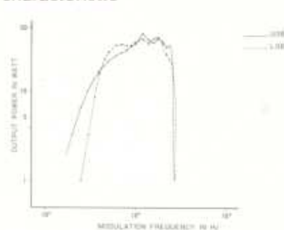
Transmitting frequency characteristic
