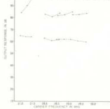
Image ratio and IF interference ratio
