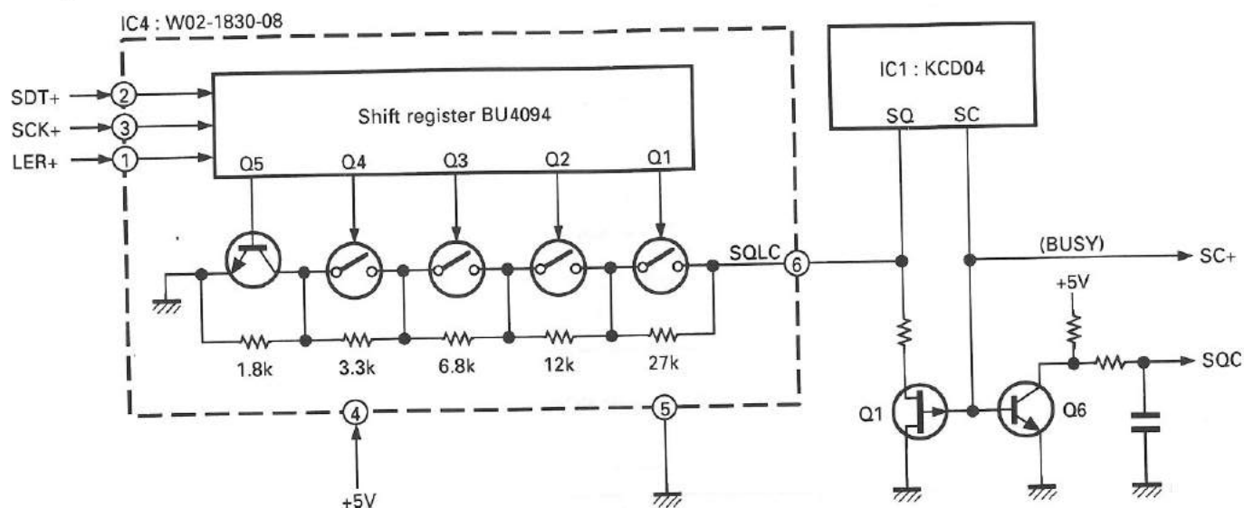
Fig. 16 Squelch circuit
