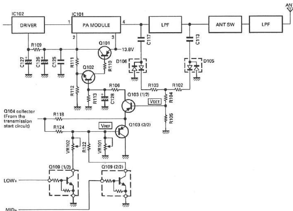
Fig. 6 APC circuit
