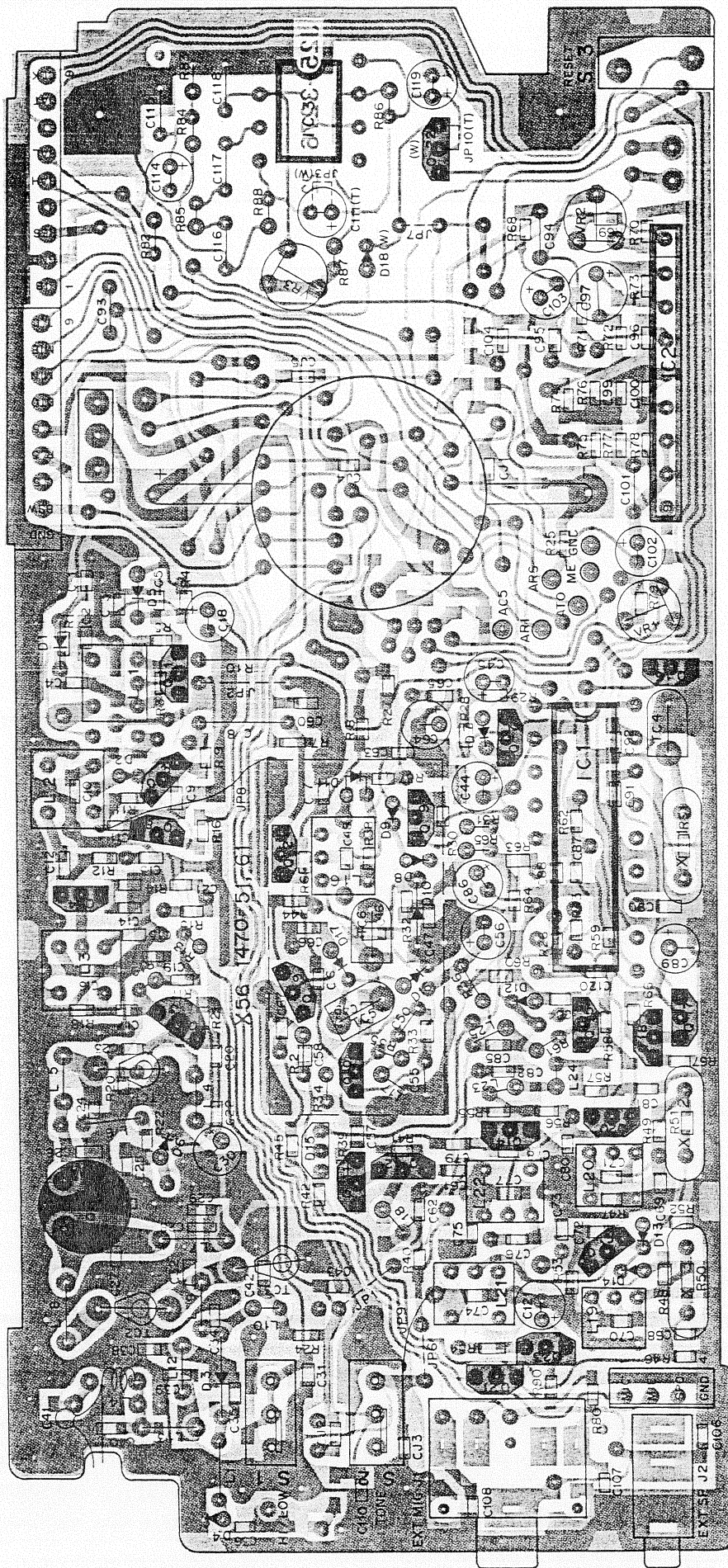
TX UNIT (X56-1470-XX) (-51 : T, -61 : W) Component side view
