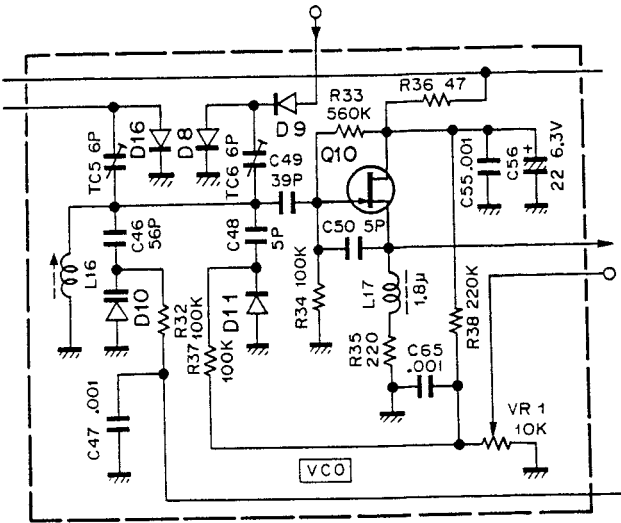
Fig. 6 VCO circuit
