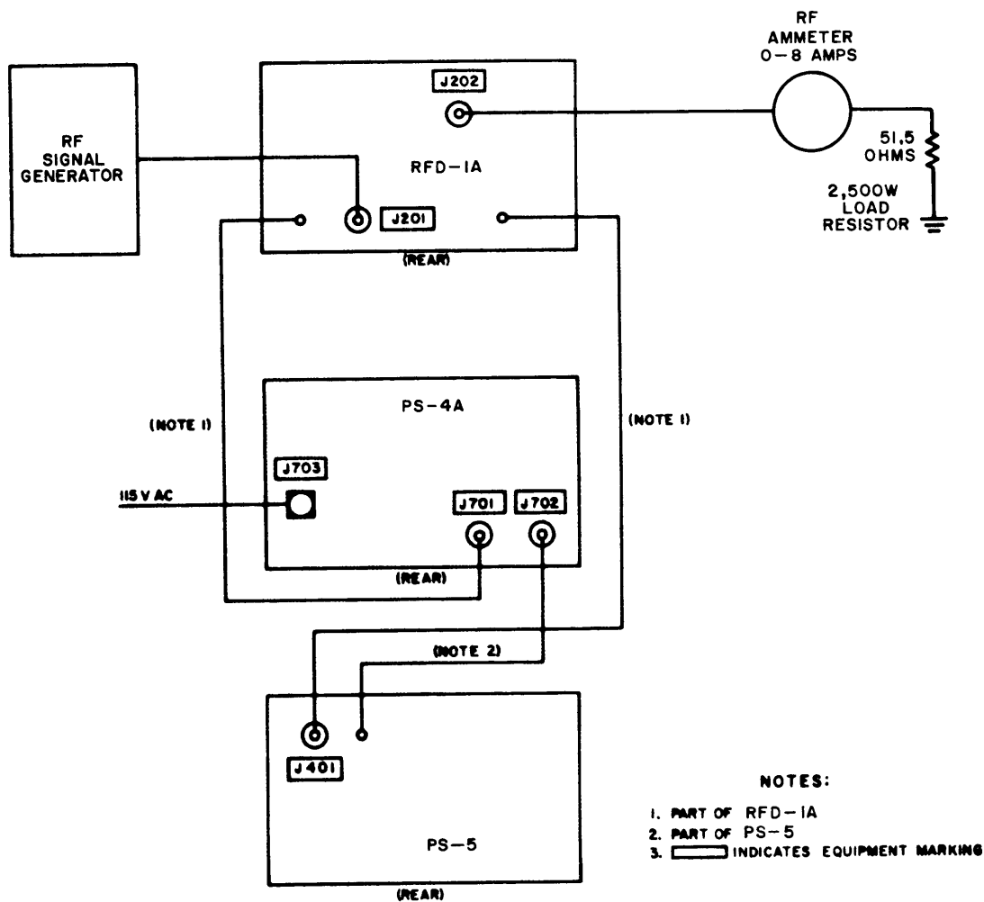
Figure 5-1. Test Setup for Trouble-Shooting PAL-1K(A)
