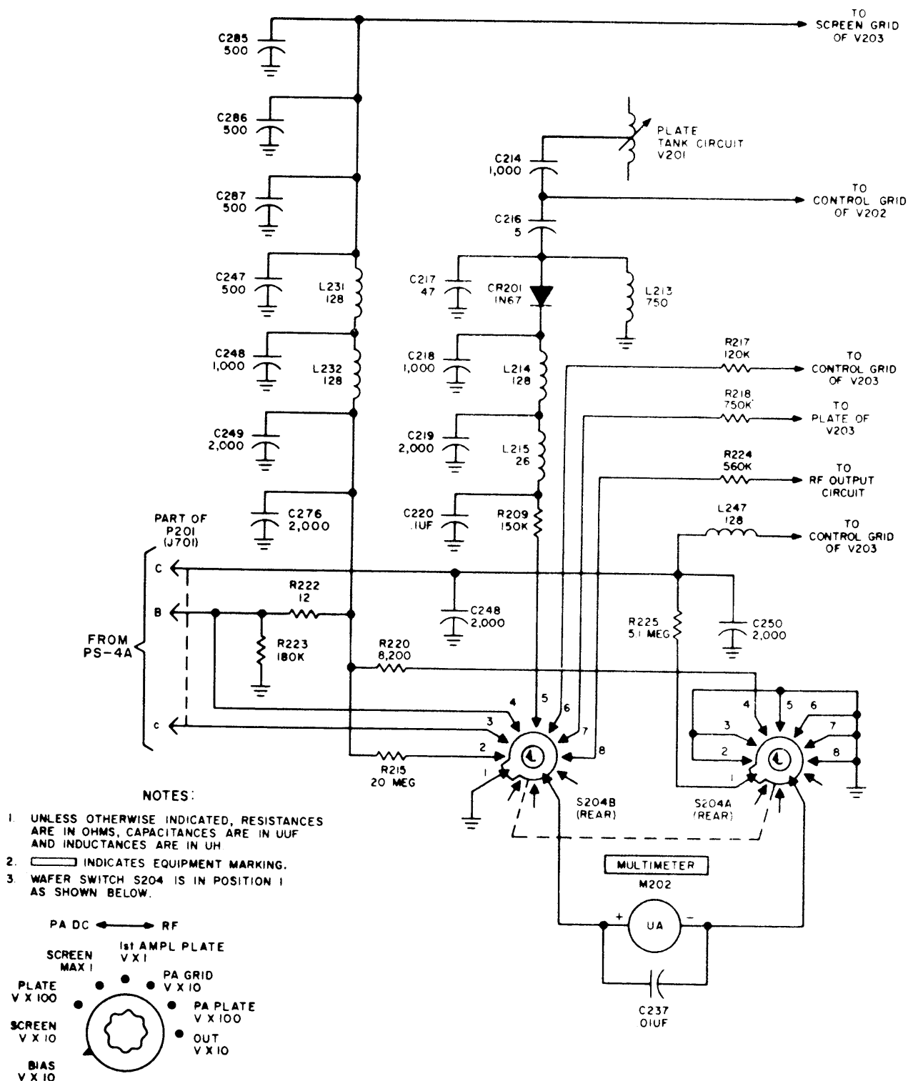
Figure 4-5. Simplified Schematic Diagram, Meter Circuit, RFD-1A
