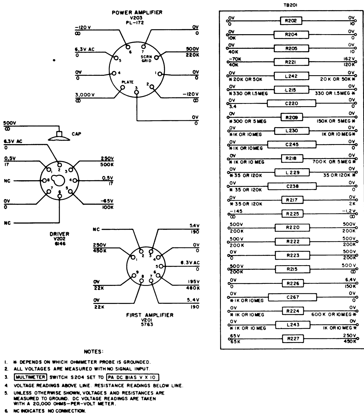
Figure 5-2. Voltage and Resistance Diagram, RFD-1A
