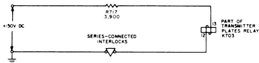
A. EQUIVALENT SCHEMATIC DIAGRAM
