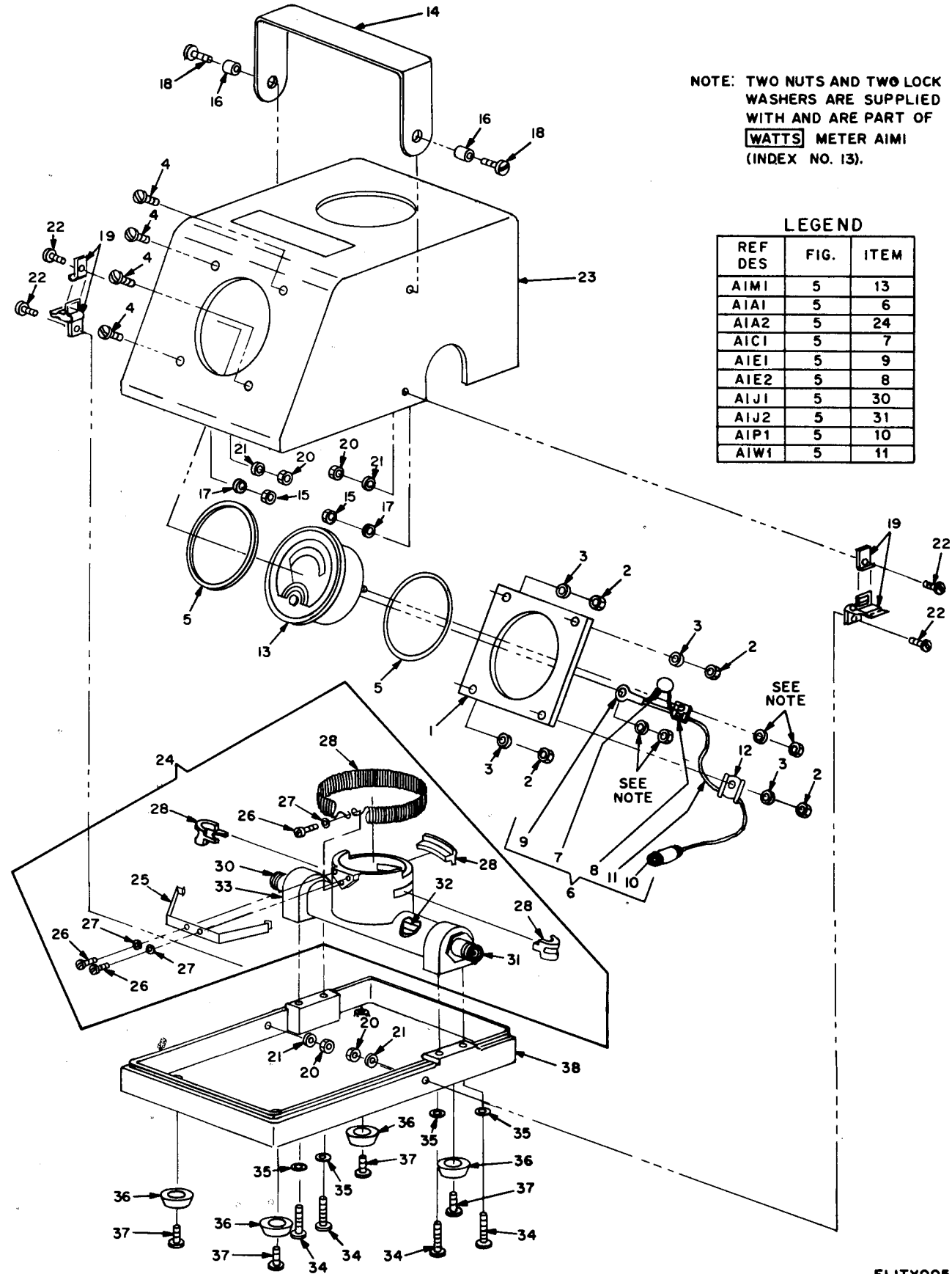
Figure 5. Wattmeter TS-1285/URM-120.
