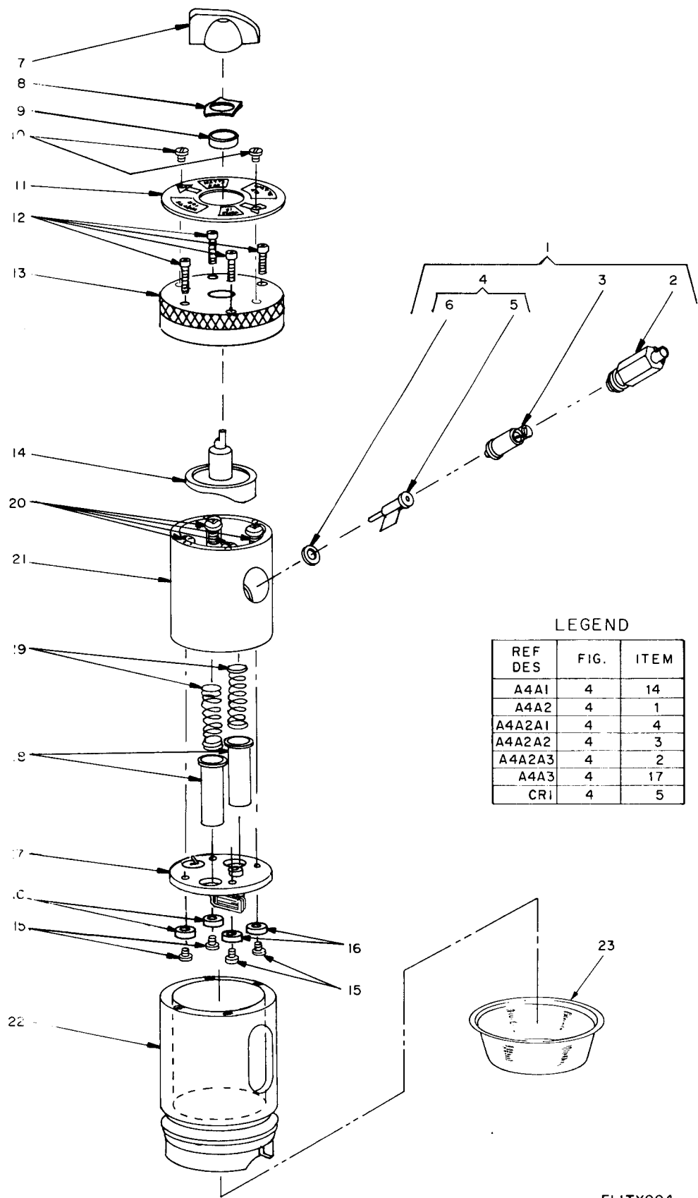
Figure 4. Coupler, Directional CU-755/URM-120.
