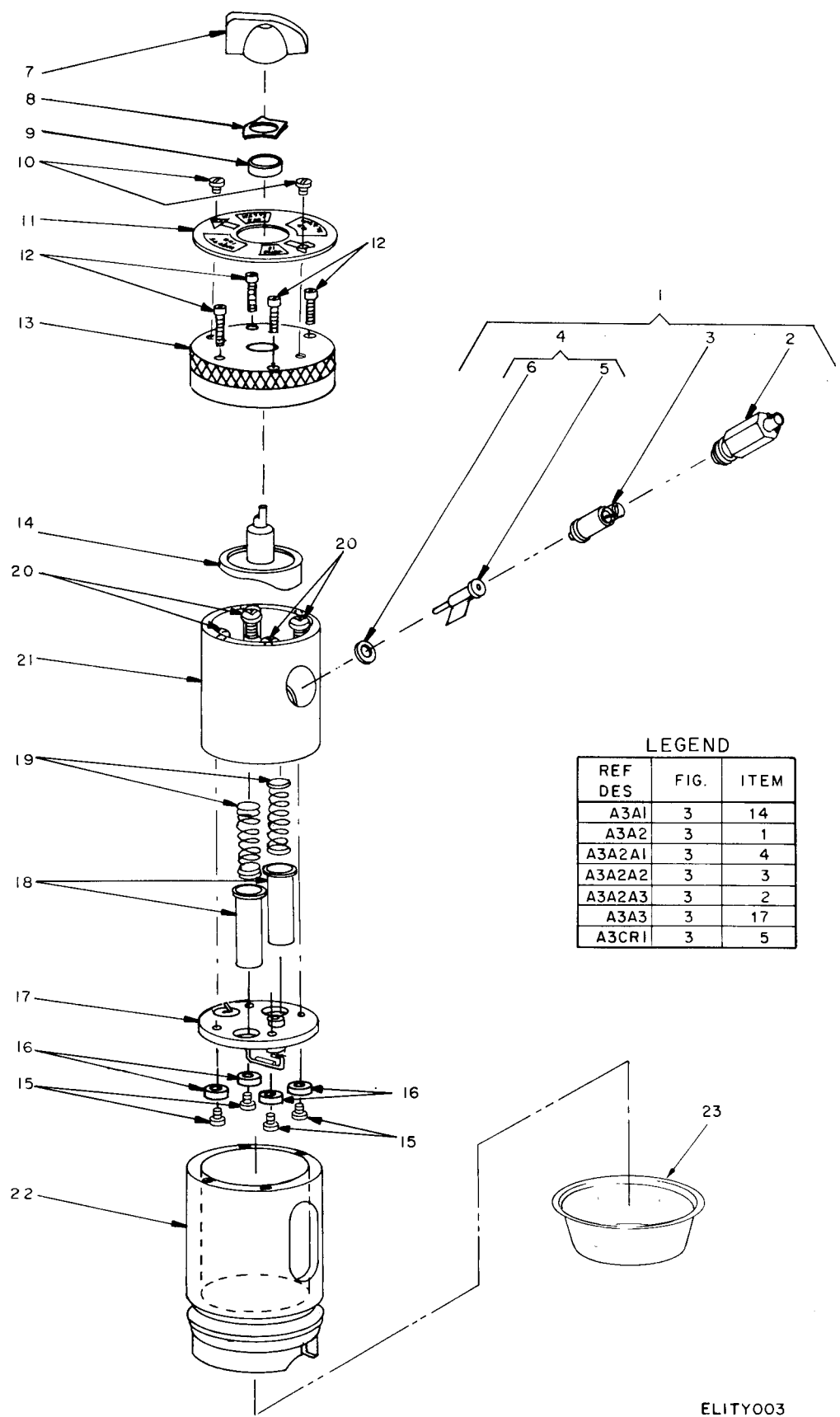
Figure 3. Coupler, Directional CU-754/URM-120.
