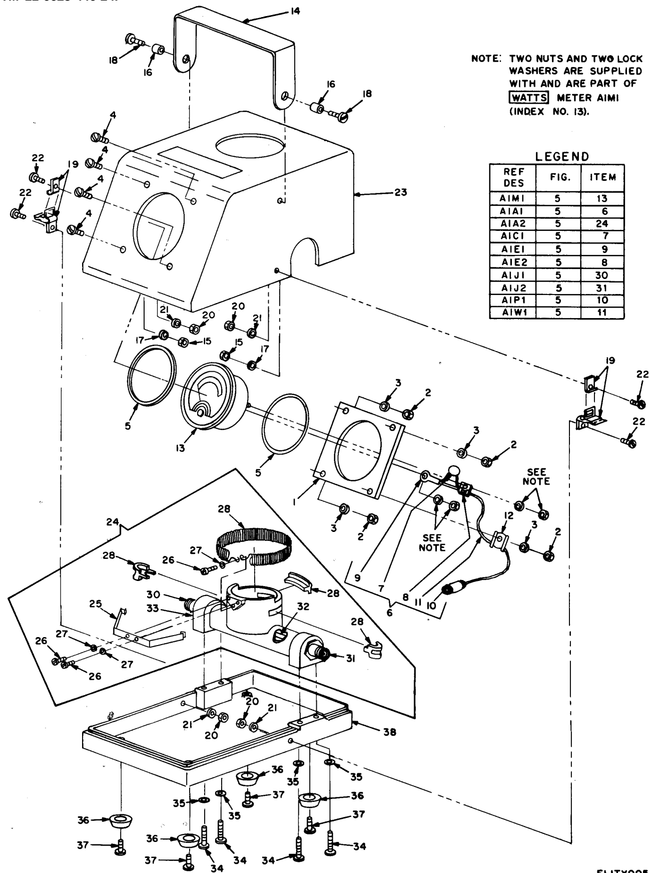
Figure 5. Wattmeter TS-1285/URM-120.
