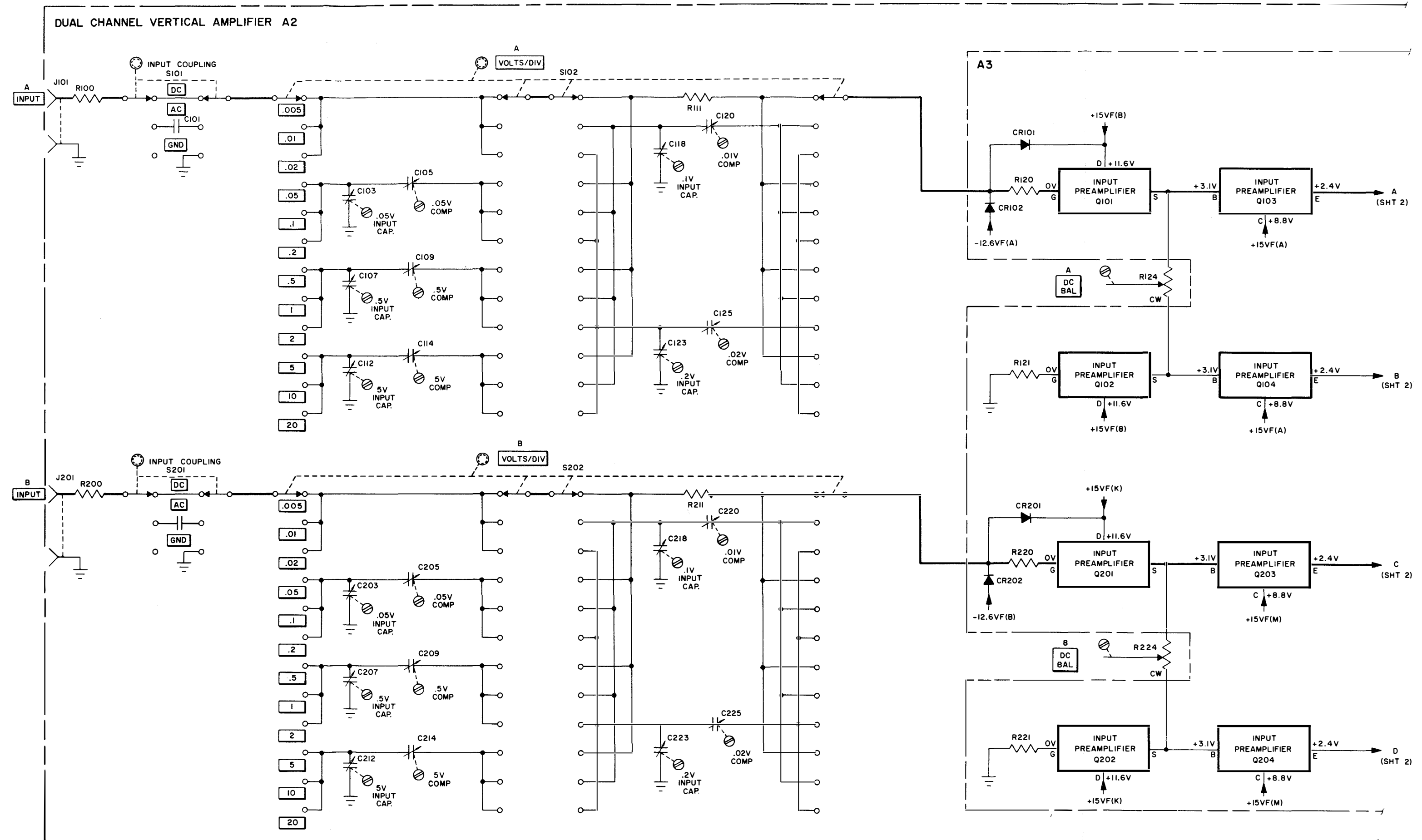
Figure 4-9. Dual Channel Vertical Amplifiers and Attenuator Functional and Servicing Block Diagram (Sheet 1 of 3)
