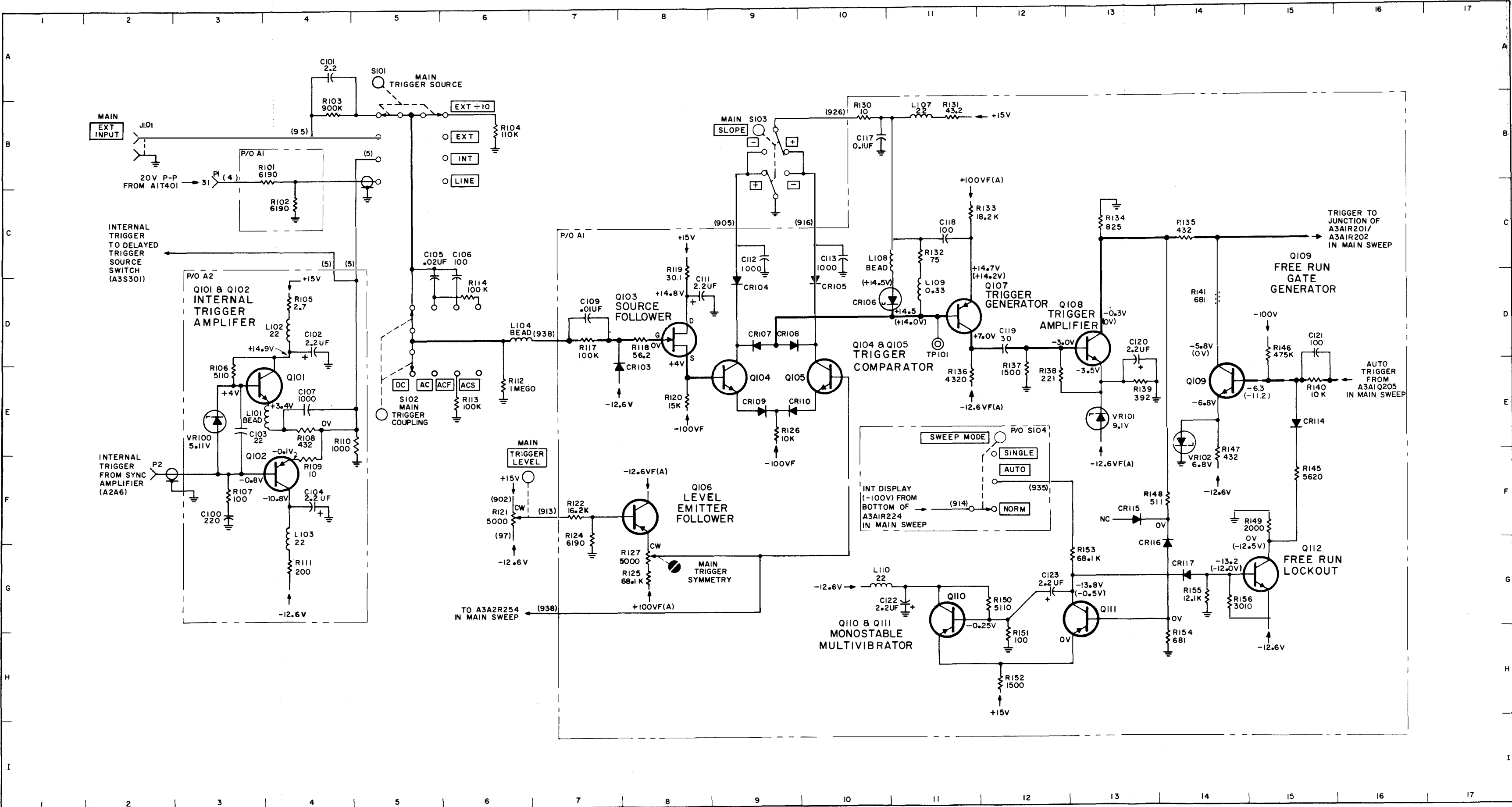
Figure 5-32. Time Base and Delay Generator Schematic Diagram (Sheet 1 of 5)
