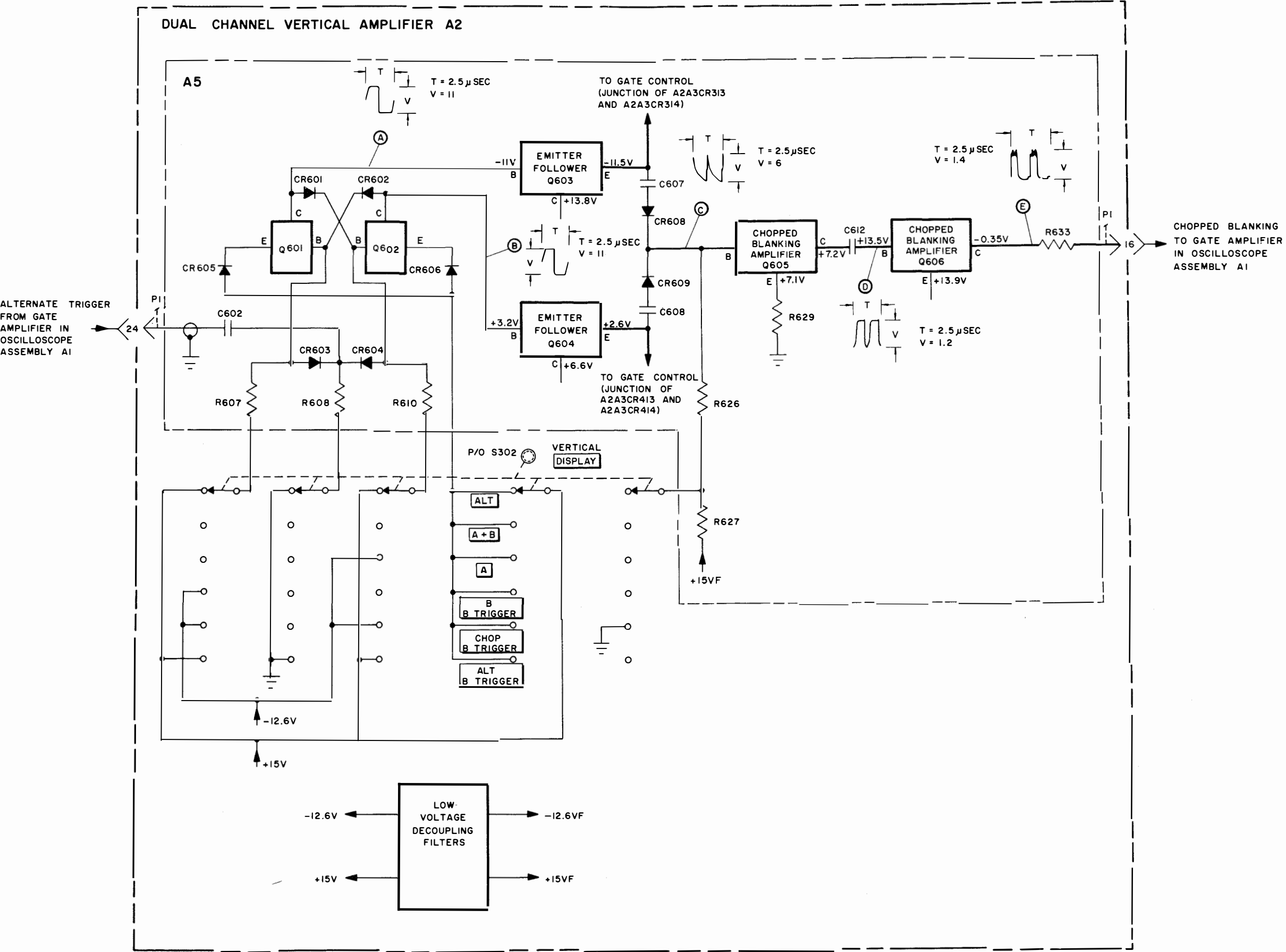
Figure 4-10. Multivibrator Functional and Servicing Block Diagram
