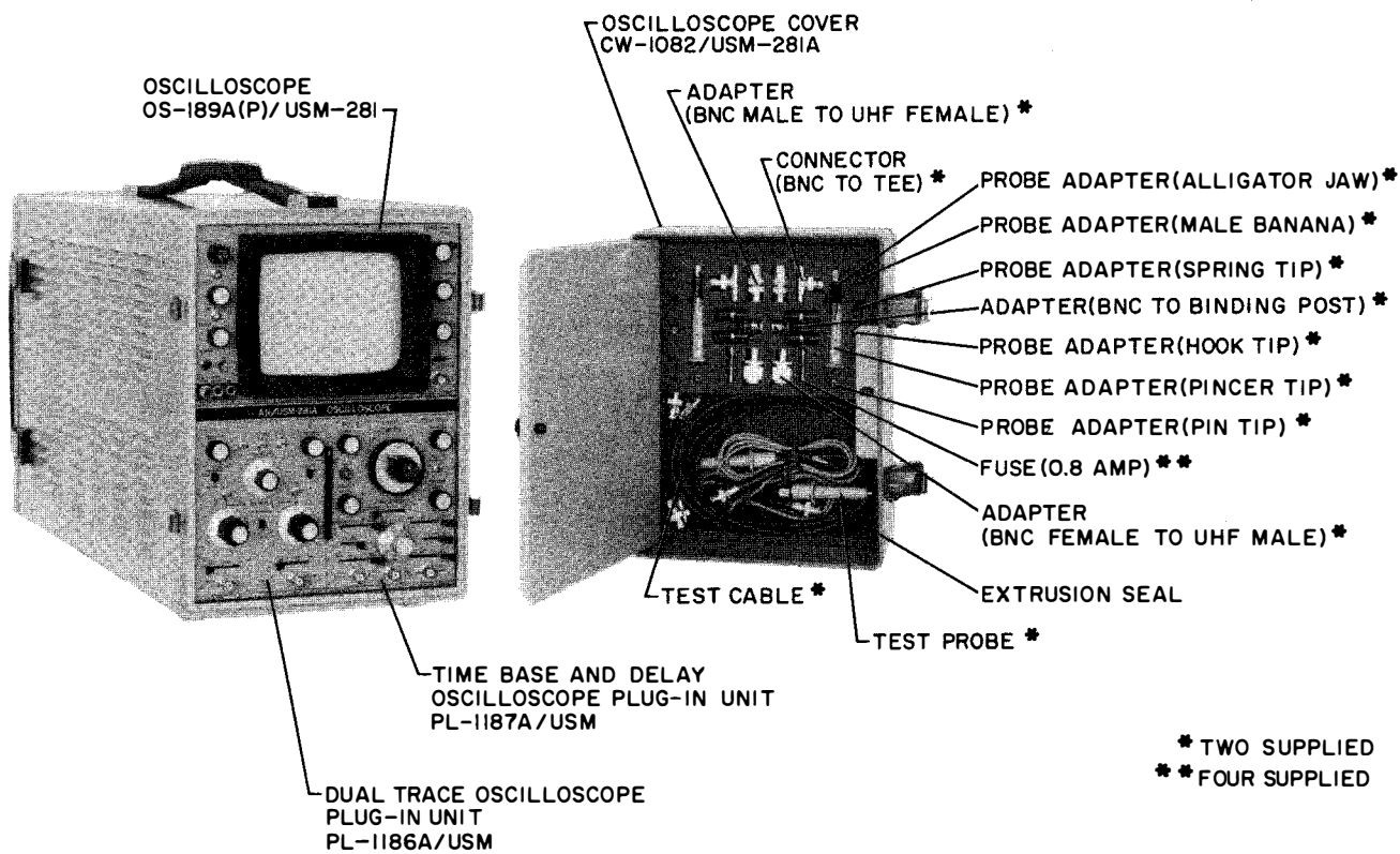
Figure 1-1. Oscilloscope AN/USM-281A
