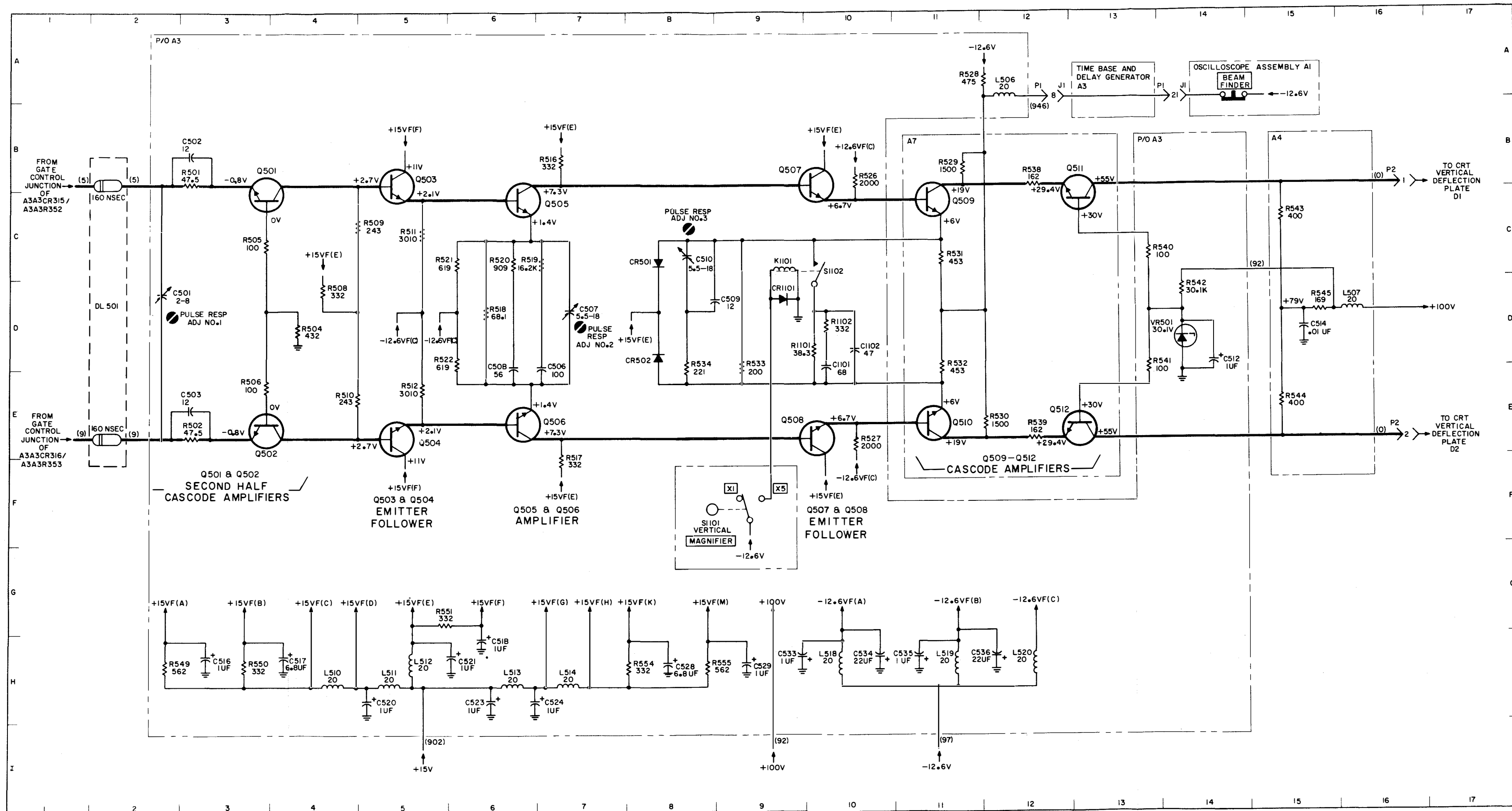
Figure 5-31. Dual Channel Vertical Amplifier Schematic Diagram (Sheet 3 of 5)
