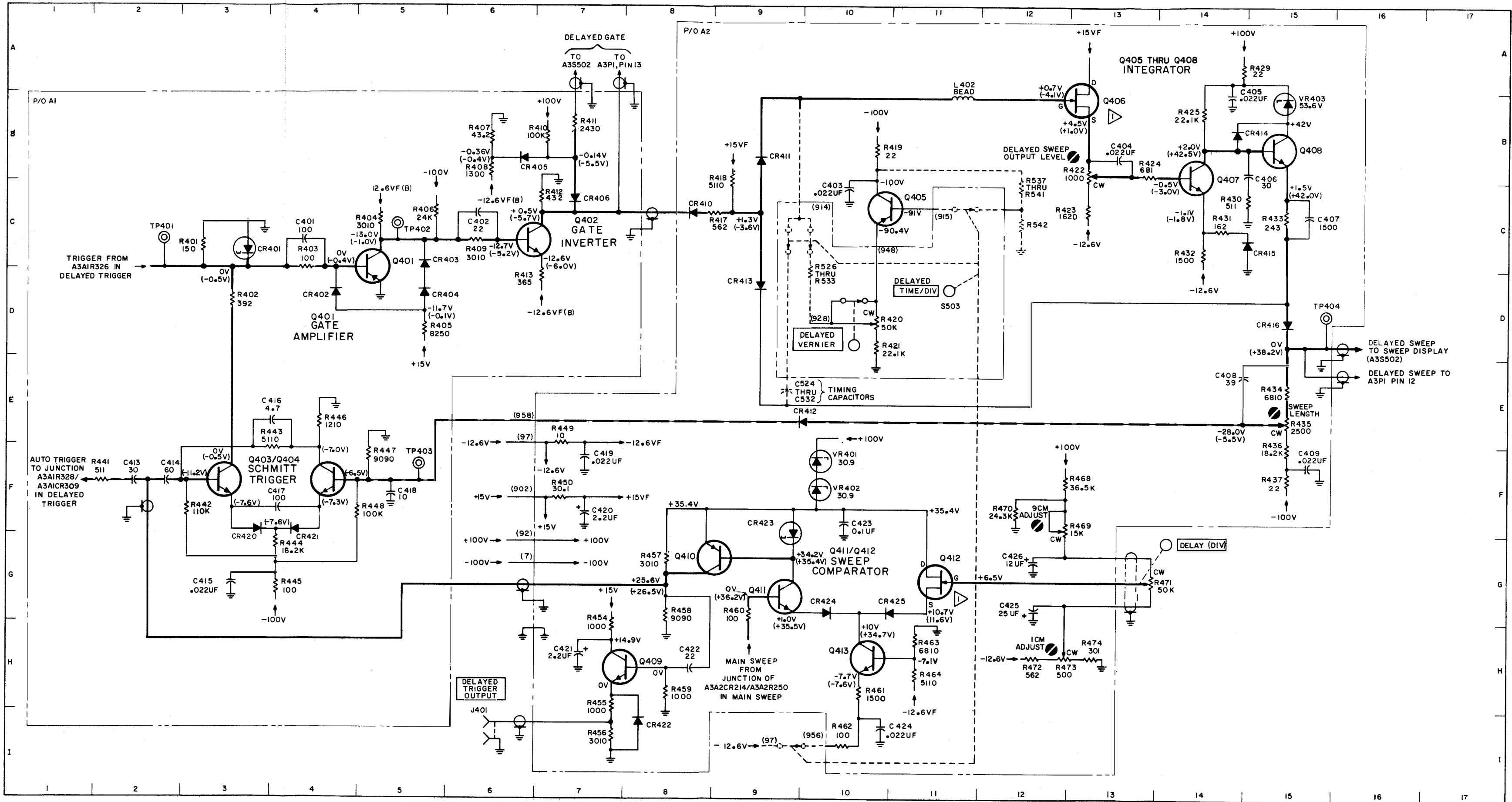
Figure 5-32. Time Base and Delay Generator Schematic Diagram (Sheet 4 of 5)
