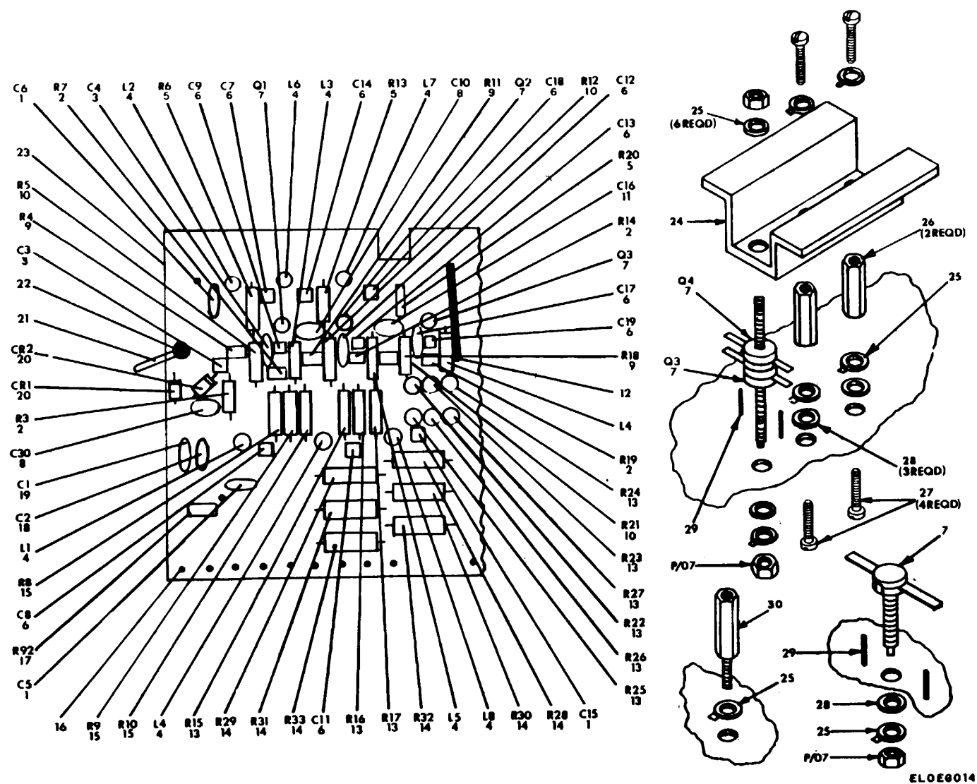
Figure 14. Circuit Card Assembly, Left (A9A1)
