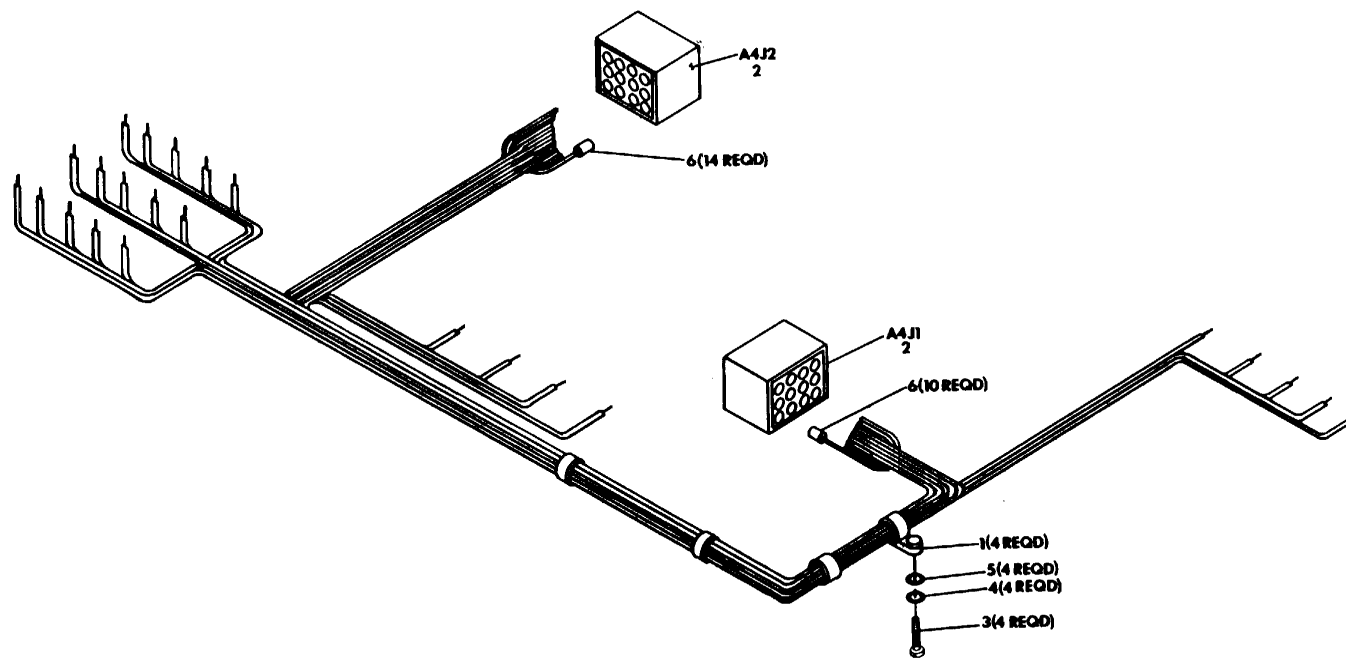
Figure 10. Harness Assembly.
