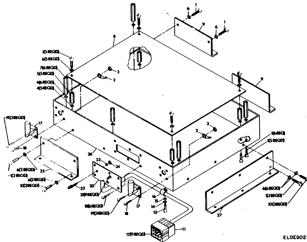
Figure 23. Box Assembly (P/OA8)
