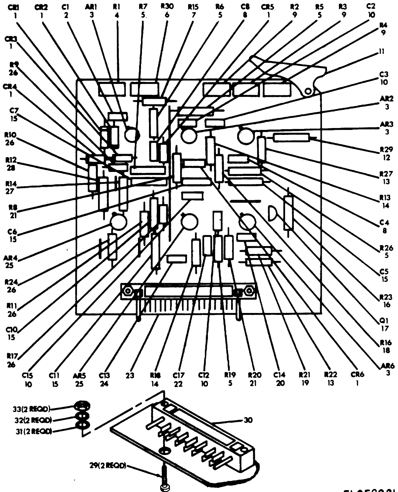
Figure 21. Circuit Card Assembly (A6).
