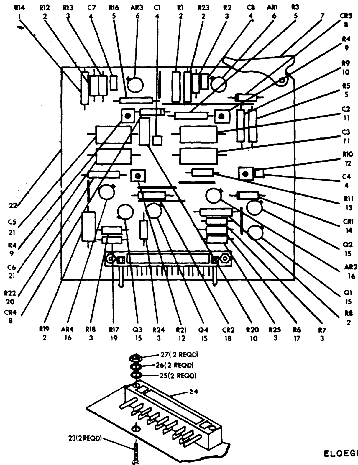
Figure 20. Circuit Card Assembly (A11).
