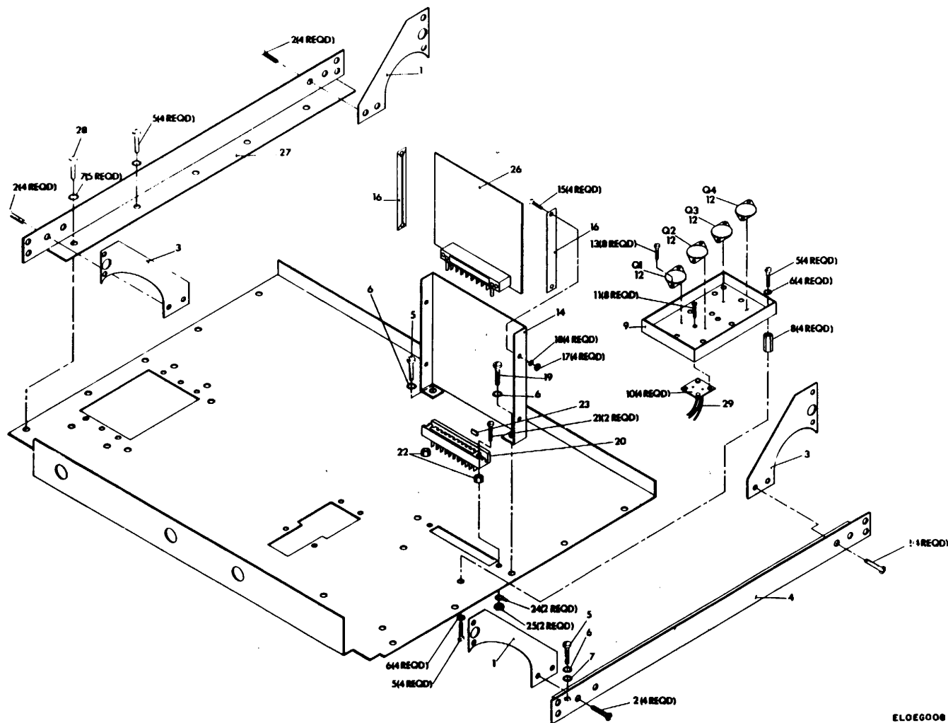
Figure 8. Top Chassis Assembly.
