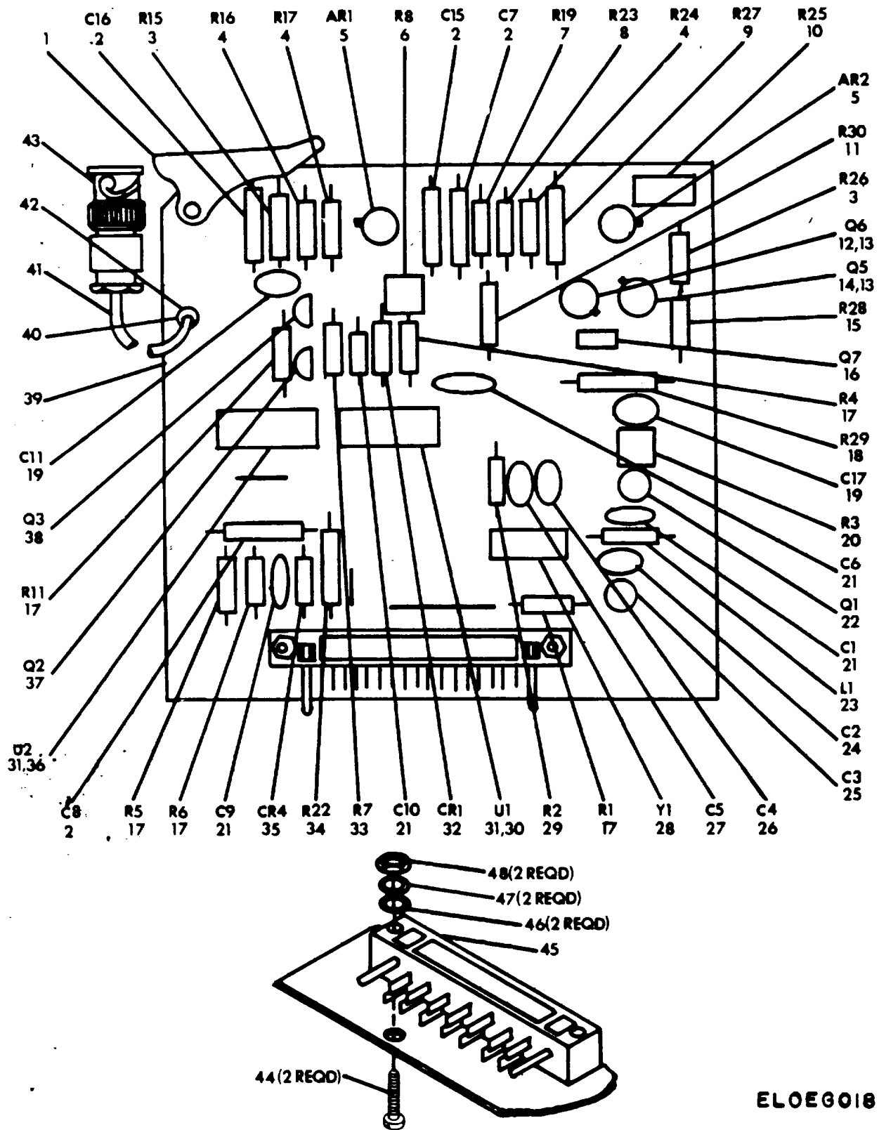
Figure 18. Circuit Card Assembly (A5).
