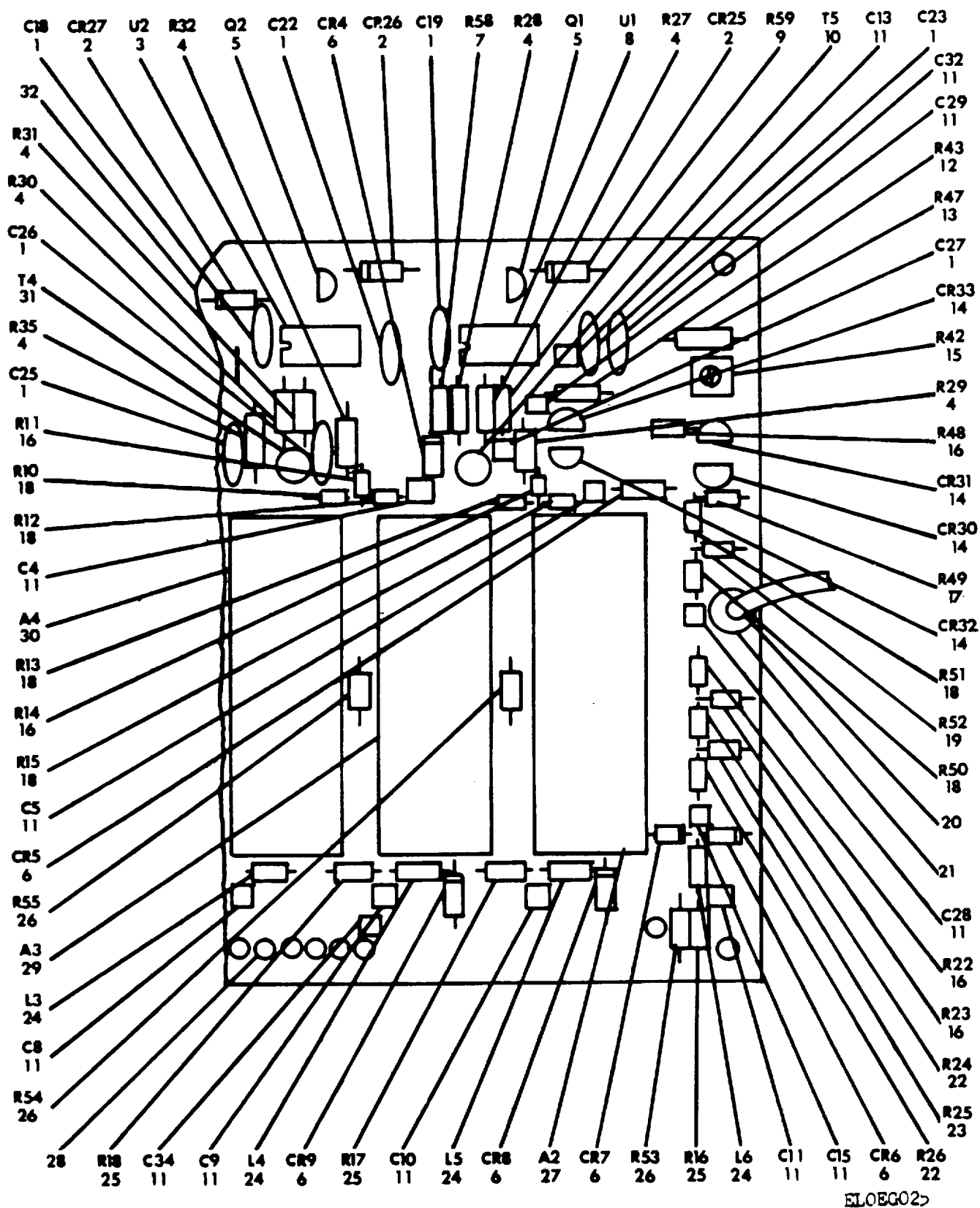
Figure 25. Circuit Card Assembly Left (A8A3).
