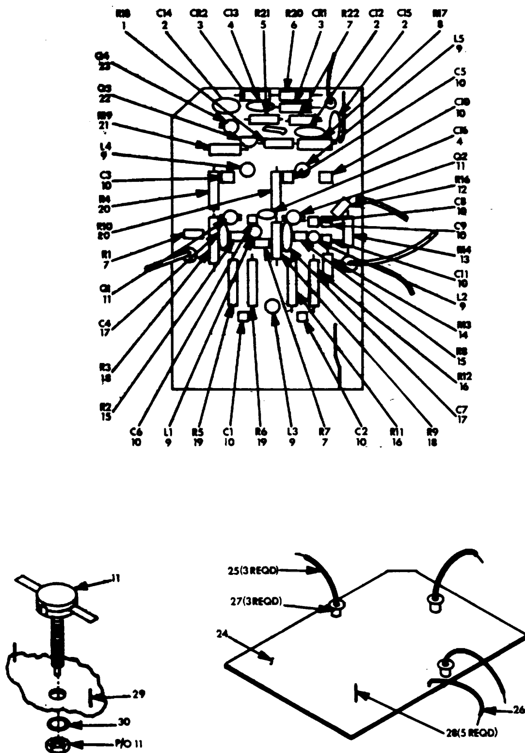
Figure 16. Circuit Card Assembly (A9A2).
