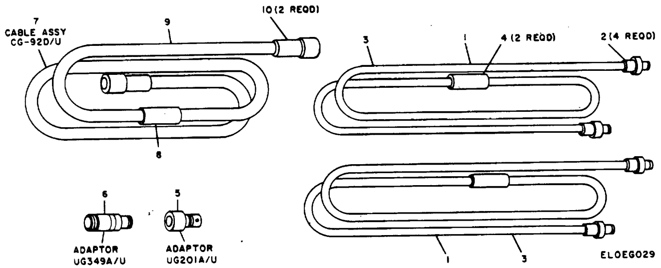
Figure 28. Cable Assemblies.
