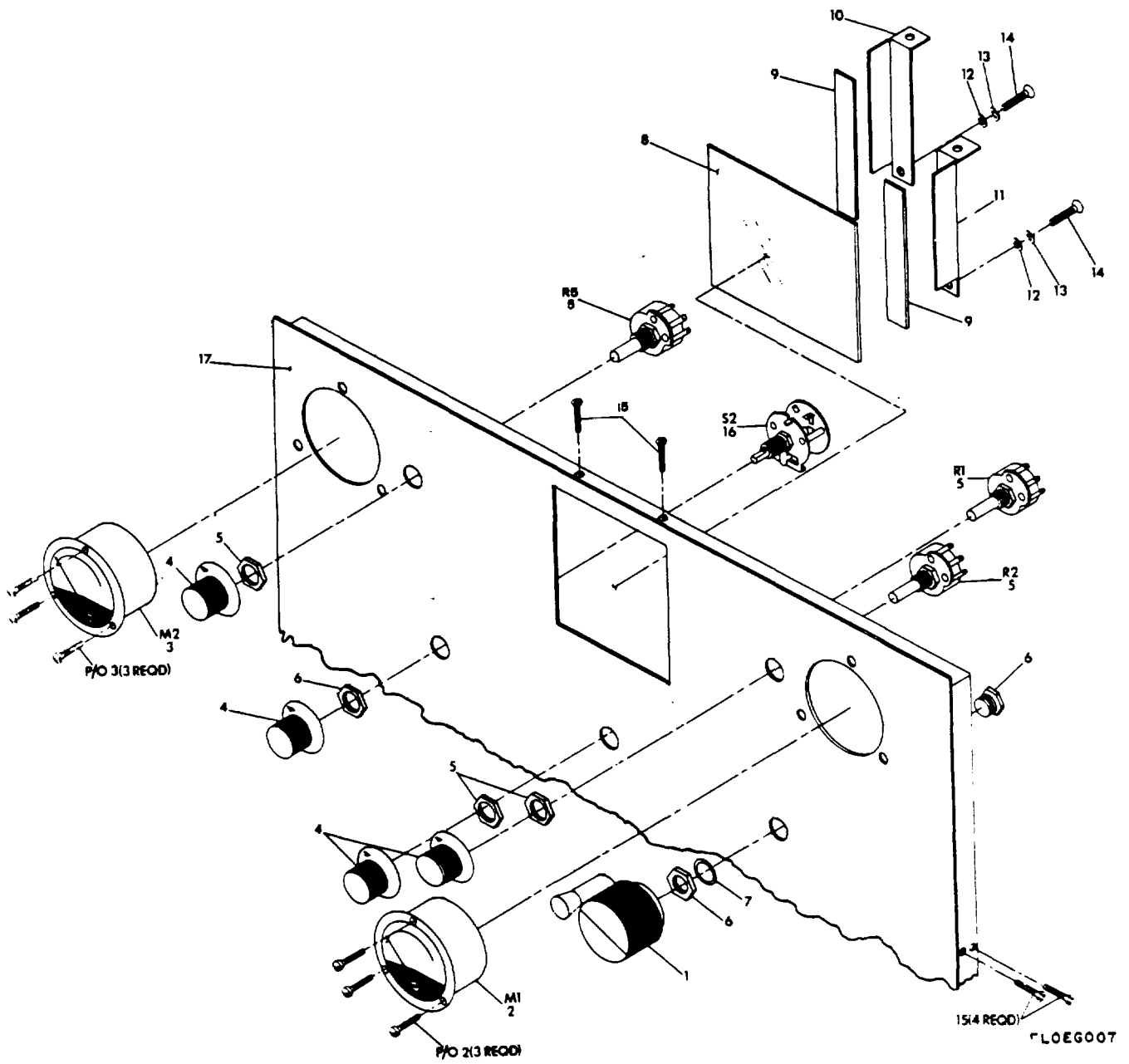
Figure 7. Panel Assembly Front (Top).
