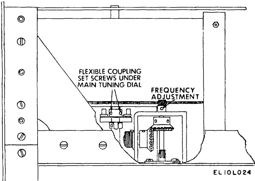
Figure 7-16. Tuning dial adjustment
