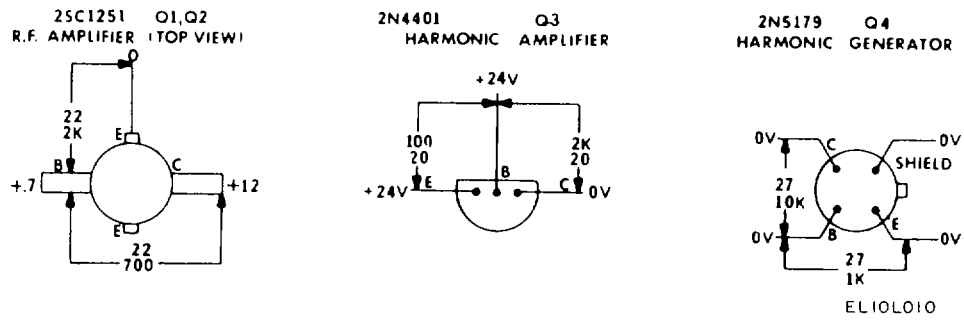
Figure 7-7. Rf preamplifier board A9A2, circuit measurements.
