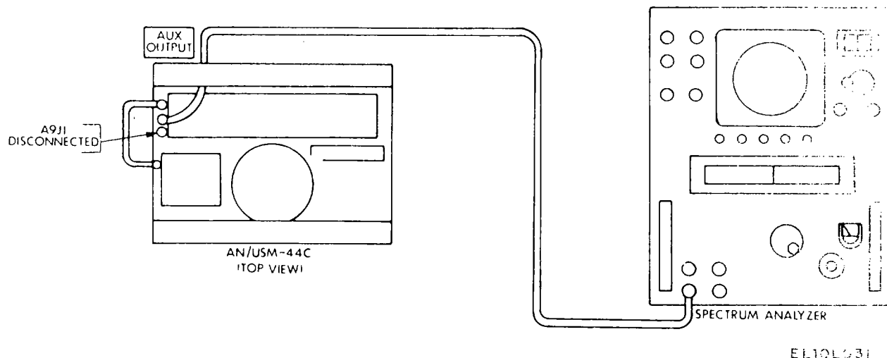
Figure 7-24. Marker amplitude adjustment, test setup.
