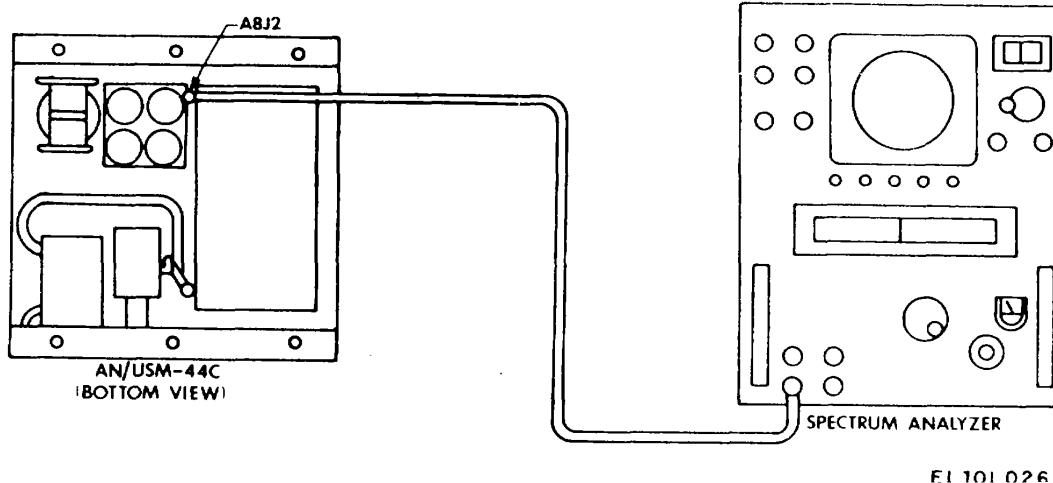
Figure 7-19. Rf divider A8, alignment test setup
