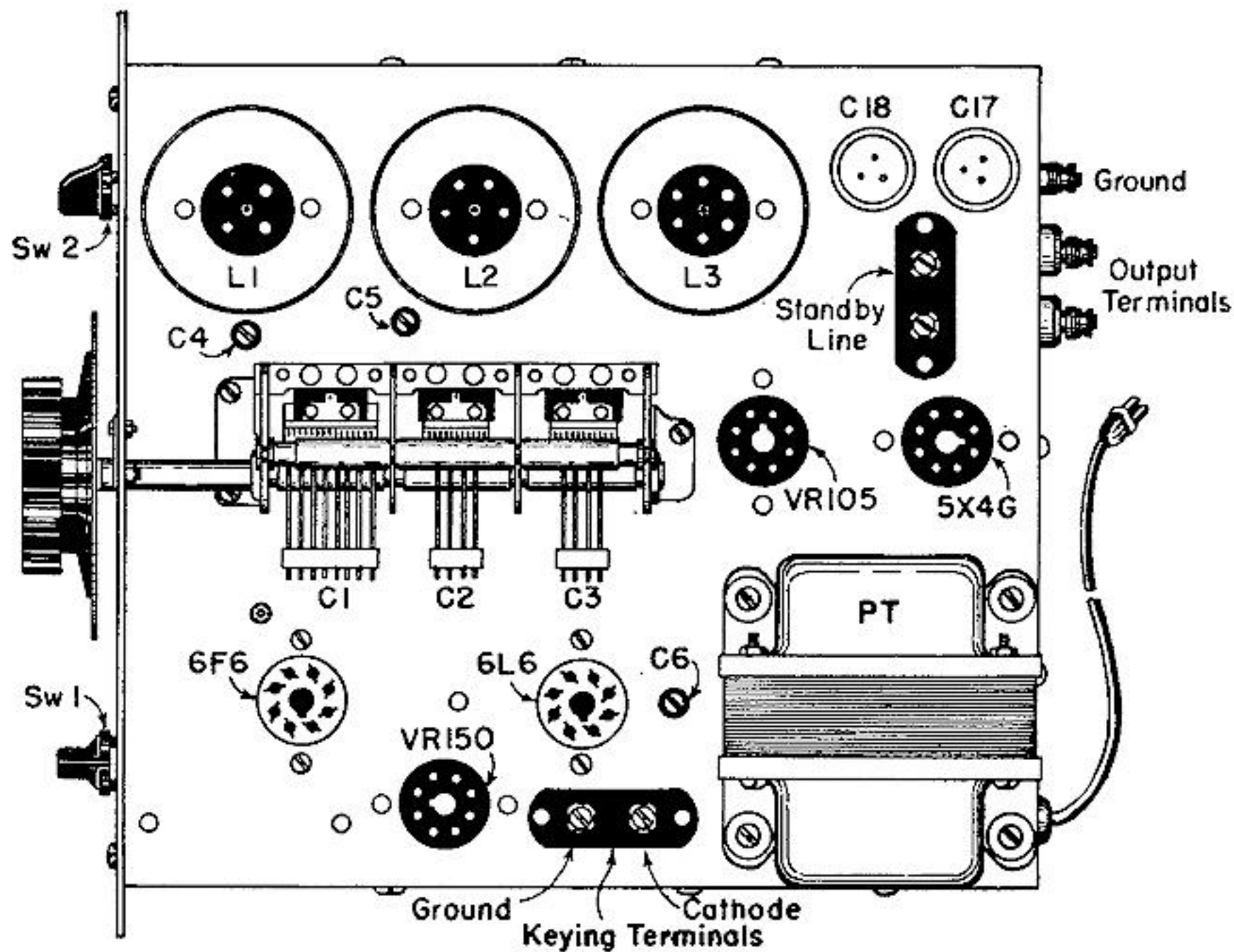
Figure 5 — DeLUXE MODEL (OLD) — TOP VIEW
