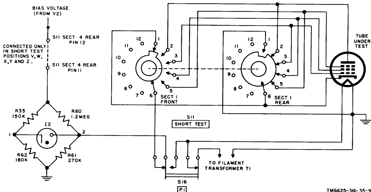
Figure 9. Short and filament continuing test circuit of Test Set, Electron Tube TV-2(*)/U, simplified schematic diagram.
