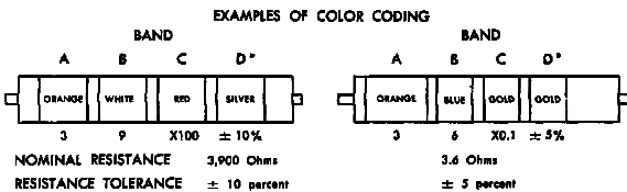
Figure 24. MIL-STD resistor color code markings.
