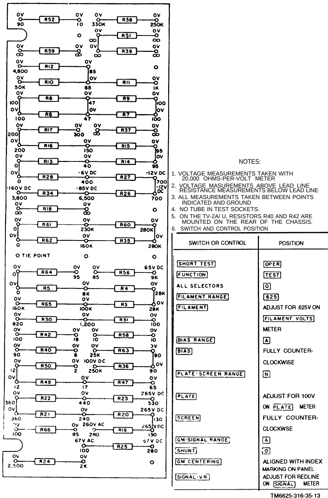
Figure 13. Resistor mounting board voltage and resistance diagram.
