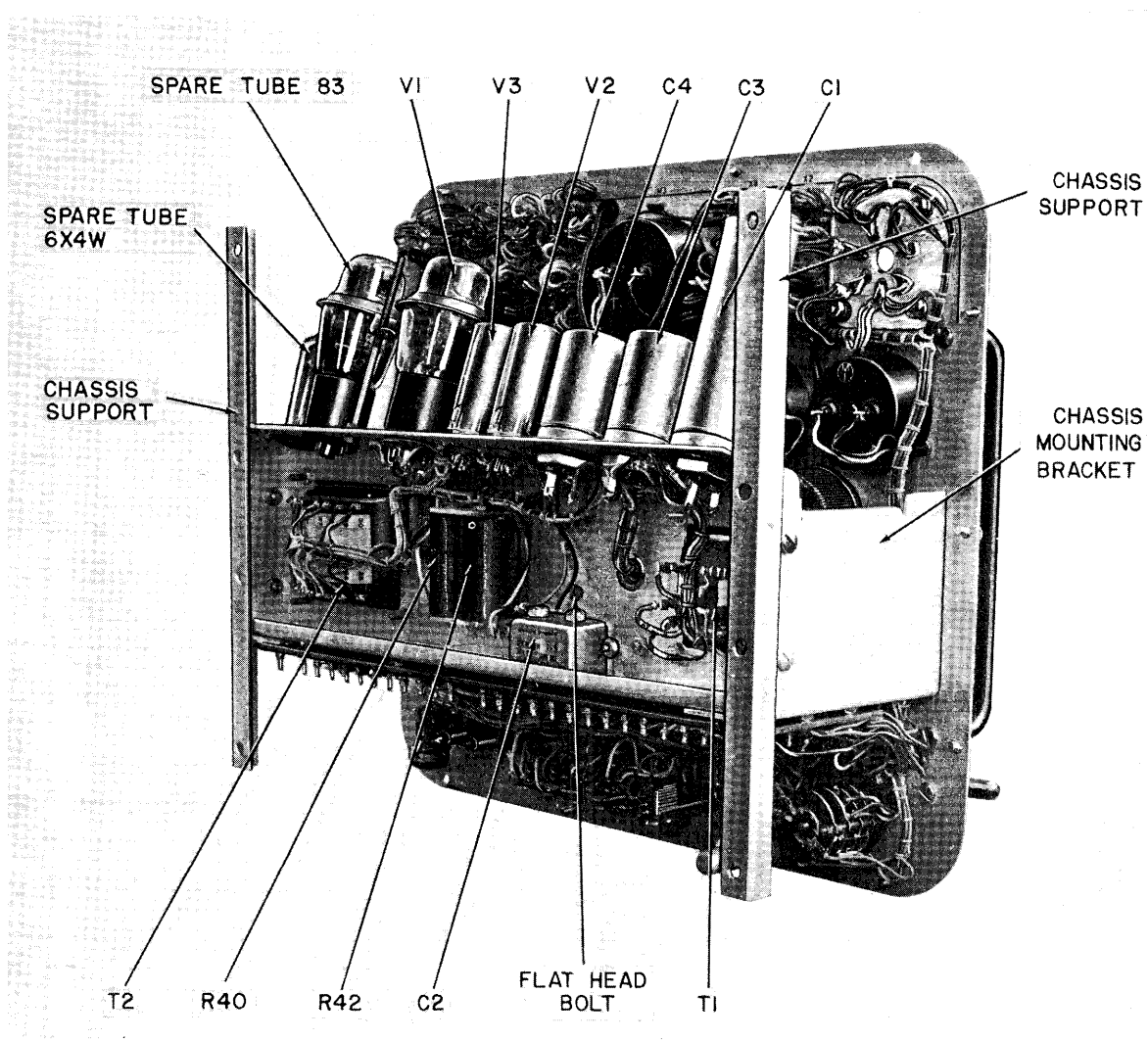
Figure 18. Rear of chassis of Test Set, Electron Tube TV-2A/U, location of parts.
