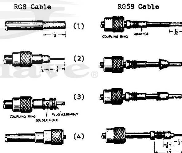
Figure 2-2. Connector Assembly
