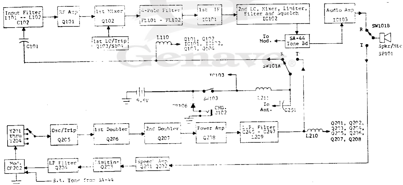
Figure 4-1. Block Diagram
