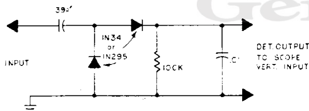
Figure 4-5. High-Impedance Detector
