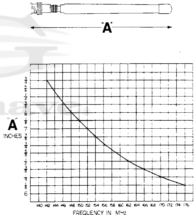
Figure 2-3. BNC-Mounting
