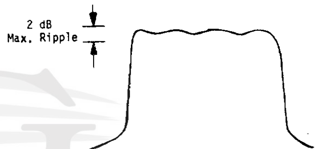
Figure 4-6. IF Response
