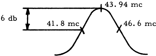
Fig. 5.5 - FL9 Response
