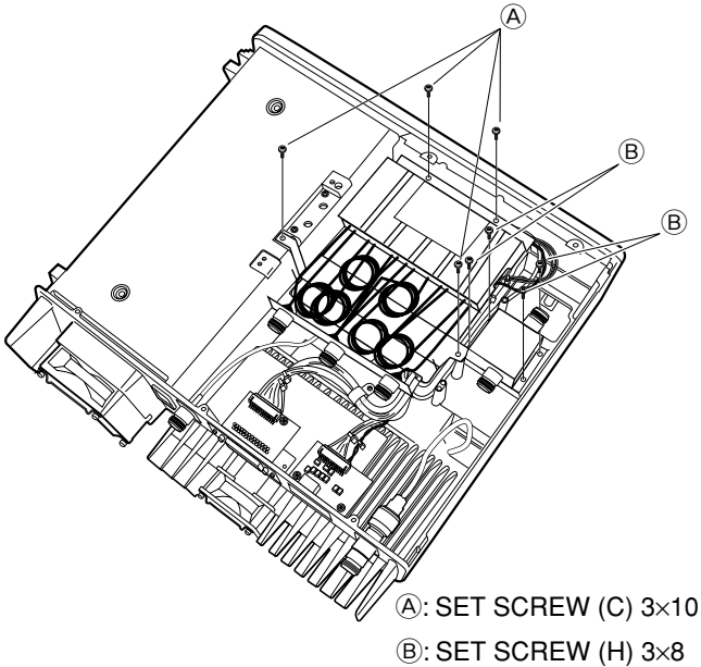
BOTTOM VIEW OF THE REPEATER
