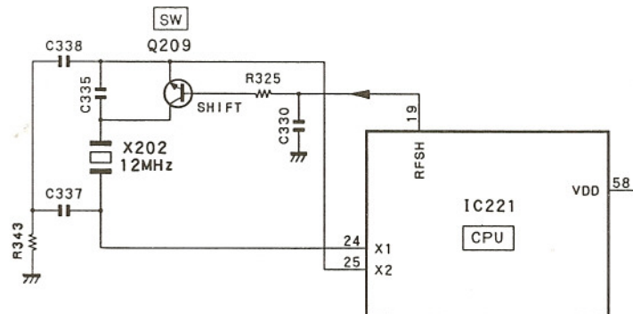
Fig. 9 CPU clock frequency shift
