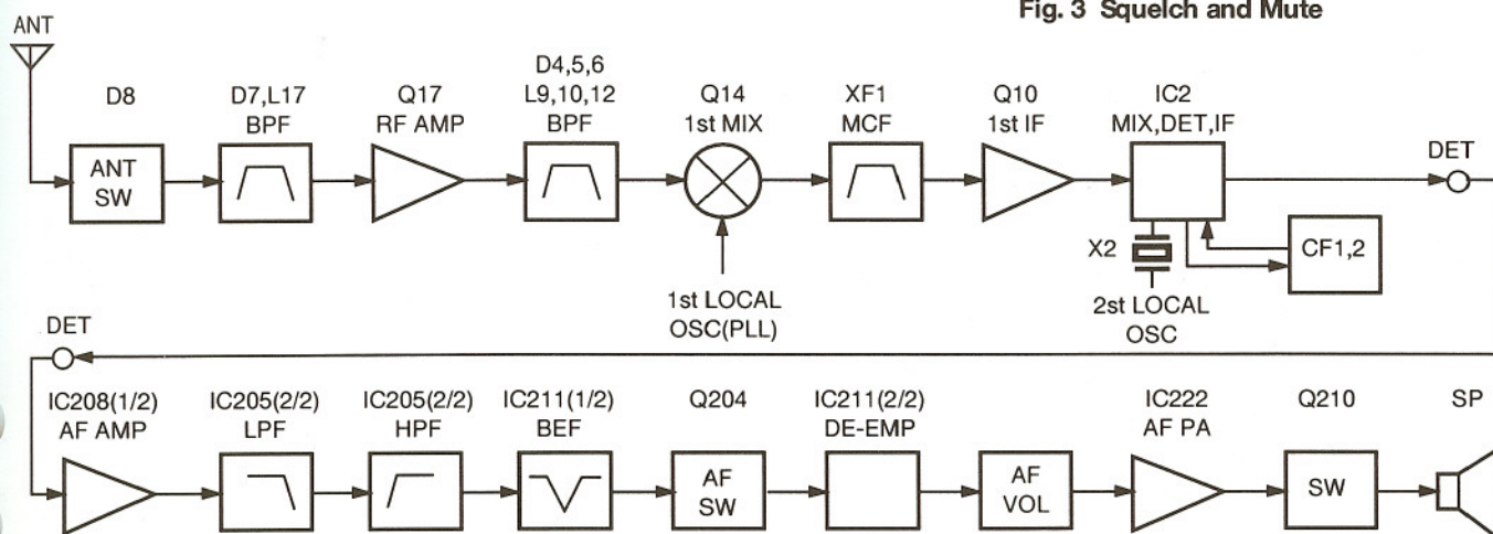
Fig. 2 Receiving system
