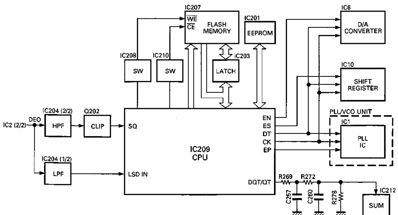
Fig. 7 Control unit block diagram
