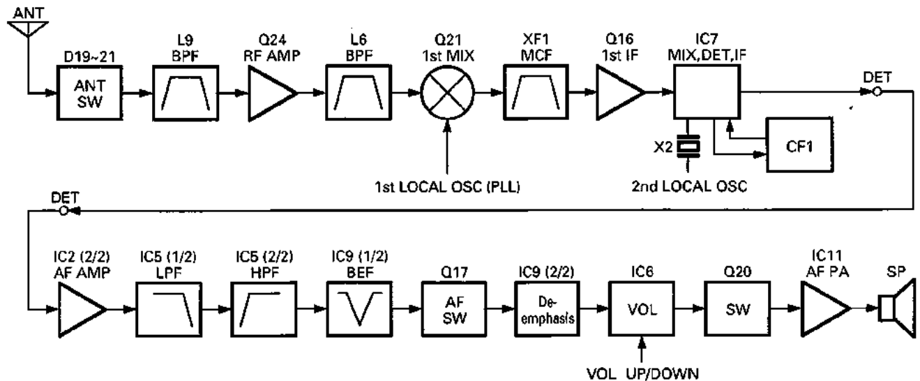
Fig. 2 Receiving system
