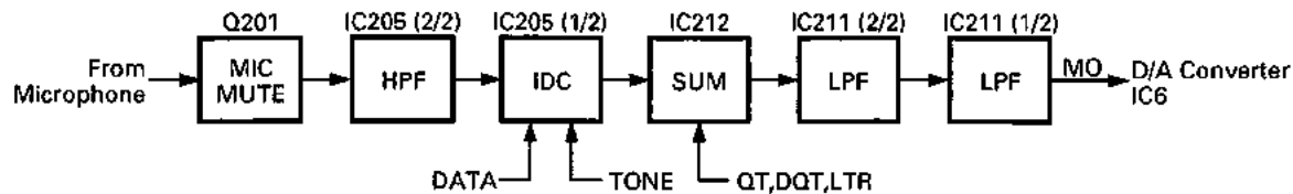
Fig. 3 Microphone amplification
