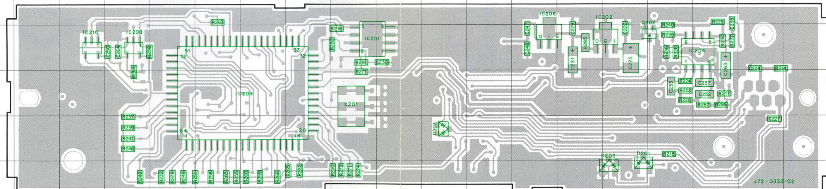
TX-RX UNIT (X57-4590-XX) (B/2) Foil side view -10 : TK-940 -11 : TK-941
