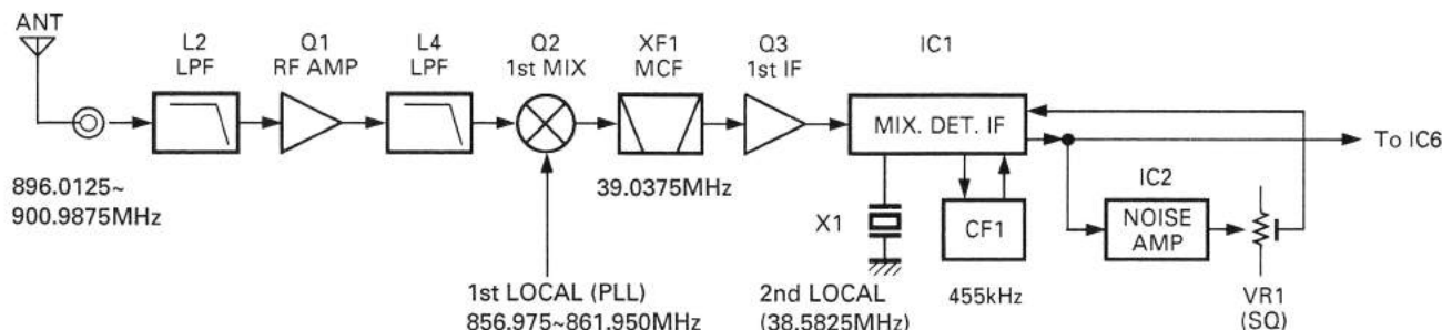
Fig. 1 Receiver system
