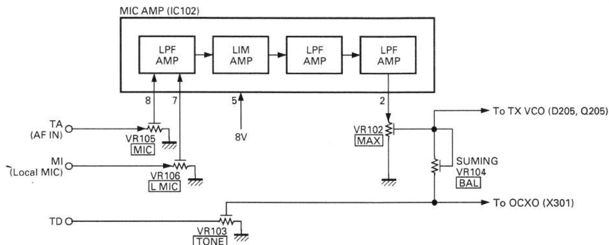
Fig. 5 Microphone amplifier
