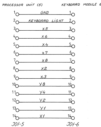
CABLE 4: PROCESSOR TO KEYBOARD
