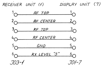
CABLE 6: RECEIVER TO DISPLAY
