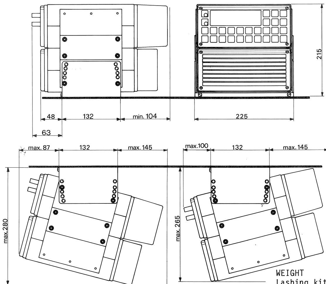
MOUNTING KIT H2068 AND H2055
