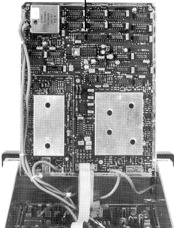
RF Shields
