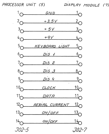
CABLE 3: PROCESSOR TO DISPLAY
