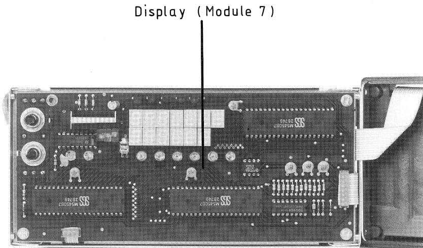
Front Chassis removed.
