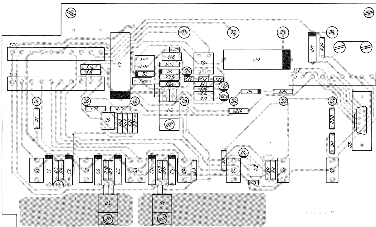
COMPONENT LOCATION TESTBOX
