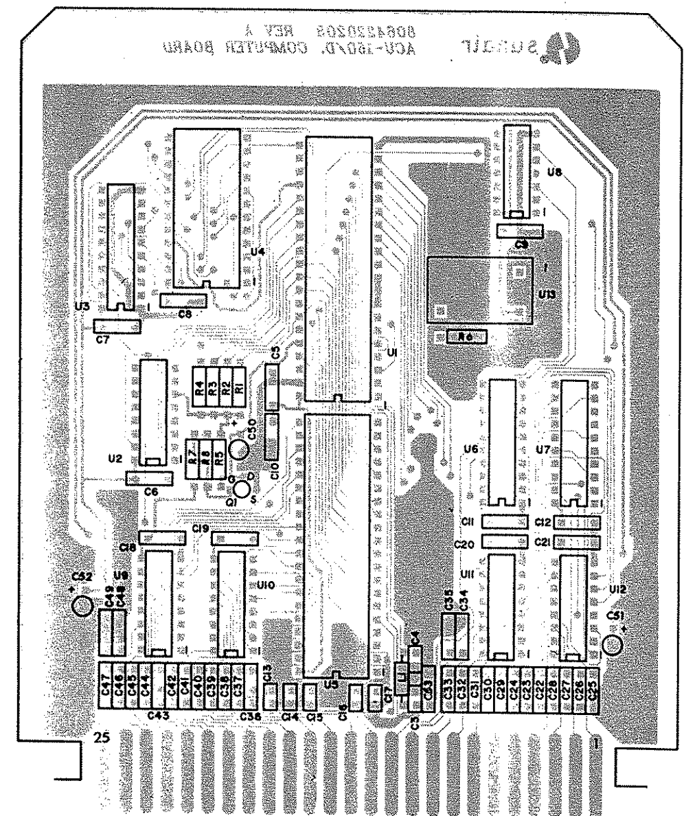
CIRCUIT SIDE
