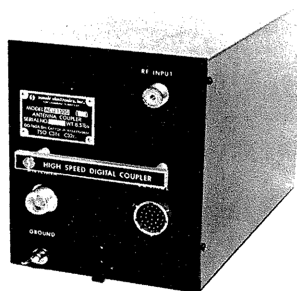
ACU-150D DIGITAL AUTOMATIC ANTENNA COUPLER
