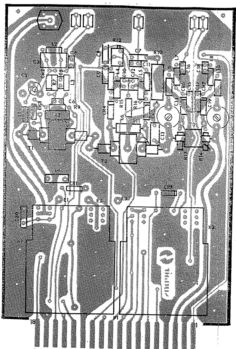
CIRCUIT SIDE
