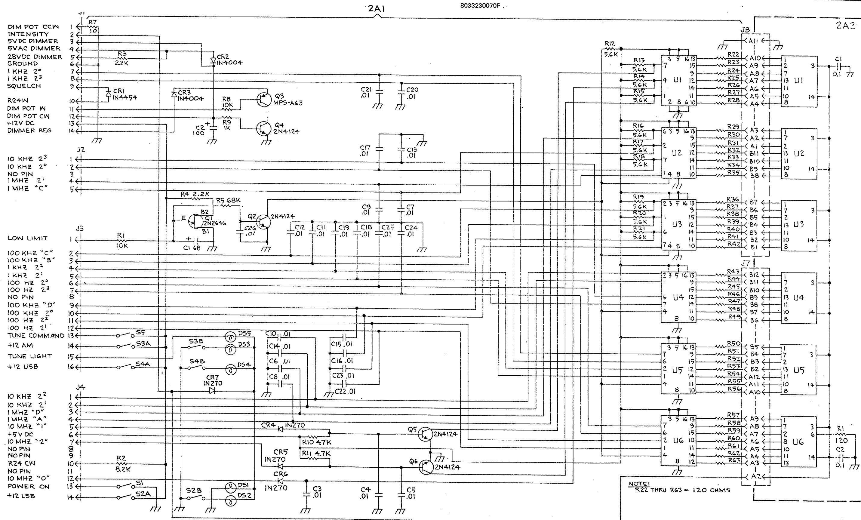
Figure 5.26 Decoder (2A1) and Display (2A2) Boards
