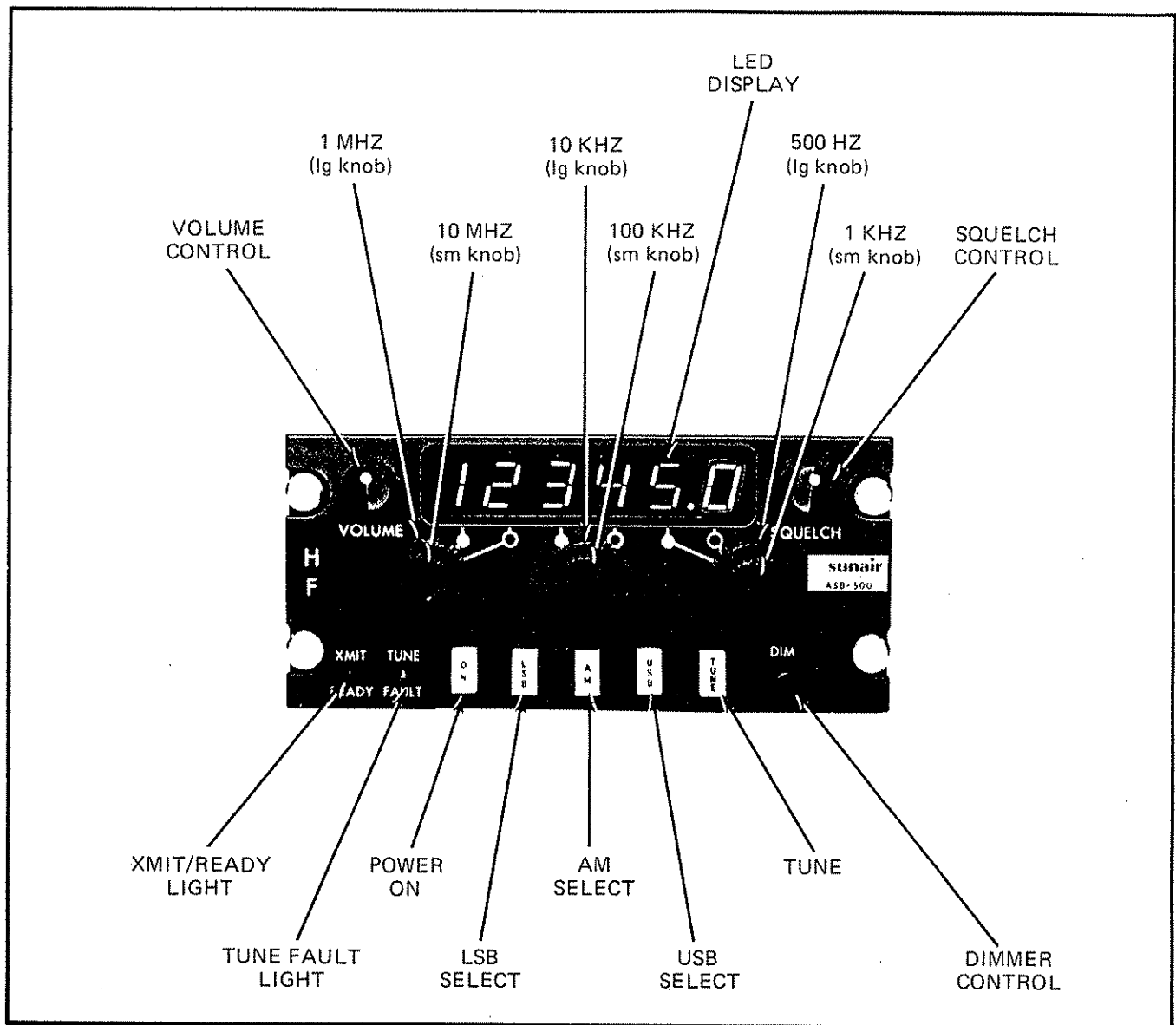
Figure 3.1 Remote Control Head Front Panel
