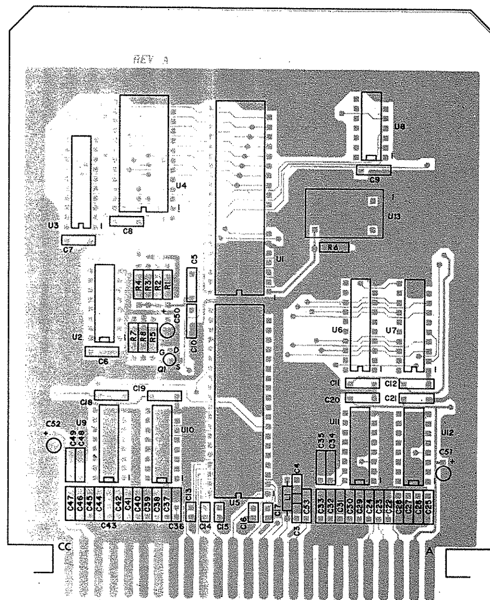
COMPONENT SIDE
