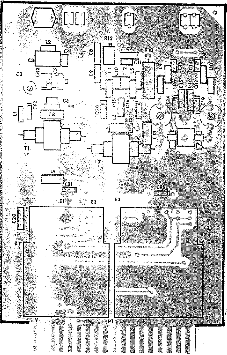
COMPONENT SIDE
