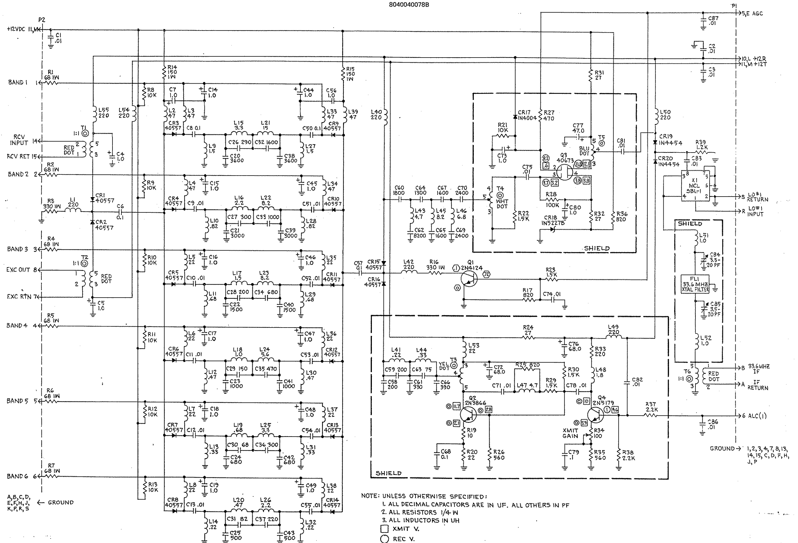
Figure 5.13 First Mixer Board (1A5)
