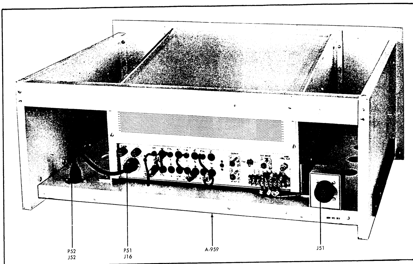
Figure 3-7. Rear View, Model XFK in Panel-Chassis Assembly
