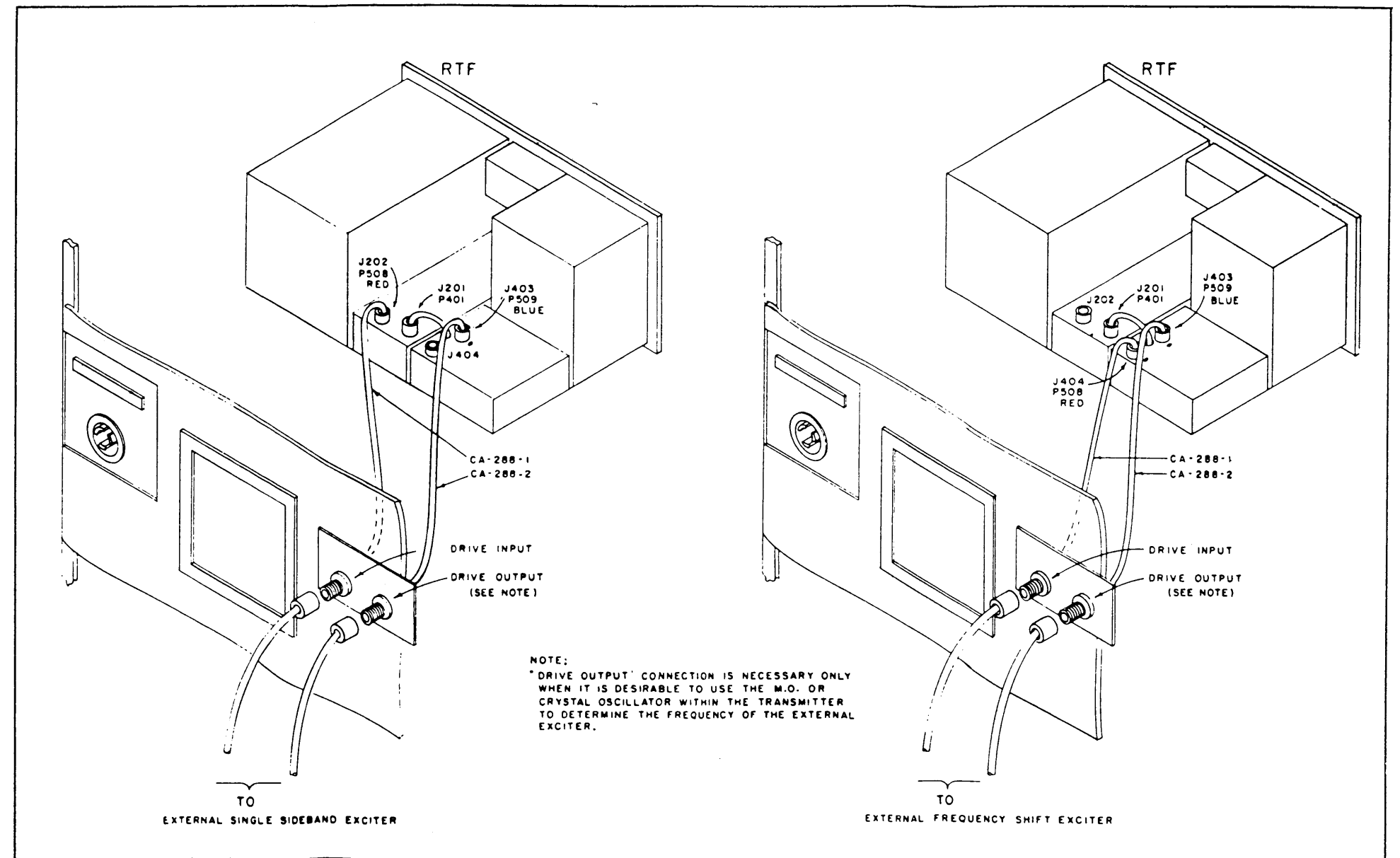
Figure 3-8A. Cabling Diagram.
