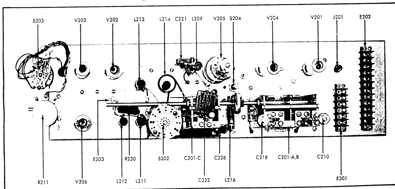
Figure 4 4. Top View, Multiplier Sub-chassis
