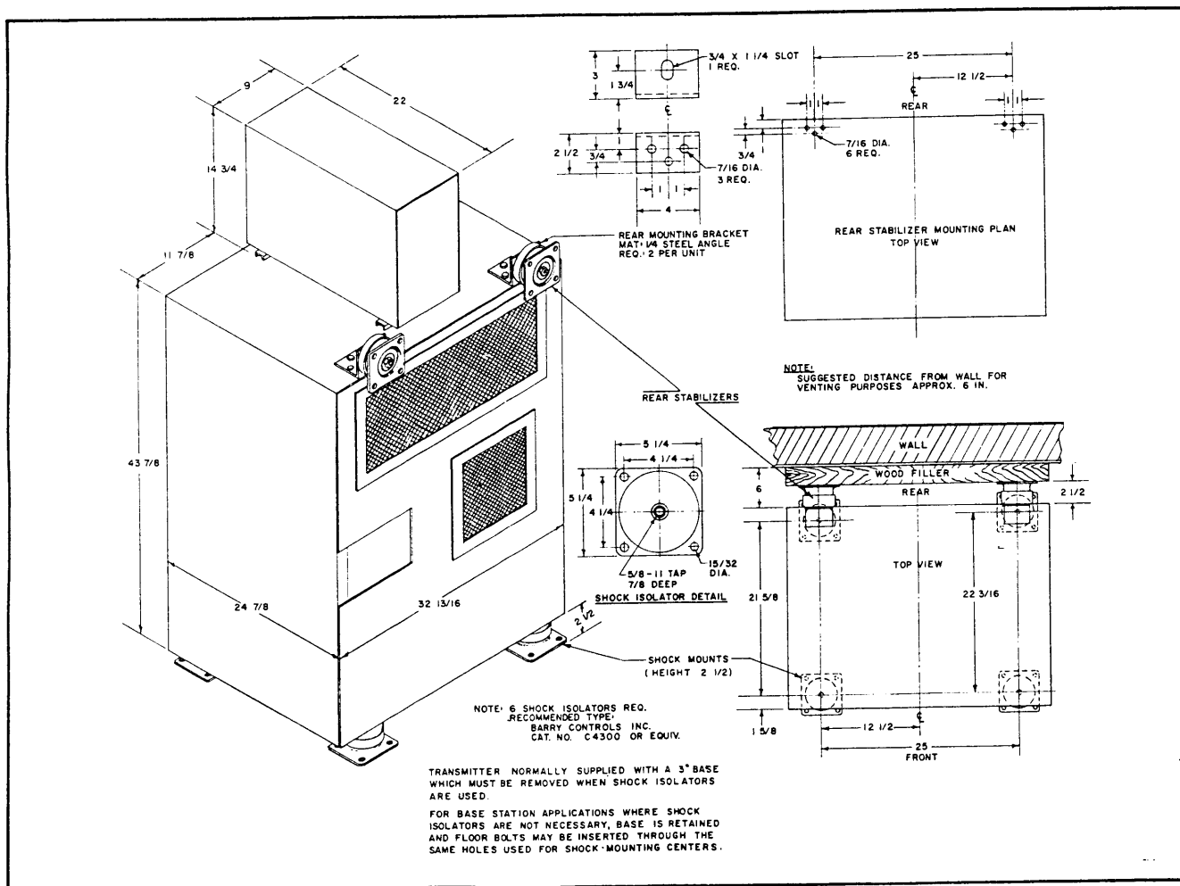
Figure 3-1. Mounting Dimensions
