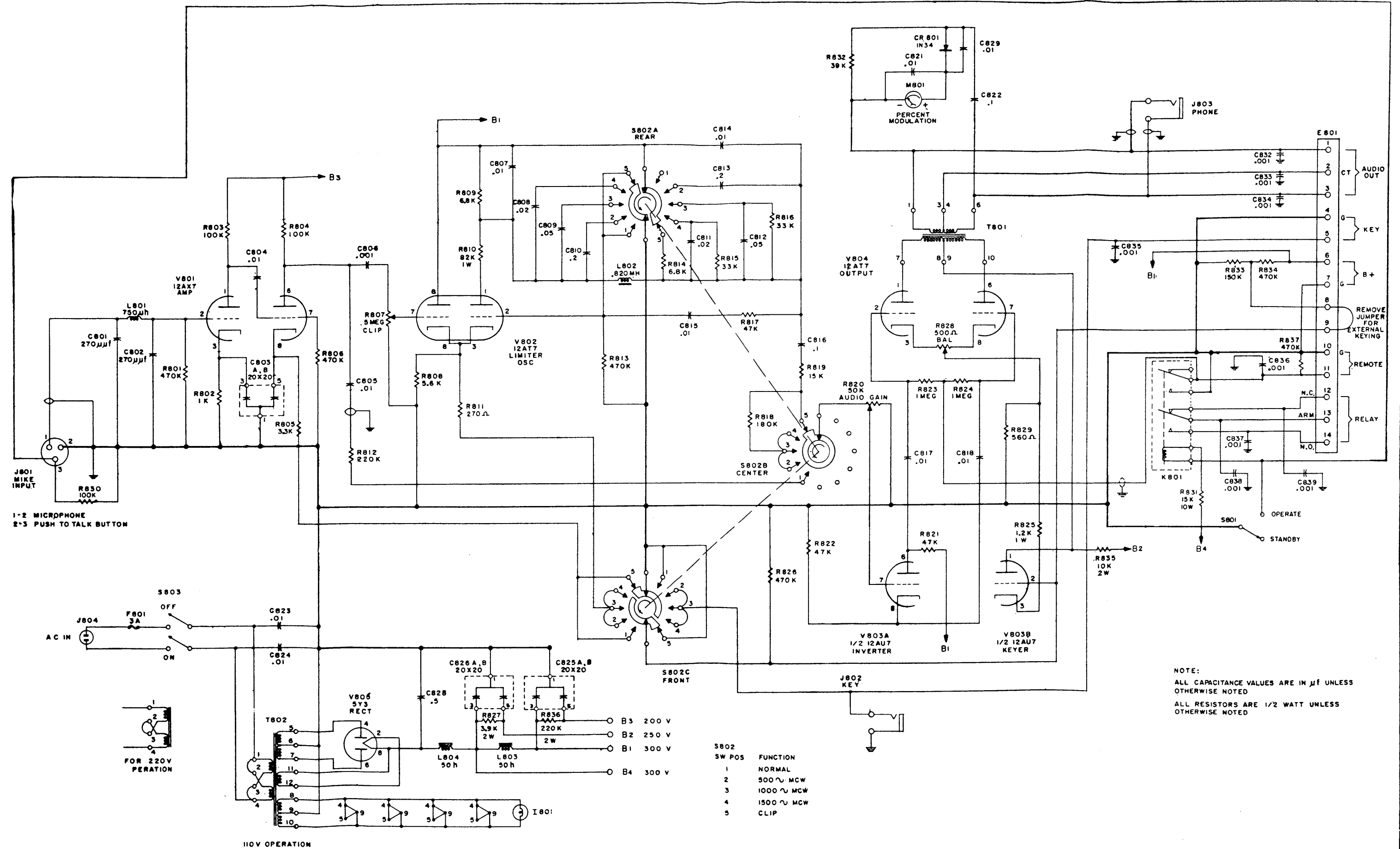
Figure 5-3 Schematic Diagram, Model RTC.
