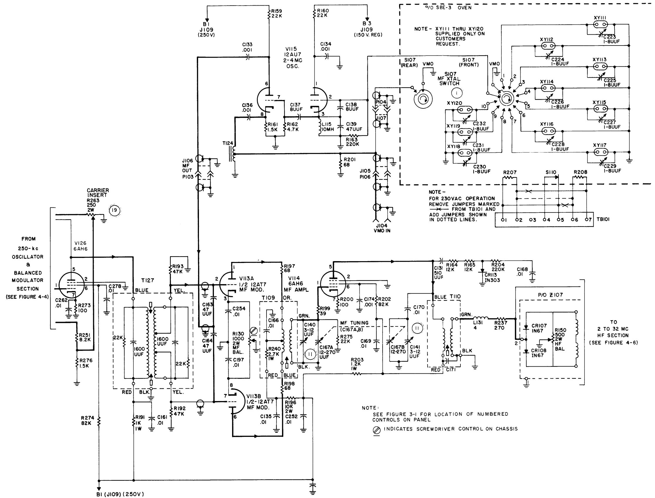
Figure 4-5. Schematic Diagram, 2- to 4-mc MF Section
