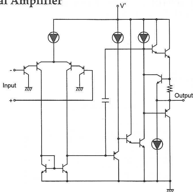
CIRCUIT DIAGRAM
