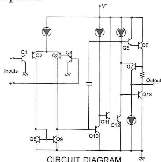
CIRCUIT DIAGRAM
