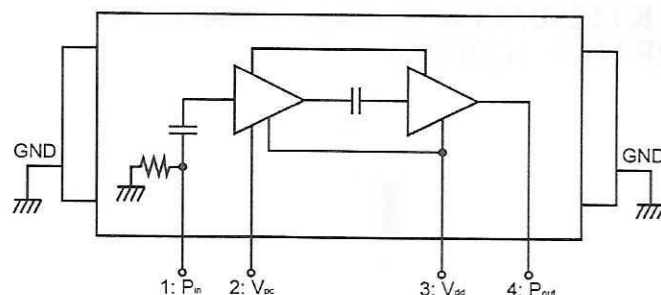
CIRCUIT DIAGRAM
