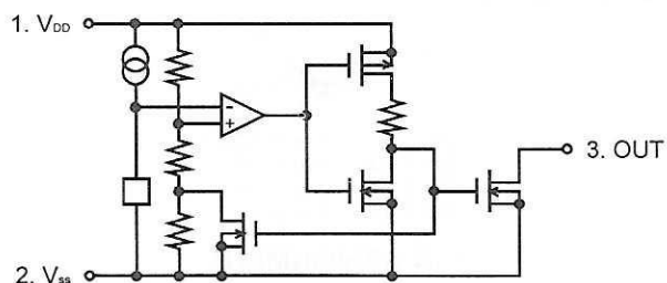
CIRCUIT DIAGRAM
