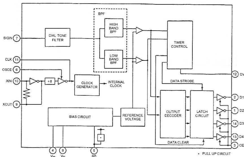
BLOCK DIAGRAM
