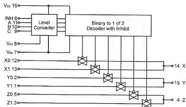
BLOCK DIAGRAM
