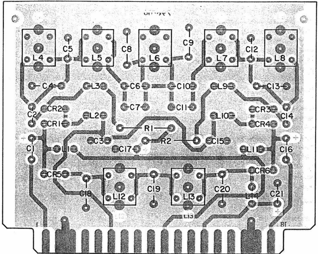
Figure 1-4. Type 796016 Input Filter (A1A1), Location of Components
