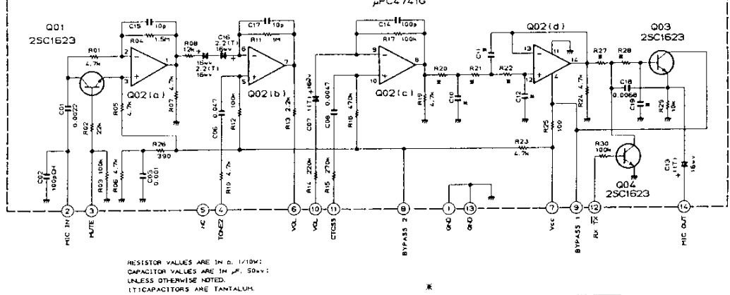
MIC AMP UNIT F2973101A (No. 8xx)
