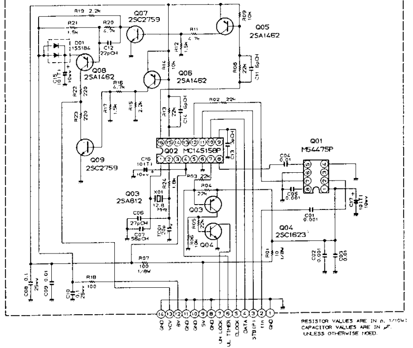
PLL UNIT F2973104A (No. 4xx)
