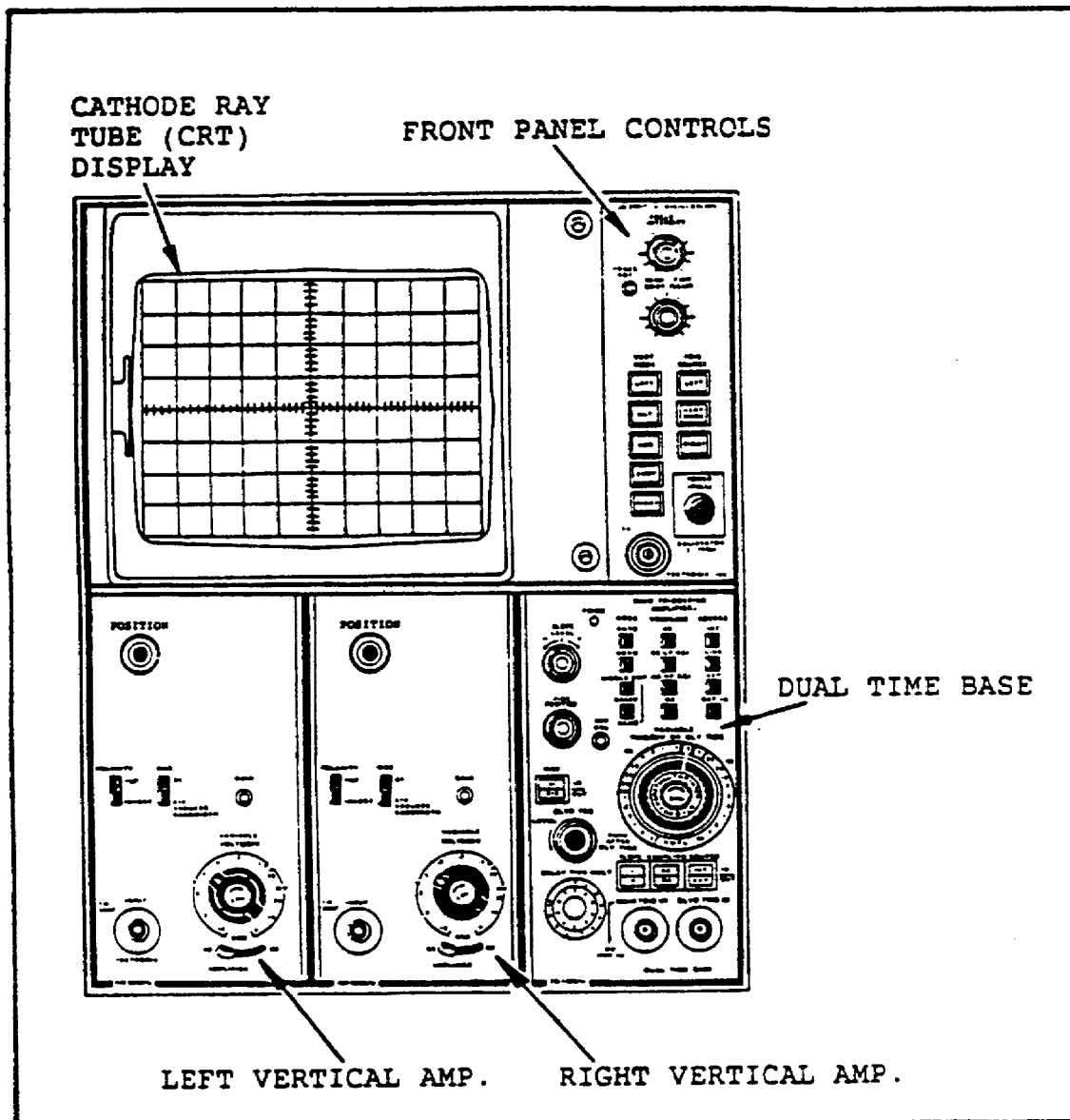
FIGURE 1. OSCILLOSCOPE SUBASSEMBLIES.
