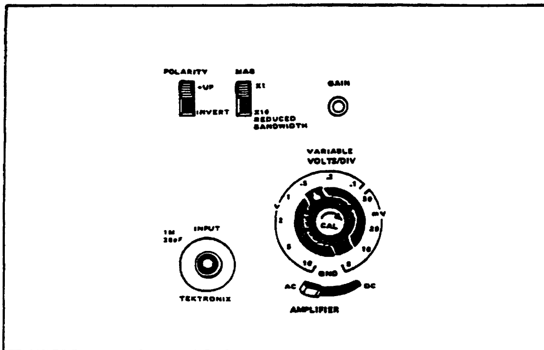
FIGURE 8. VOLTS/DIV SWITCH.
