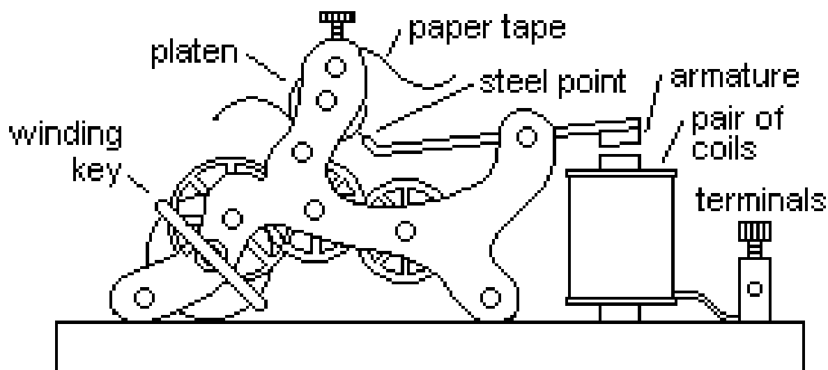
Morse Register
