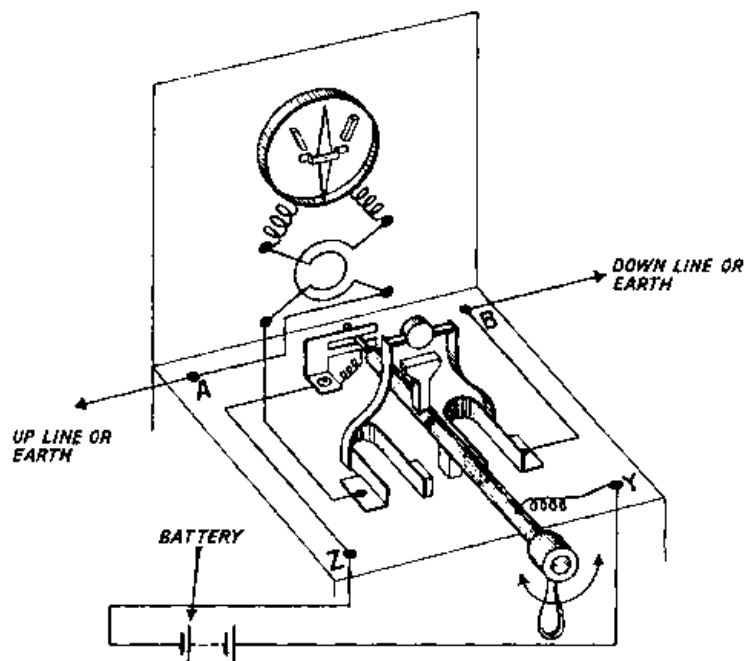
Single-needle Instrument.
