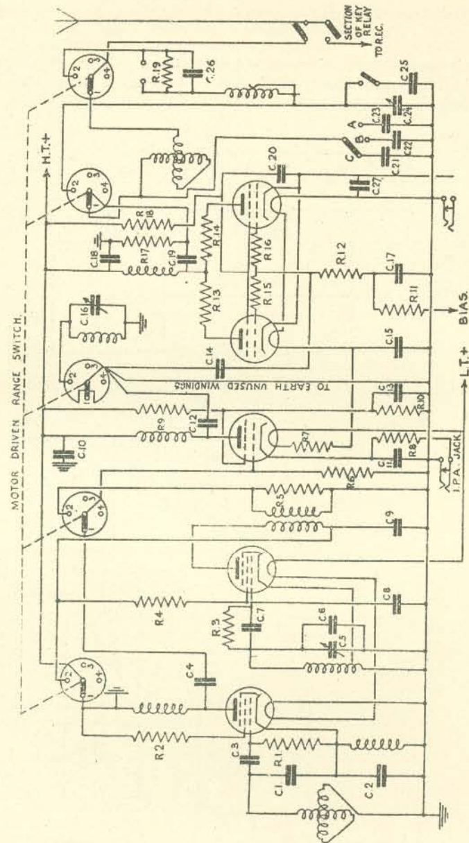
FIG. 93.—Circuit diagram transmitter, T.A. 12B.
