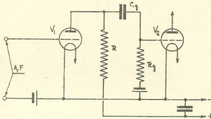
FIG. 41.—Resistance-capacity coupling.
