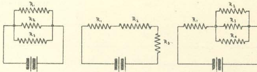
FIG. 1.—Resistance arrangements.
