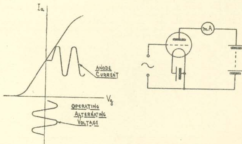
FIG. 17D —Triode characteristics (b).
