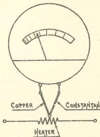
FIG. 3.—Thermo-junction ammeter.
