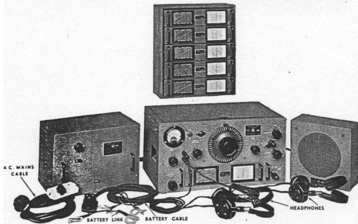
PLATE 1 — INSTALLATION.
