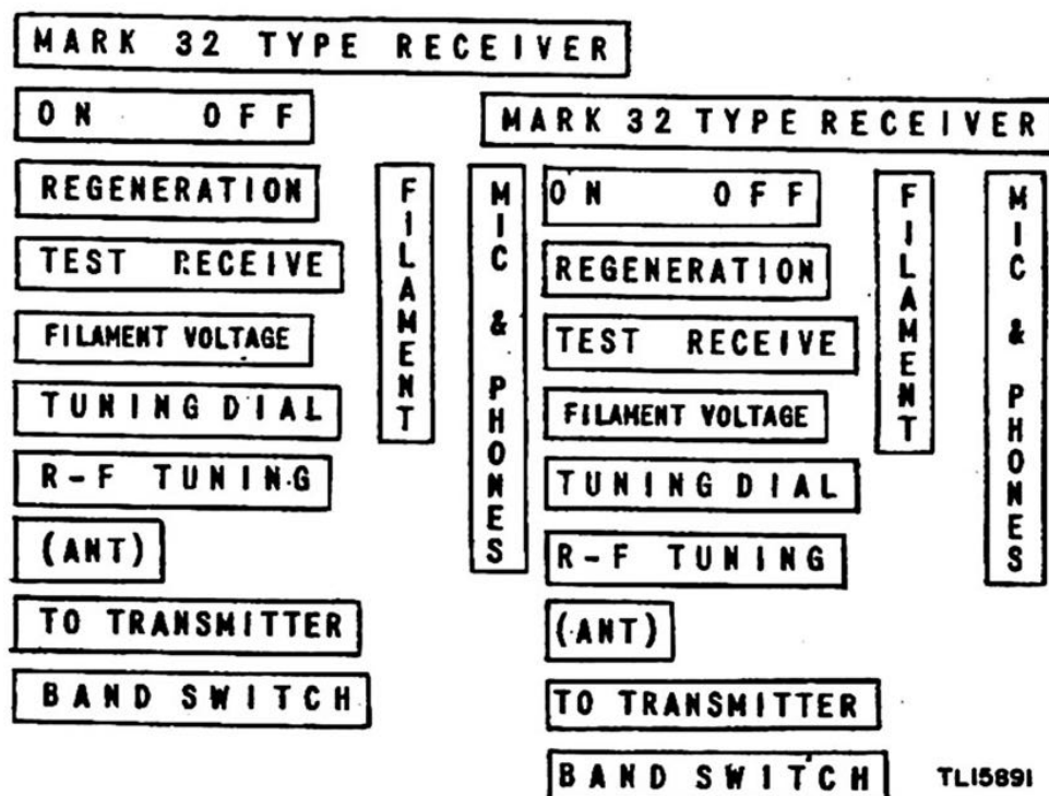
Figure 33. Name tabs for installation and operation of Mark 32 Type Receiver. (These may be cut out and placed on the receiver.)
