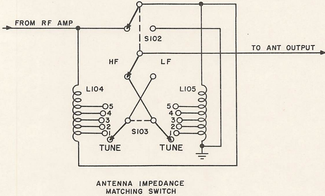
FIG. 18.1 ANTENNA IMPEDANCE MATCHING SWITCH FOR TRANSMITTER RT-6 SERIAL NOS. 2001 TO 2614.
