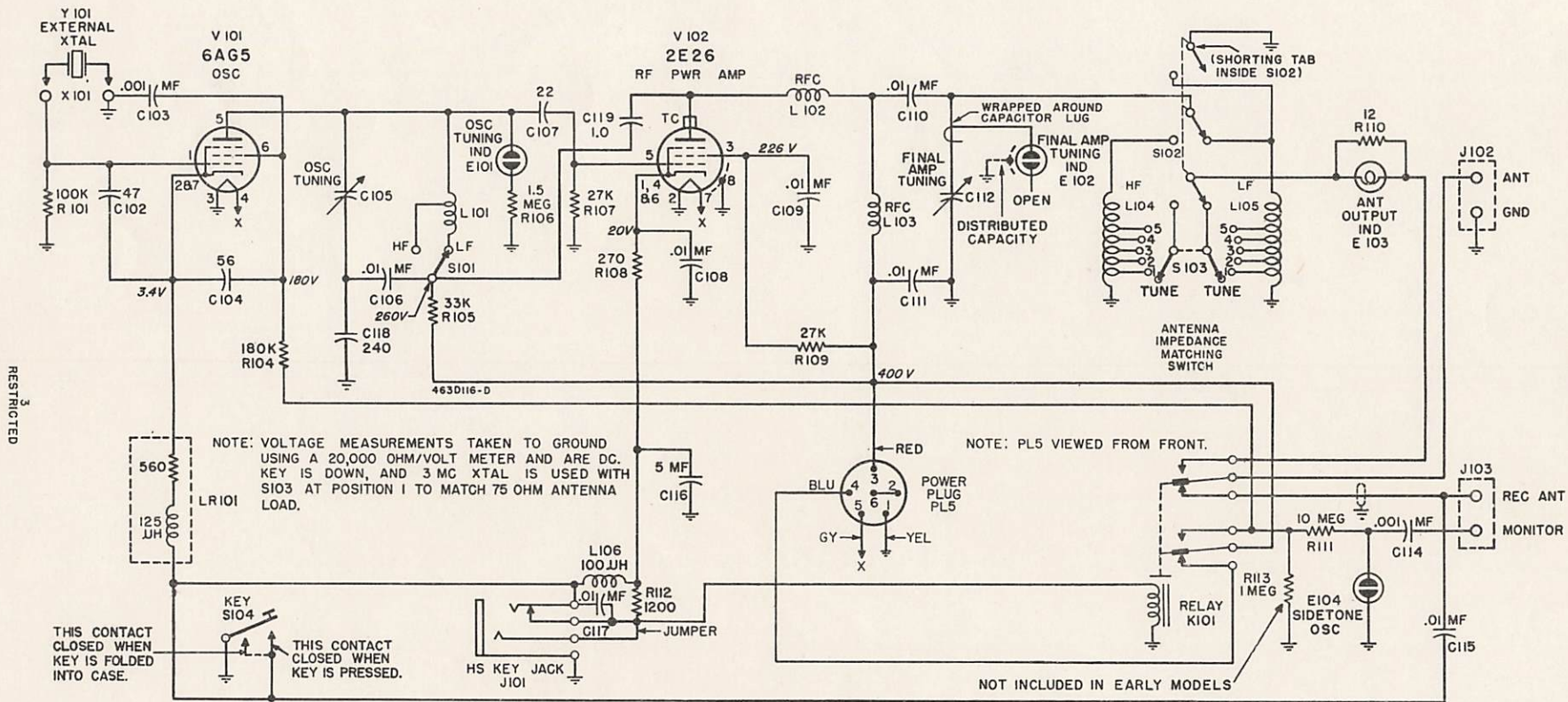
FIGURE 18. TRANSMITTER RT-6 SCHEMATIC DIAGRAM
