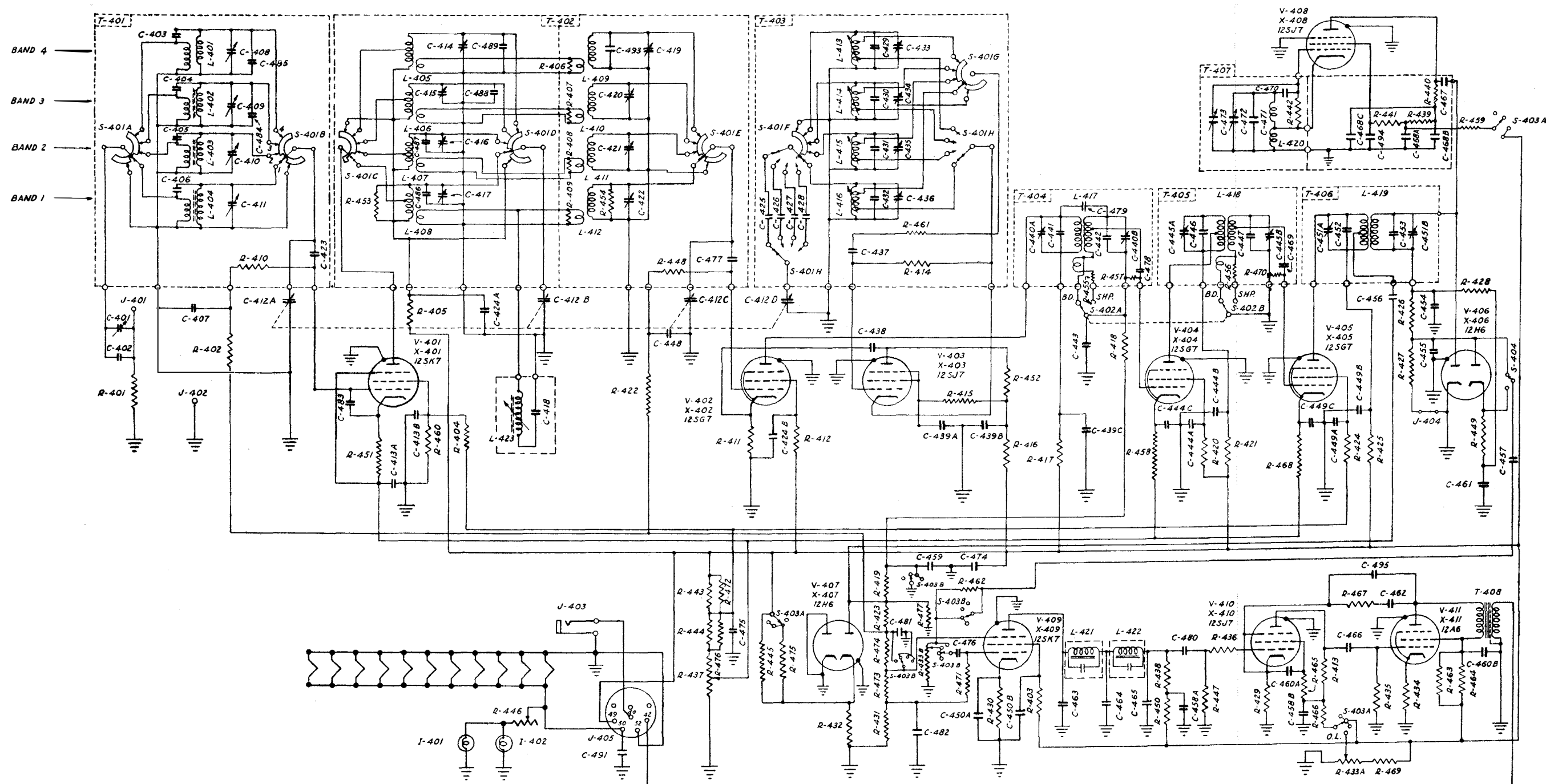
FIG. 62 MEDIUM FREQUENCY RECEIVER, TYPE CAY-46076-A, SCHEMATIC DIAGRAM (DWG. T-7611588).
