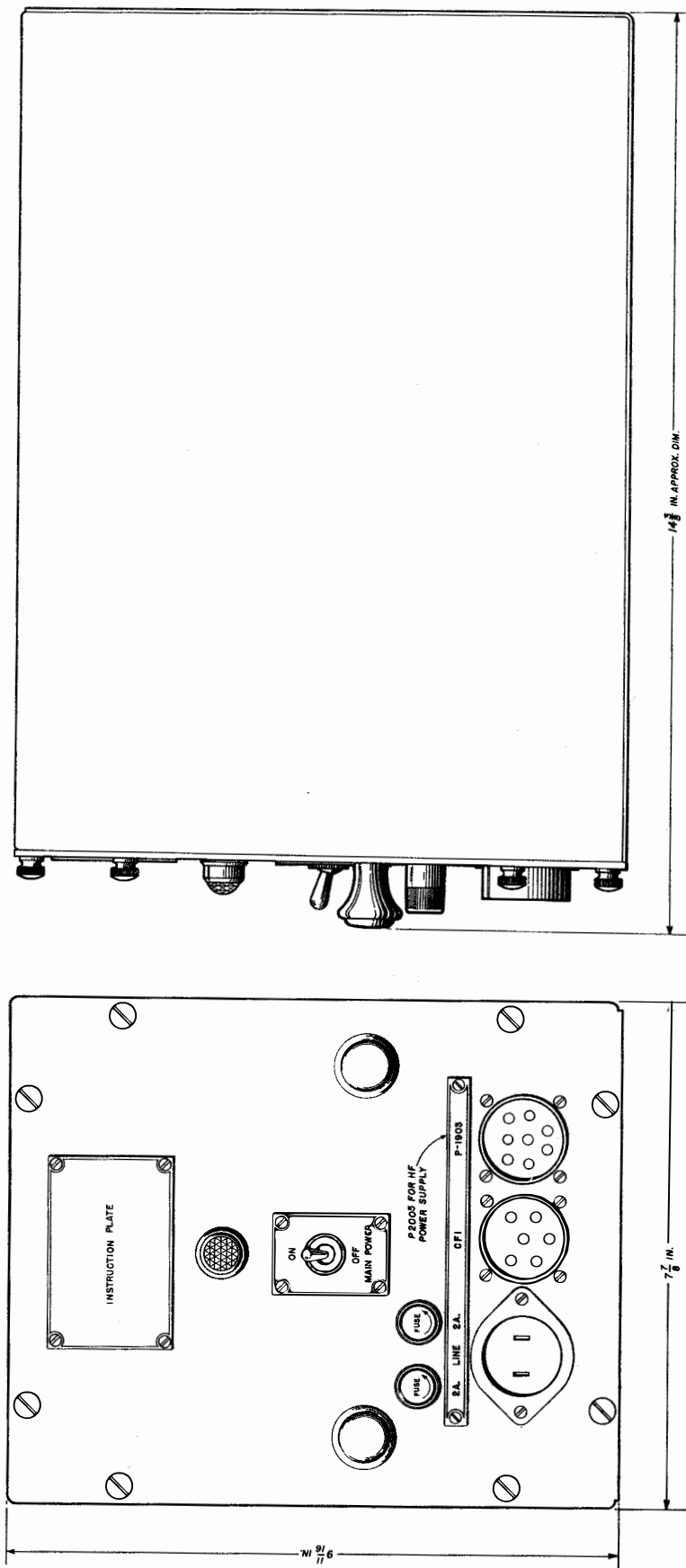
FIG. 54 RECTIFIER POWER UNIT, TYPE CAY-20086, FOR 115 VOLT, 60 CYCLE, A.C. OPERATION, OUTLINE AND DIMENSIONS (DWG. T-7613096).
