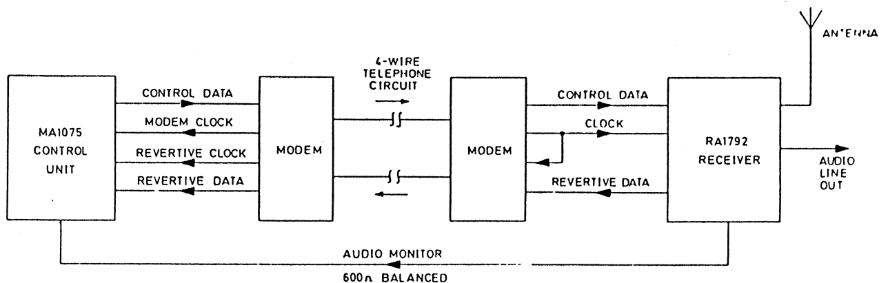
Fig. 1(b) Remote Control System
