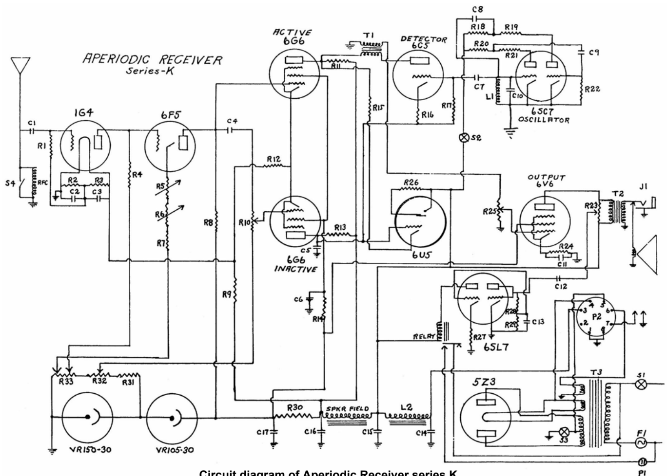
Circuit diagram of Aperiodic Receiver series K.
