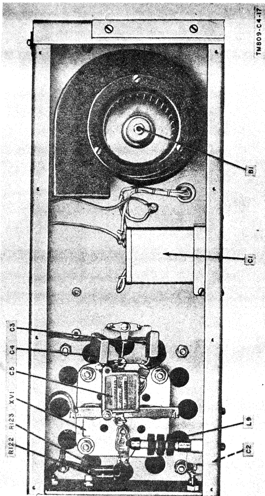
Figure 47. RF deck, blower duct (cover removed), A model transmitters.
