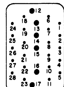
PIN LAYOUT OF JACKS J6, J7 & PLUG P2
