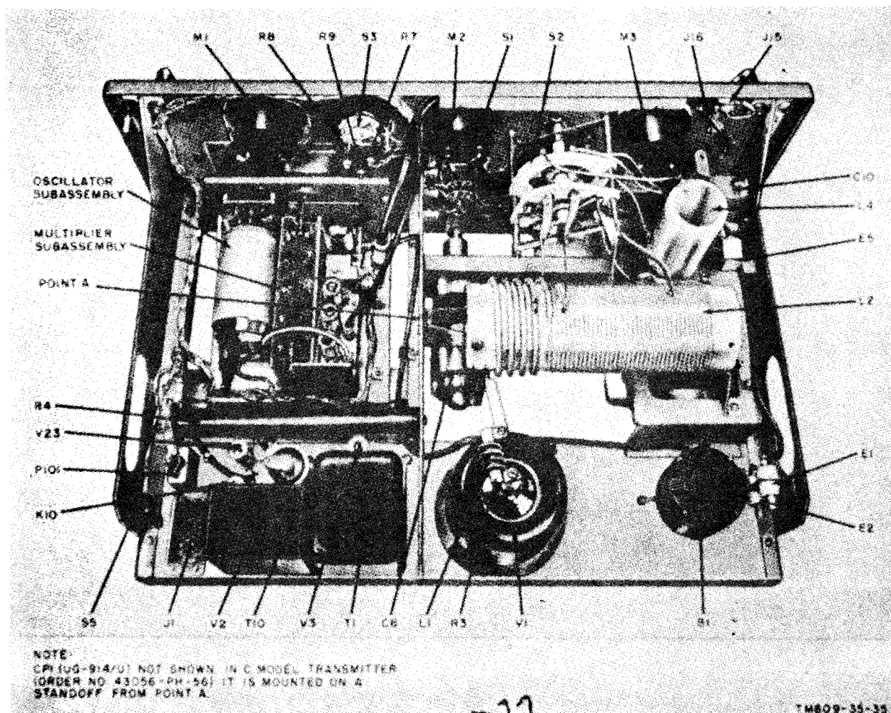
Figure 40. RF deck of B model transmitters and C model transmitters procured on Order No. 43056-Phila-56, top view.
