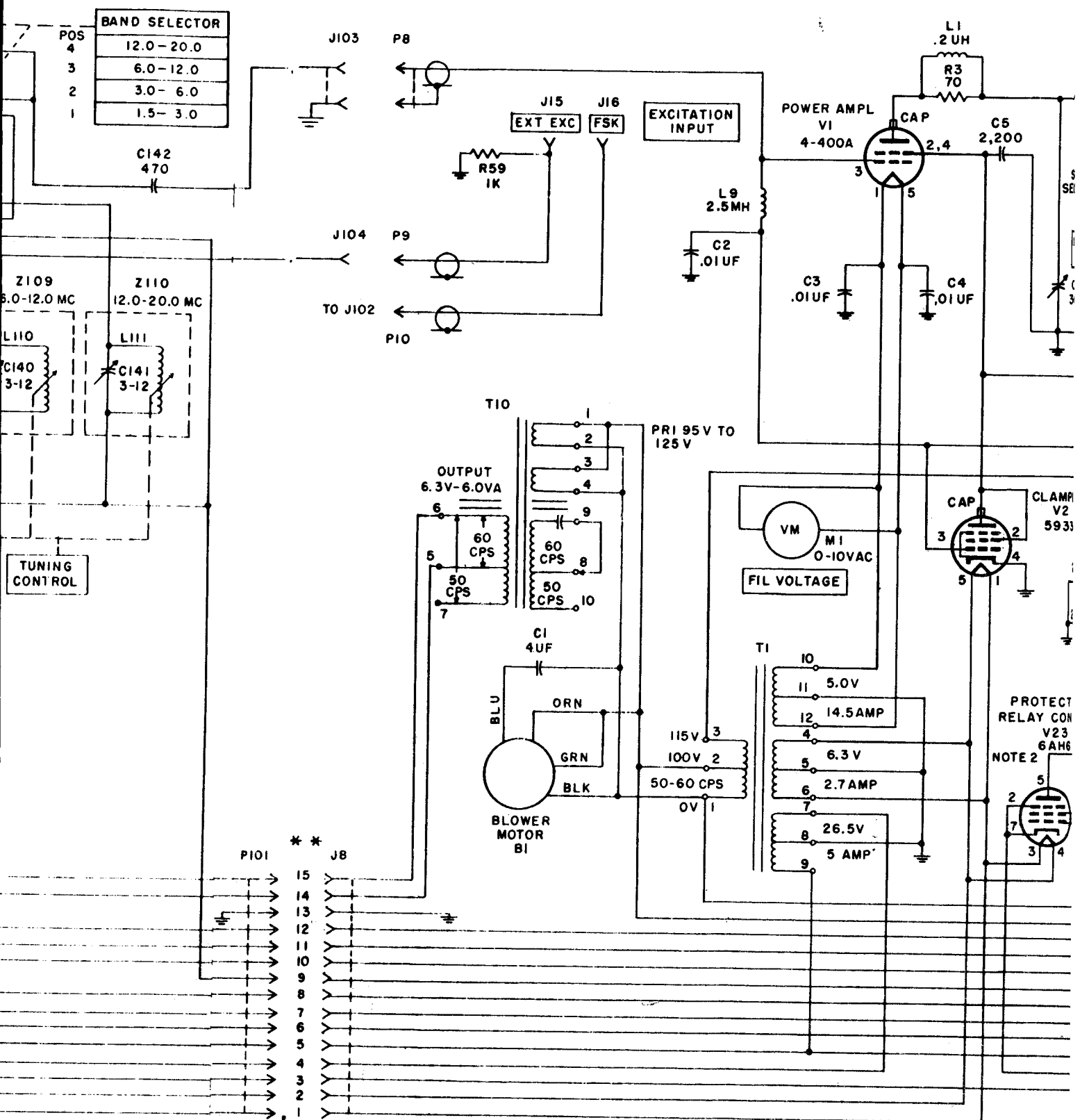
Model transmitters, schematic diagram of RF deck
