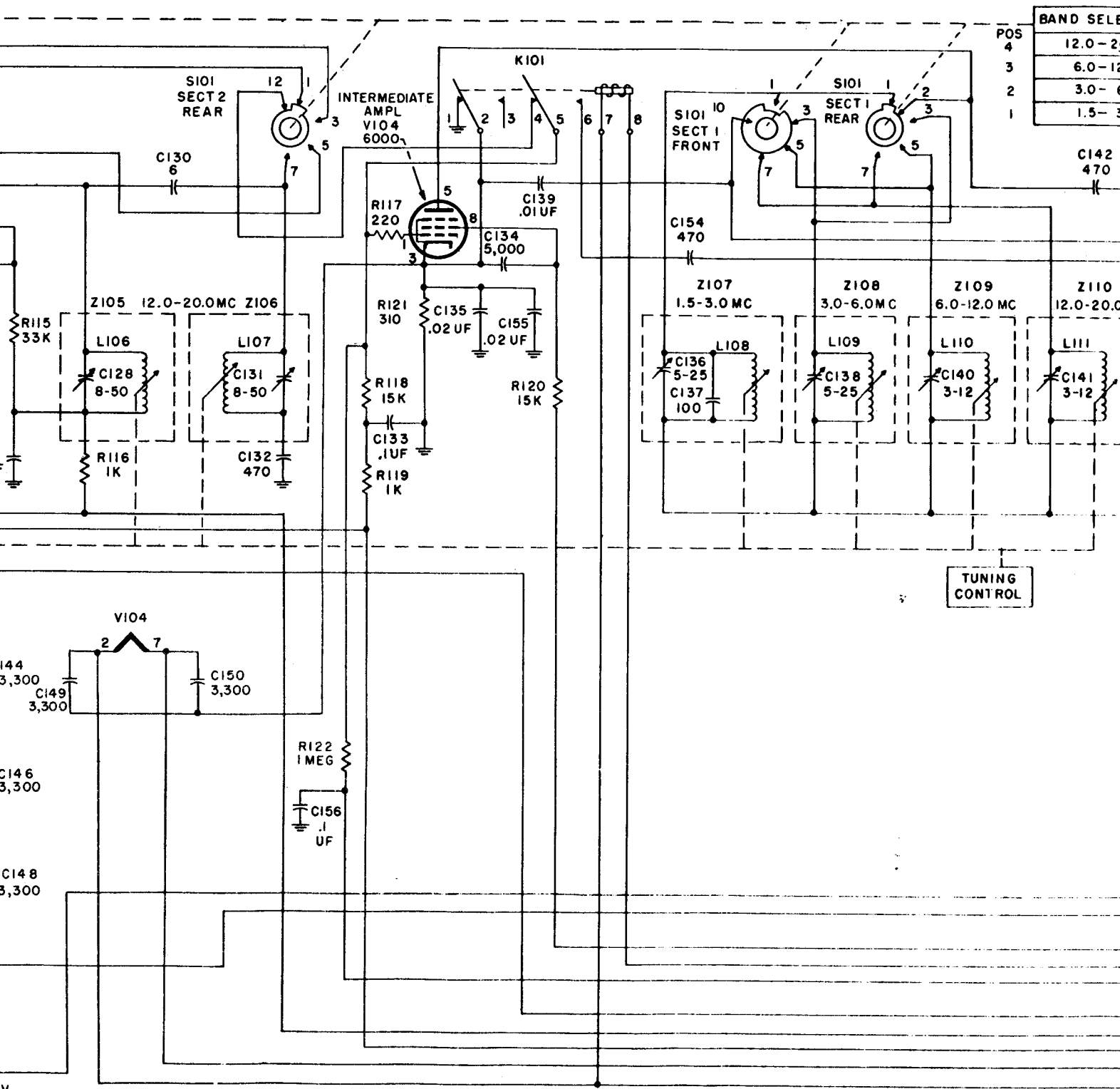
Figure 100. B and C model transmitters, schematic
