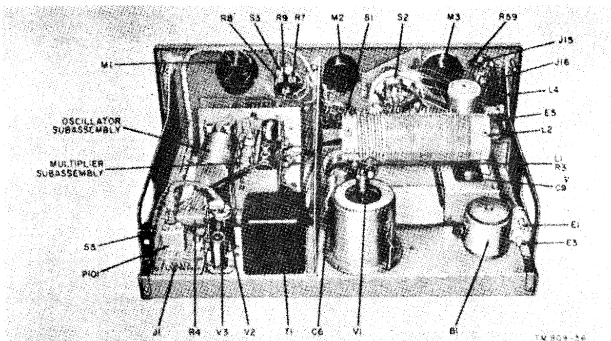
Figure 39. RF deck of basic model transmitter, top view.
