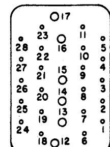
PIN LAYOUT OF PLUGS P1, P6, P7 & JACK J2
