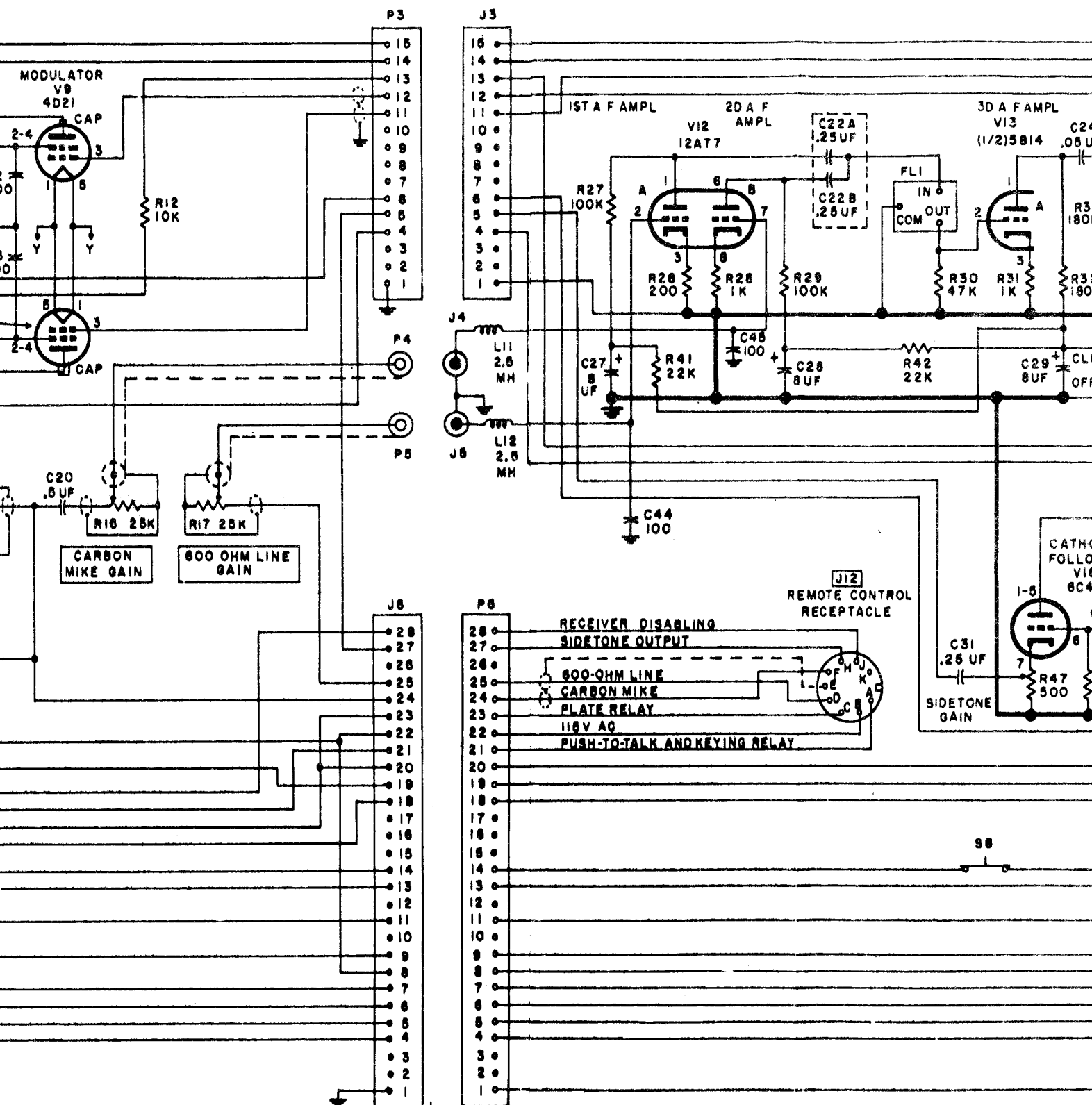
Figure 98. Basic model transmitter, schematic diagram of modulator deck, power deck, and housing
