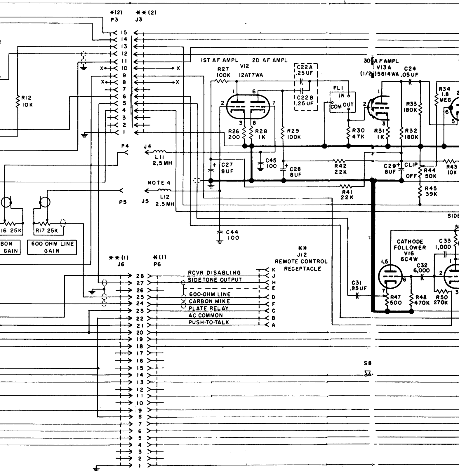
Figure 101. B and C model transmitters, schematic diagram of modulator section
