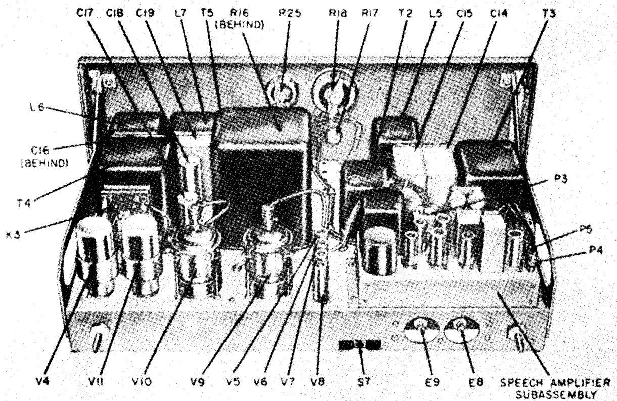
Figure 60. Modulator deck top view, basic model transmitters.
