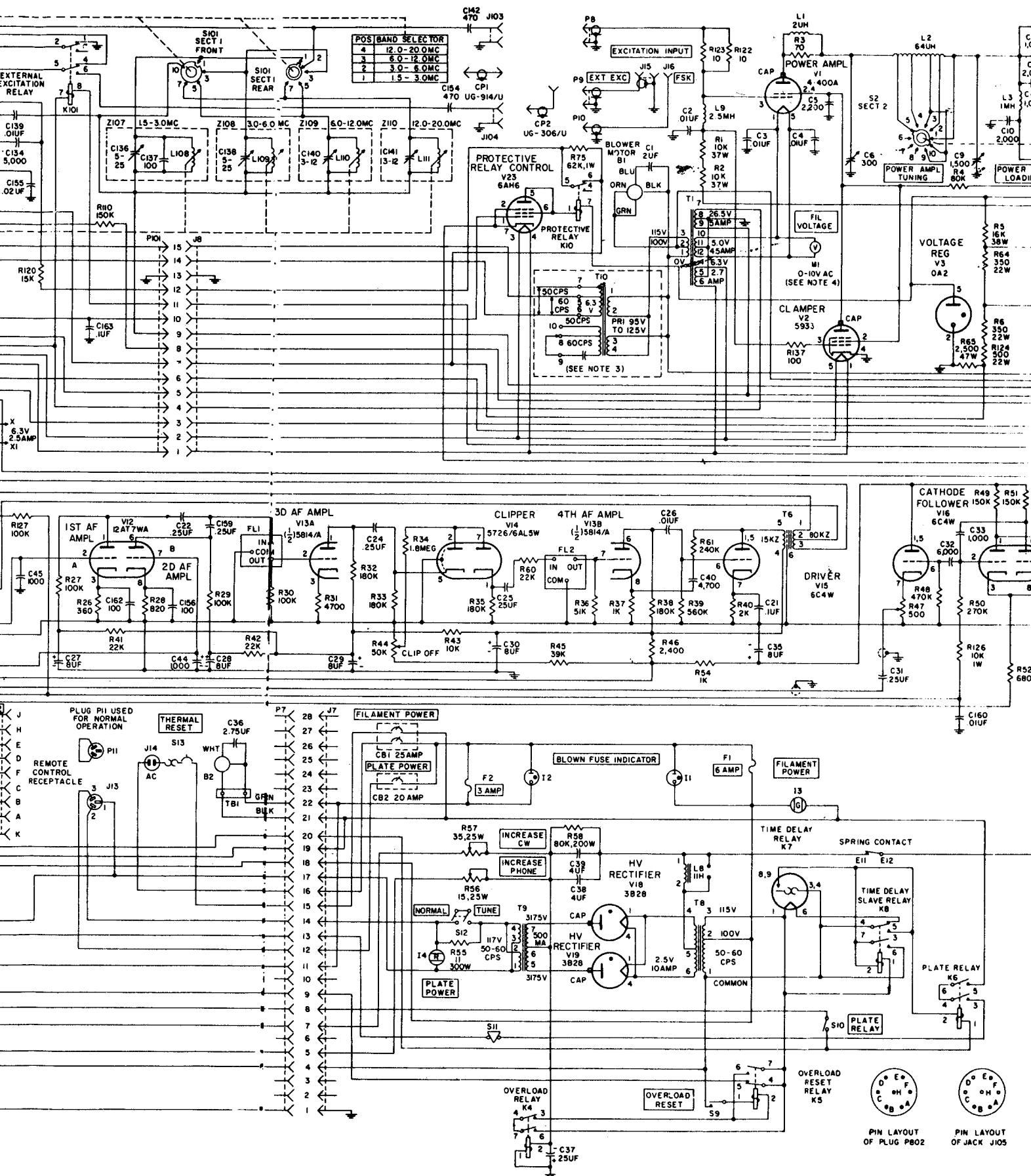
99. A model transmitter, complete schematic diagram.
