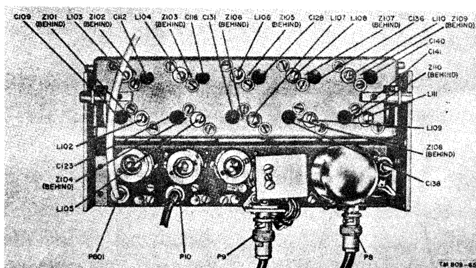
Figure 49. Multiplier subassembly, top view.
