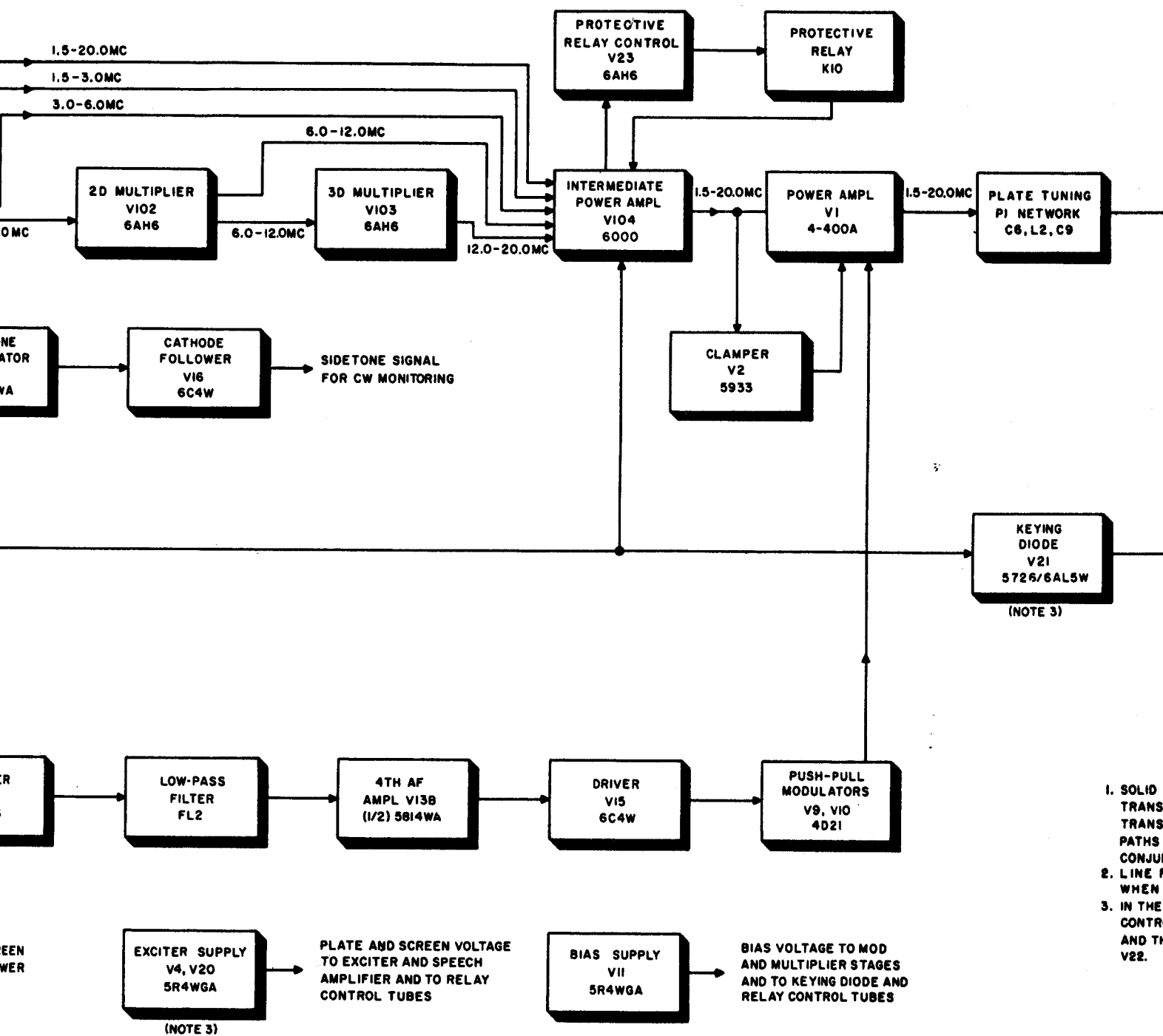
Figure 2. Lettered model transmitters, block diagram.
