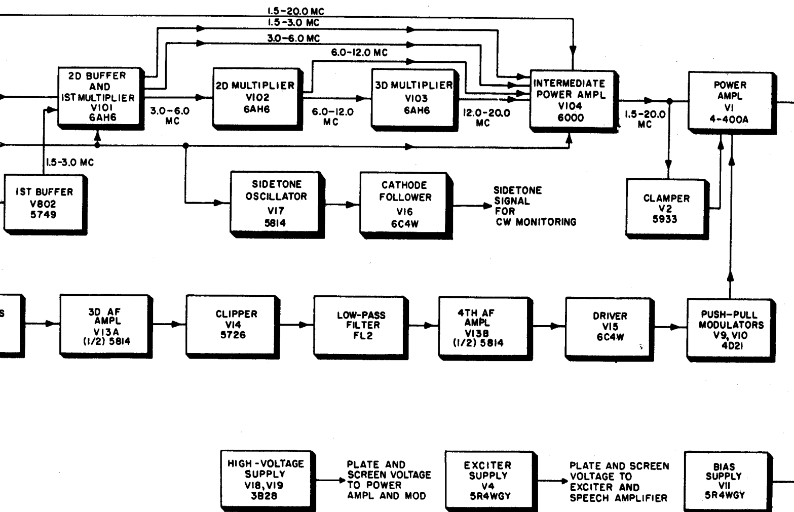
Figure 1. Basic model transmitter, block diagram.
