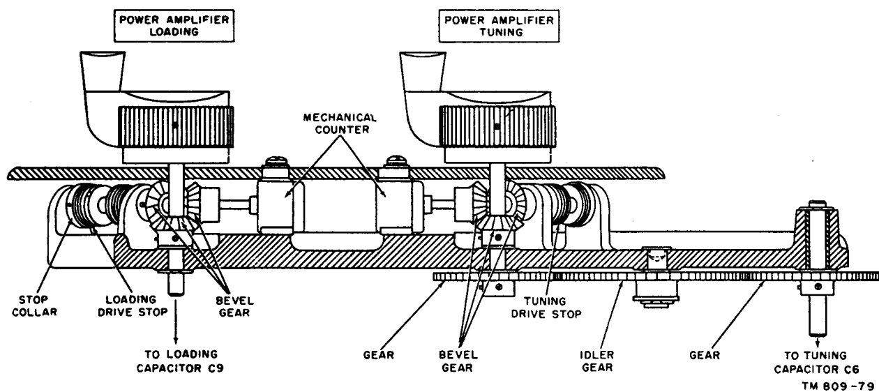
Figure 93. Power amplifier tuning drive, gear assembly.
