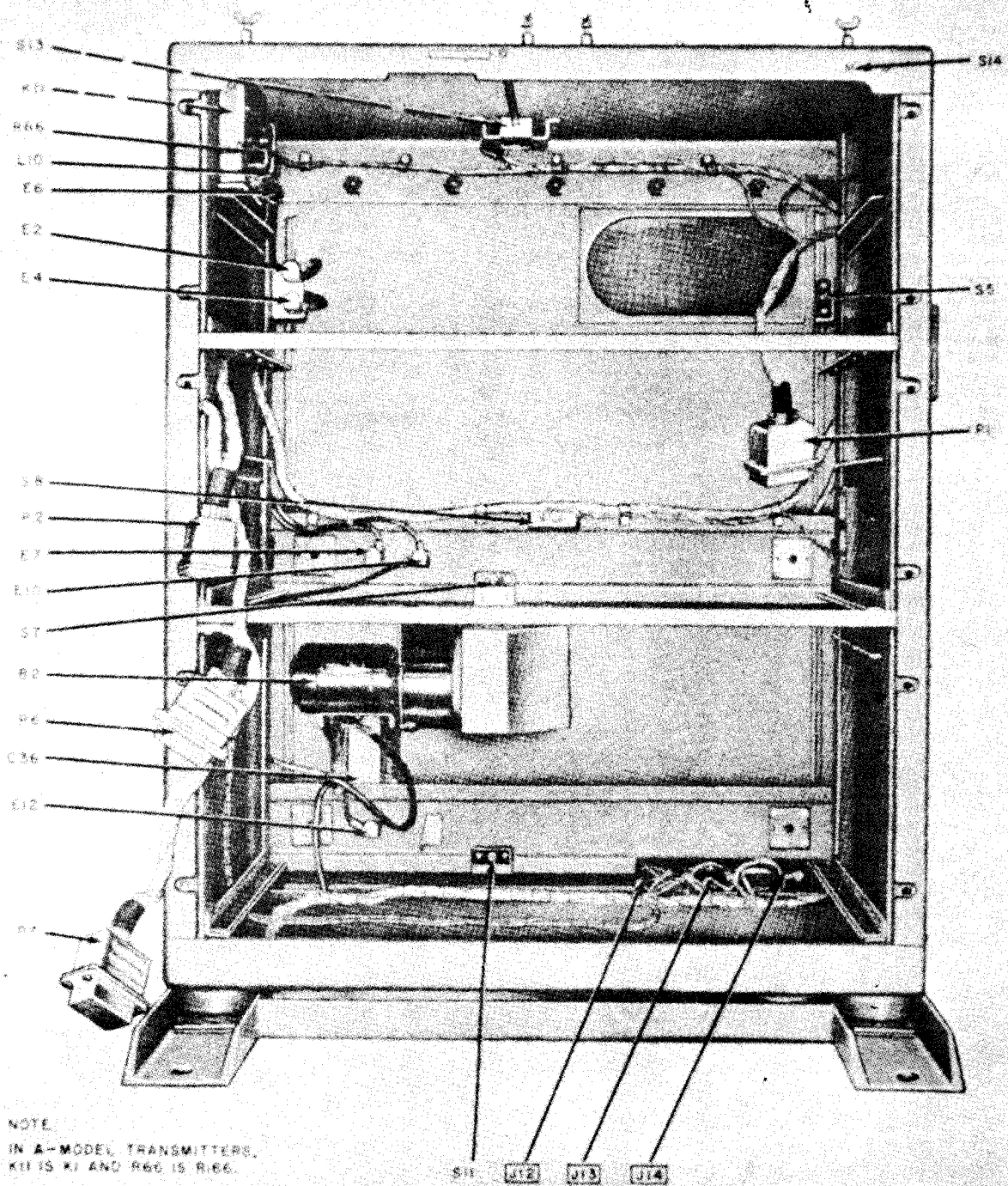
Figure 88. Transmitter housing, decks removed, lettered model transmitters.
