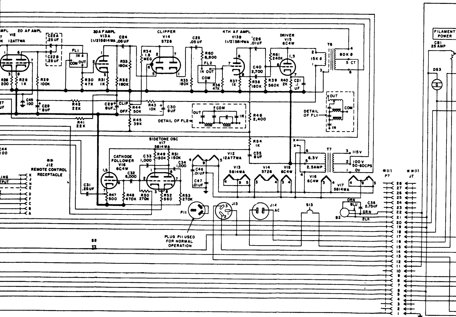
108. (Added) E model transmitters, modulator deck, power deck, and housing, schematic diagram.
