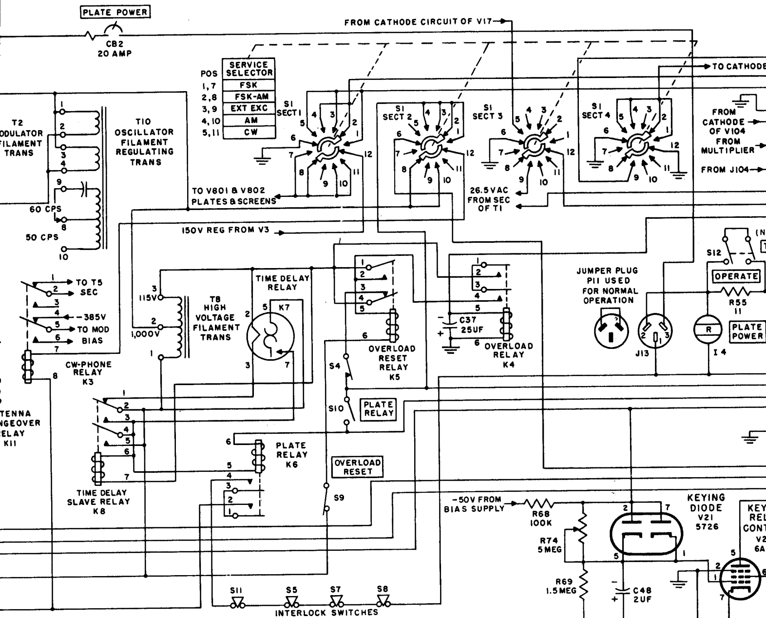
Figure 30. Primary power distribution and control circuits, B and C model transmitters.
