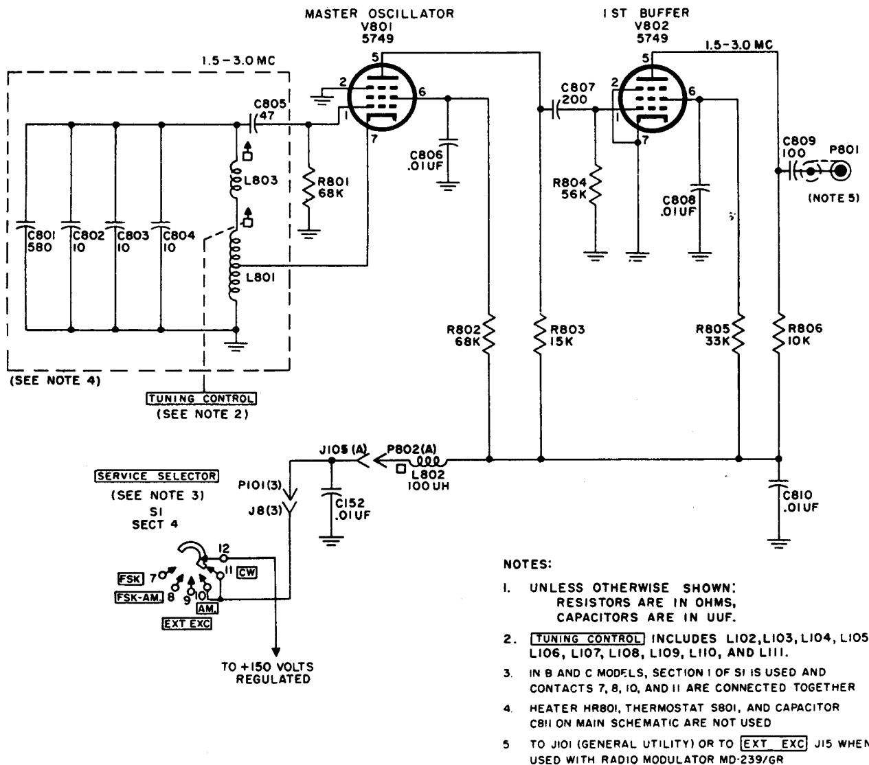
Figure 3. Master oscillator and first buffer stages.
