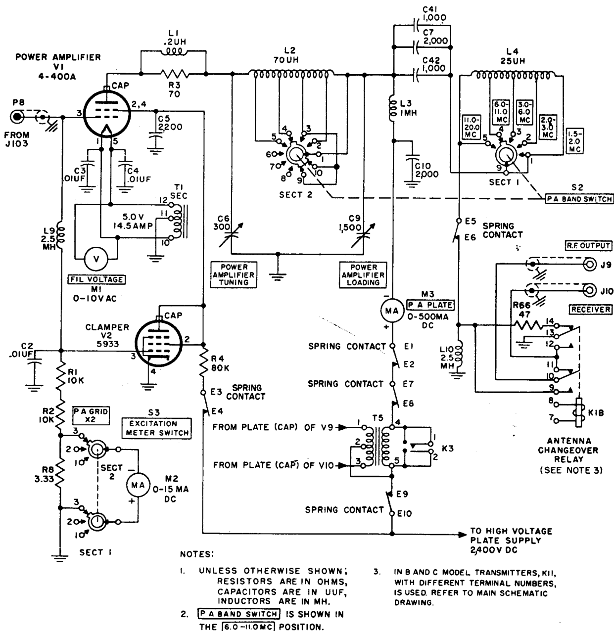
Figure 9. Power amplifier and clamper stages, basic, B, and C models.
