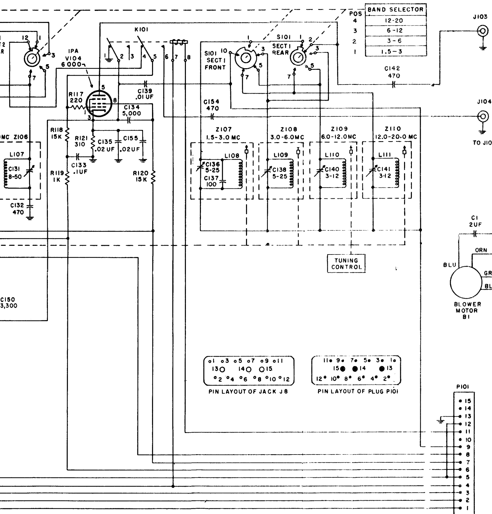
Figure 97. Basic model transmitter, schematic diagram of RF deck.
