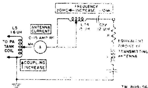
Figure 35. Antenna tuning unit with range switch in 10-20 MC position.
