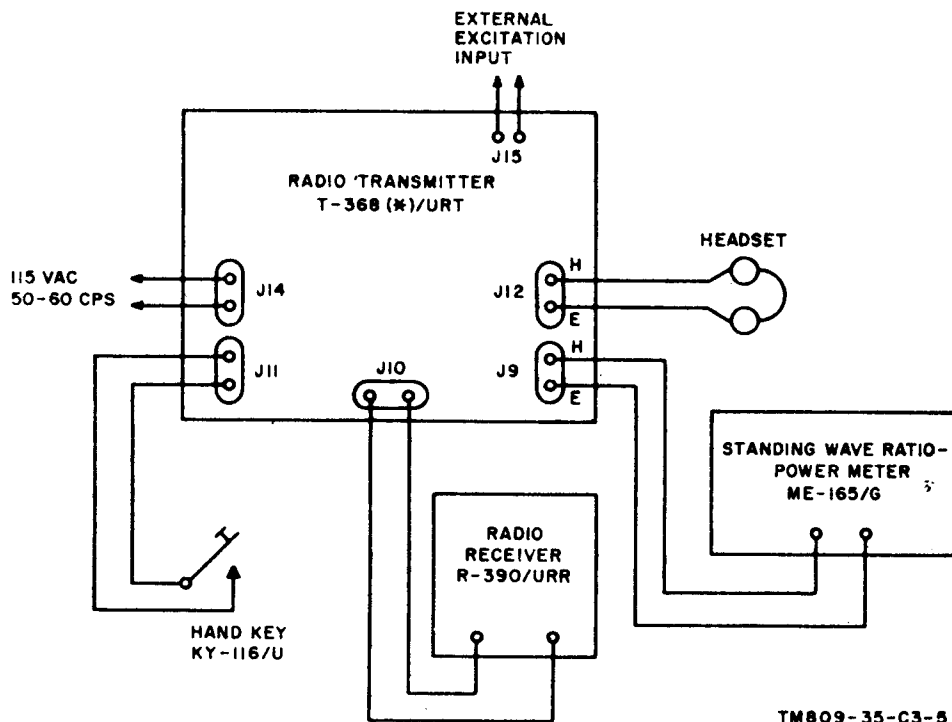
Figure 108. FSK operational and band edge tuning test setup.
