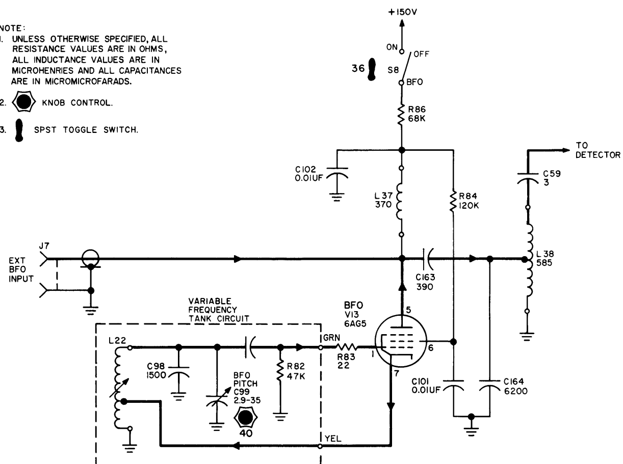
Figure 4-8. Schematic Diagram, GPR-90RXD, BFO
