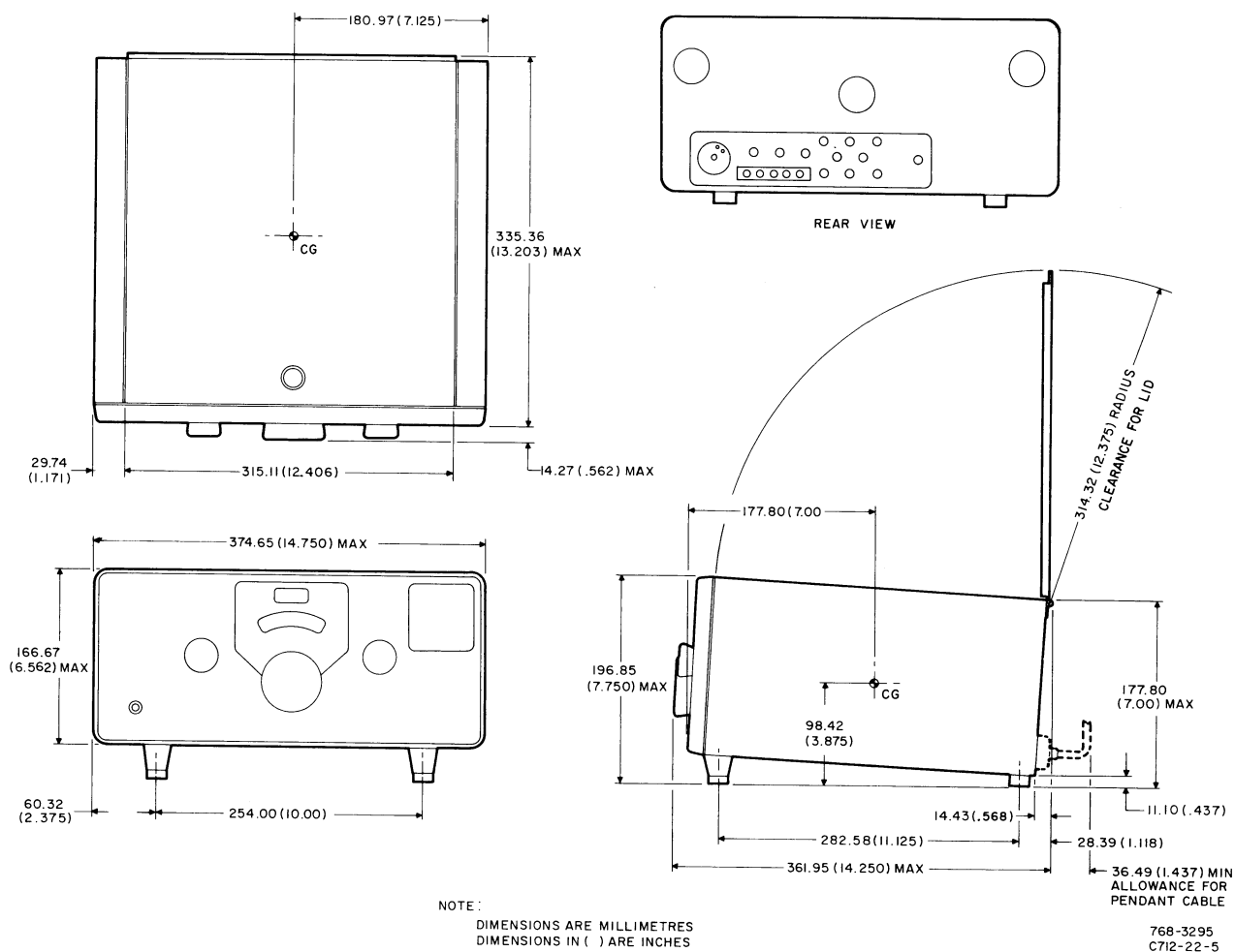
Figure 1-3. 51S-1/1A Receiver, Outline and Mounting Dimensions
