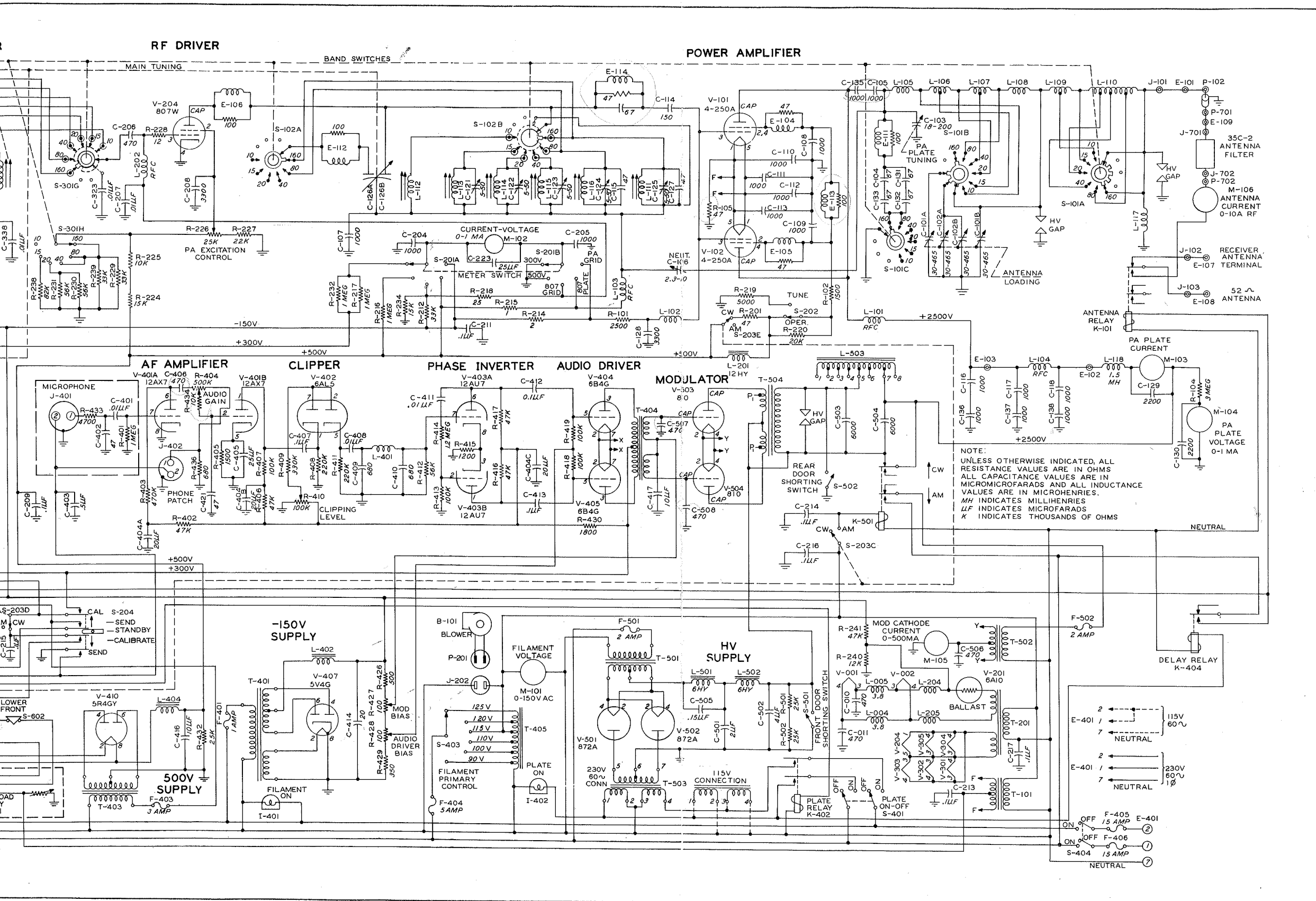
Figure 7-4. KW-1 Main Schematic
