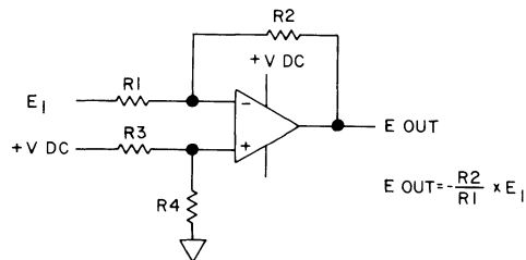
Figure 9-13.3. Inverting Amplifier with Offset Voltage.
