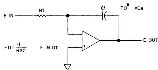
Figure 9-12.7. Integrator Circuit.
