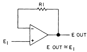
Figure 9-13.6. Unity Gain Amplifier.
