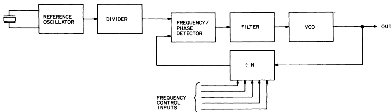
Figure 5-1. Basic Phase-Locked Loop Block Diagram.
