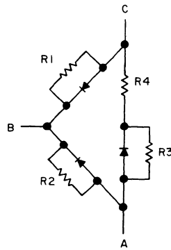
Figure 9-16.2. DC Equivalent of Transistor Circuit.
