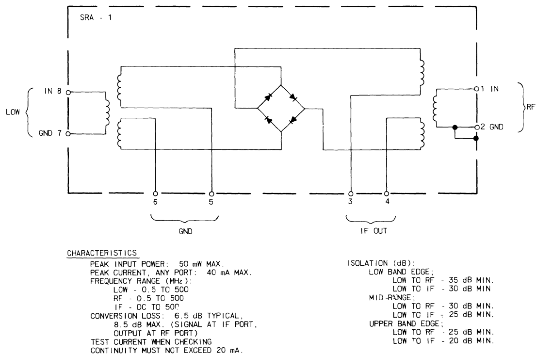
Figure 9-7.1. SRA-1 Double Balanced Mixer Simplified Schematic Diagram.
