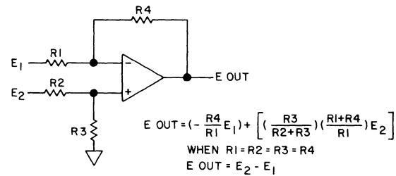
Figure 9-13.9. Difference Amplifier.
