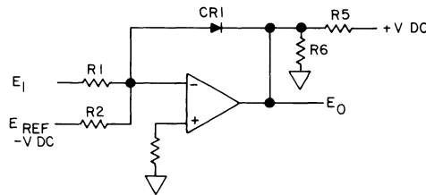
Figure 9-13.14. Voltage Comparator with Low and High Output Limiting.
