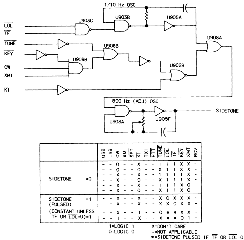
Figure 4-9. Side Tone Oscillator Diagram and Chart.
