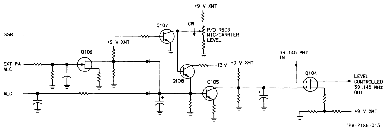
Figure 4-7. Exciter ALC Simplified Diagram.
