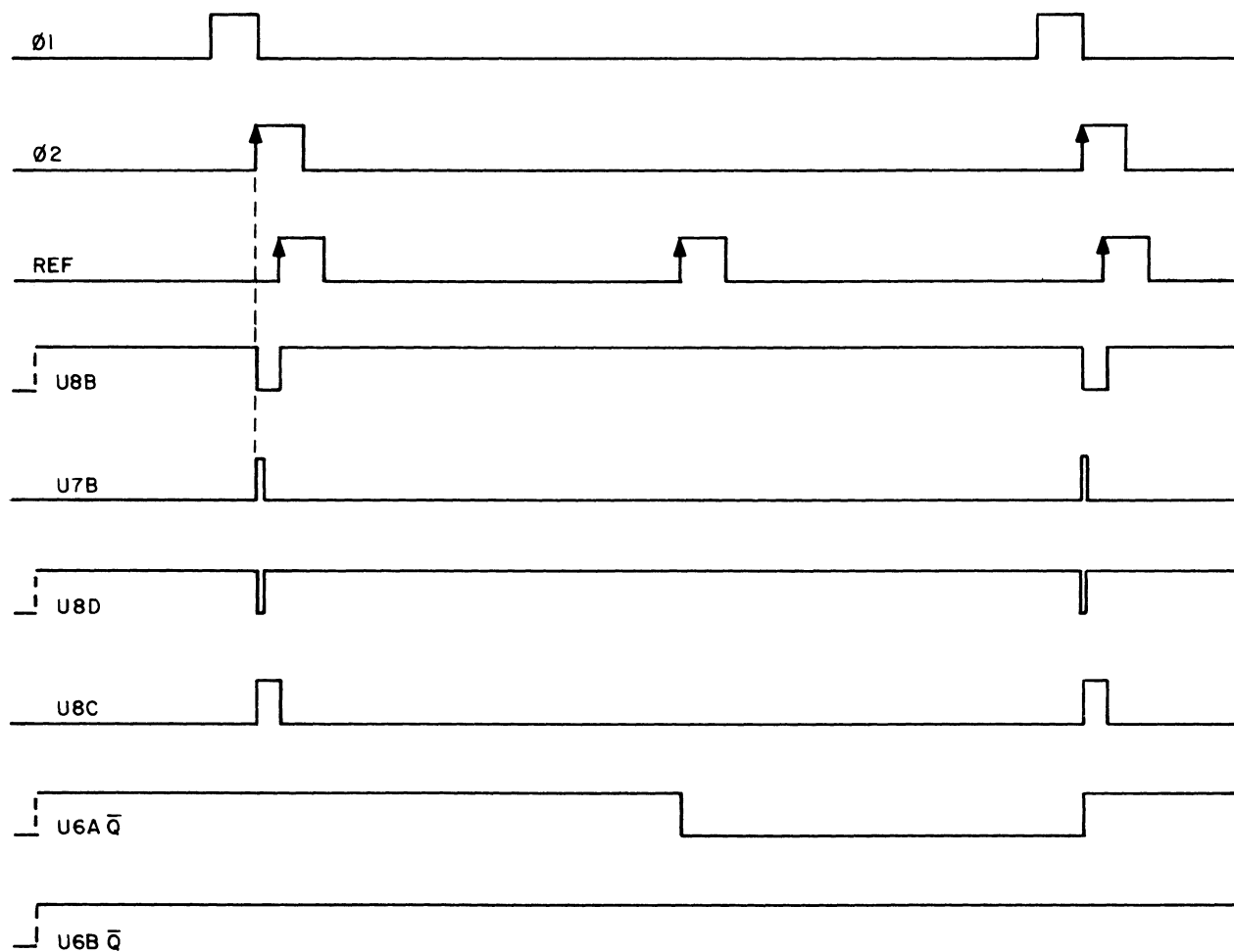
FREQ / Ø DET AND RAMP GEN. CONTROL
