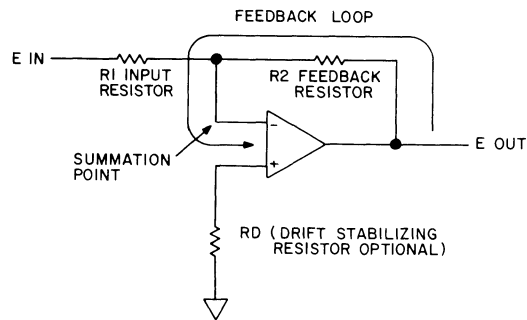
Figure 9-12.2. Circuit Notation.
