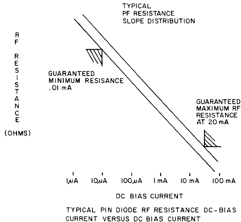
Figure 9-11.1. IN5767 Pin Diode Typical RF Resistance Slope Distribution.
