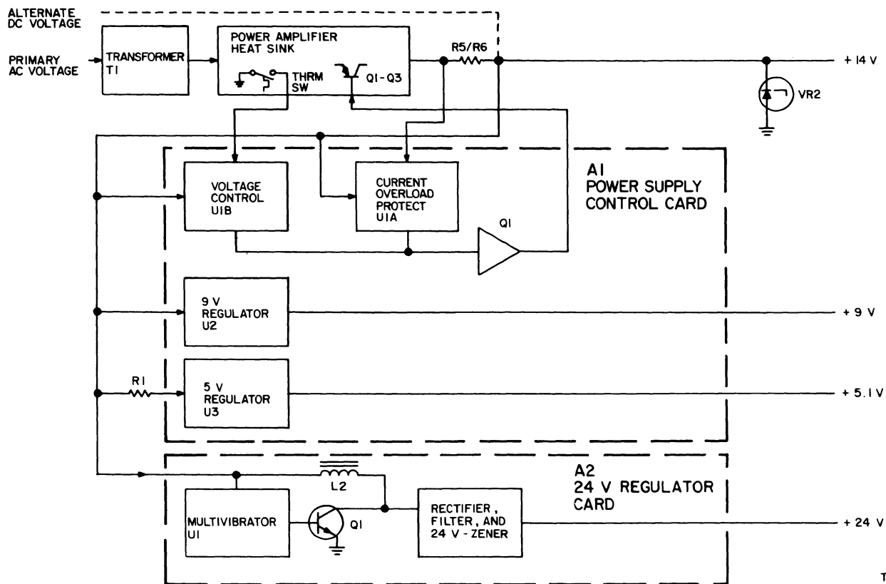
Figure 6-1. Power Supply Block Diagram.
