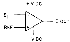
Figure 9-13.11. Voltage Comparator.
