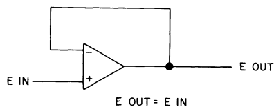
Figure 9-12.4. Voltage Follower.
