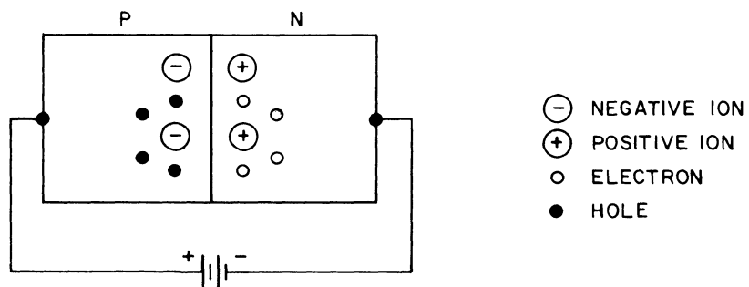
Figure 9-14.8. Forward Biased P-N Junction.
