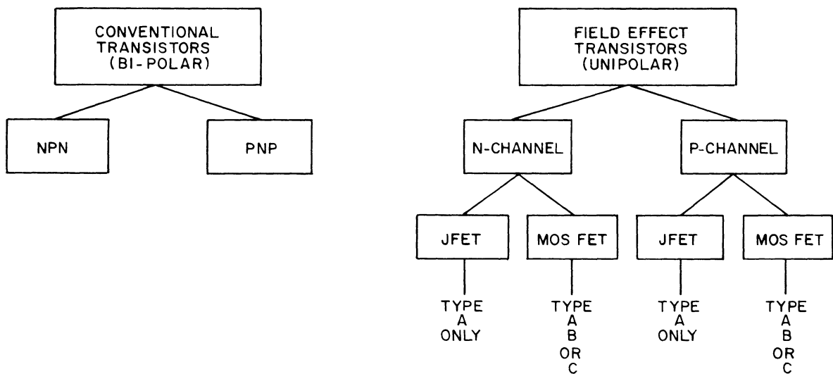
Figure 9-14.4. Classes of FETS.
