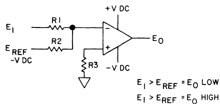
Figure 9-13.12. Voltage Comparator Using One Input.
