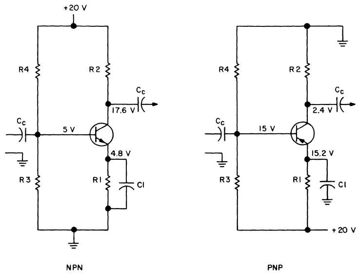
Figure 9-16.1. NPN and PNP Transistor Circuits.
