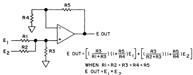
Figure 9-13.7. Noninverting Summing Amplifier.
