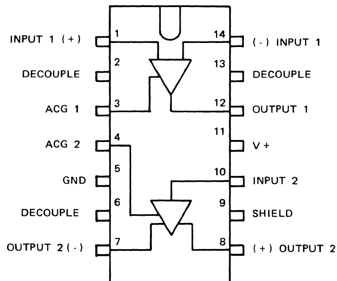
Figure 9-9.1. \mu A757 Connection Diagram.
