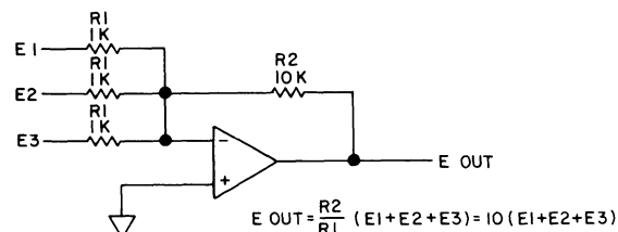
Figure 9-12.8. Voltage Adder.
