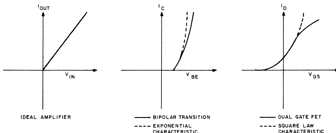
Figure 9-15.4. Transfer Characteristics of Amplifier.
