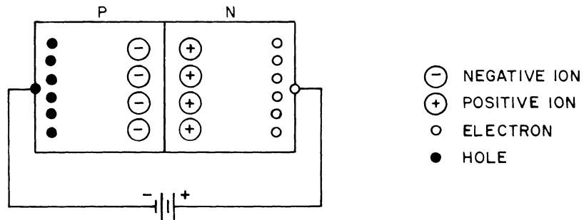
Figure 9-14.7. Reverse Biased P-N Junction.
