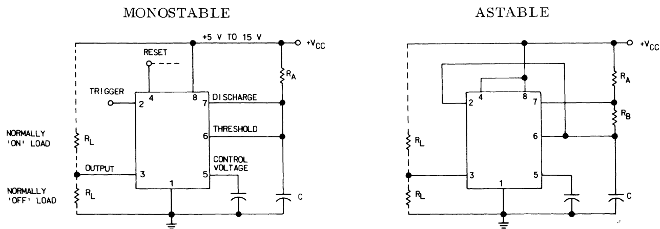
Figure 9-4.1. LM 555 Timer Diagram.
