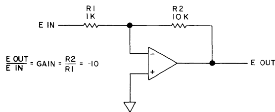
Figure 9-12.1. Inverting Amplifier.
