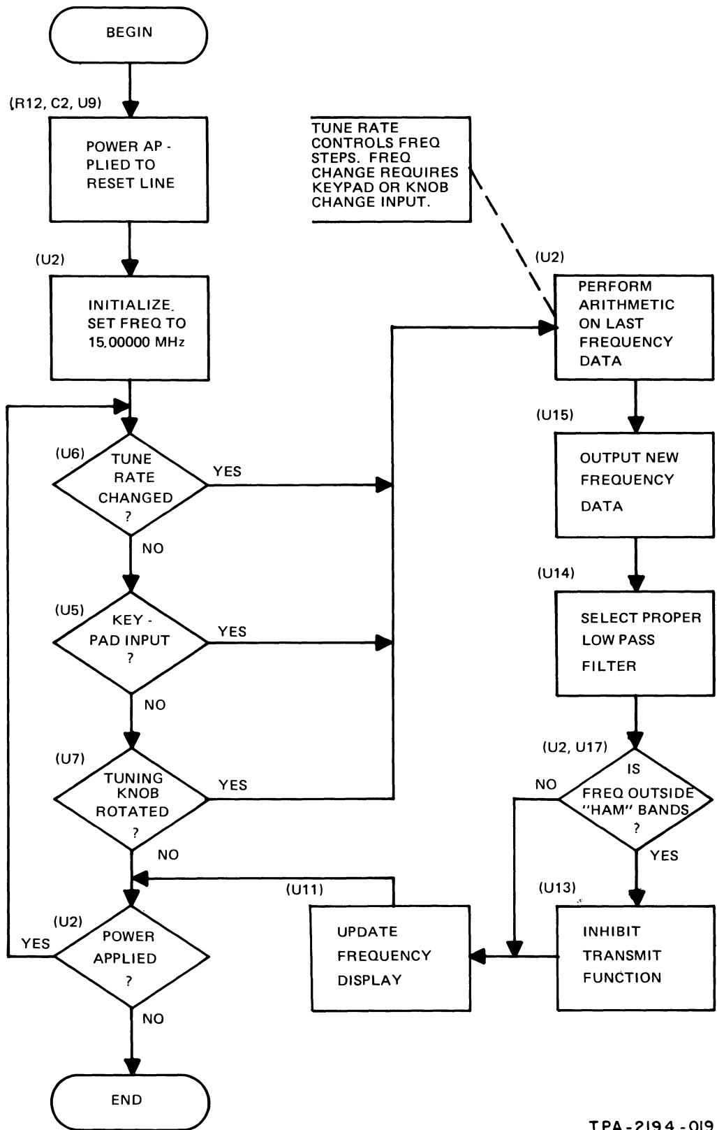
Figure 7-2. Microprocessor Operation Flow Chart.
