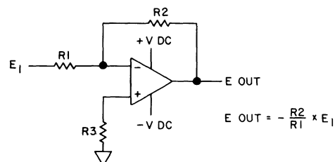
Figure 9-13.2. Inverting Amplifier with Added Temperature Stability.
