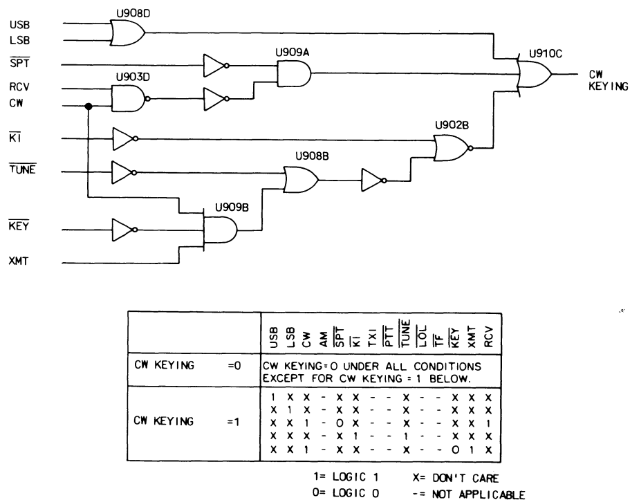
Figure 4-8. CW Keying Logic Diagram and Chart.
