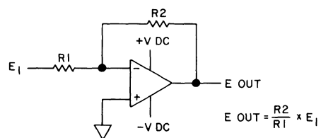
Figure 9-13.1. Inverting Amplifier.
