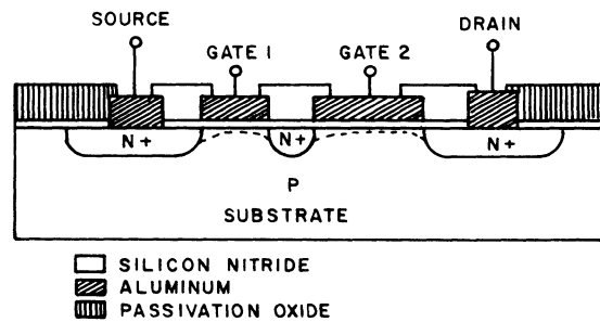
Figure 9-15.1. Dual-Gate MOS FET Cross Section.
