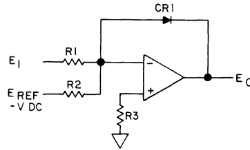
Figure 9-13.13. Voltage Comparator with Low Output Limiting.
