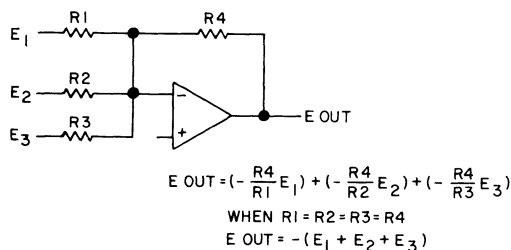
Figure 9-13.8. Inverting Summing Amplifier.
