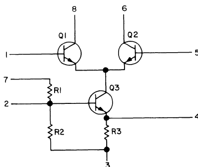
Figure 9-8.1. CA3028 Product Detector Simplified Schematic.
