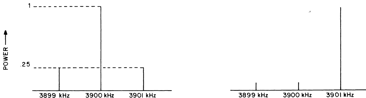
Figure 9-2.1. Comparison of AM and SSB Spectra.
