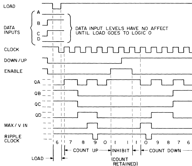
Figure 9-5.2. Programmable Divider Counter Operation.
