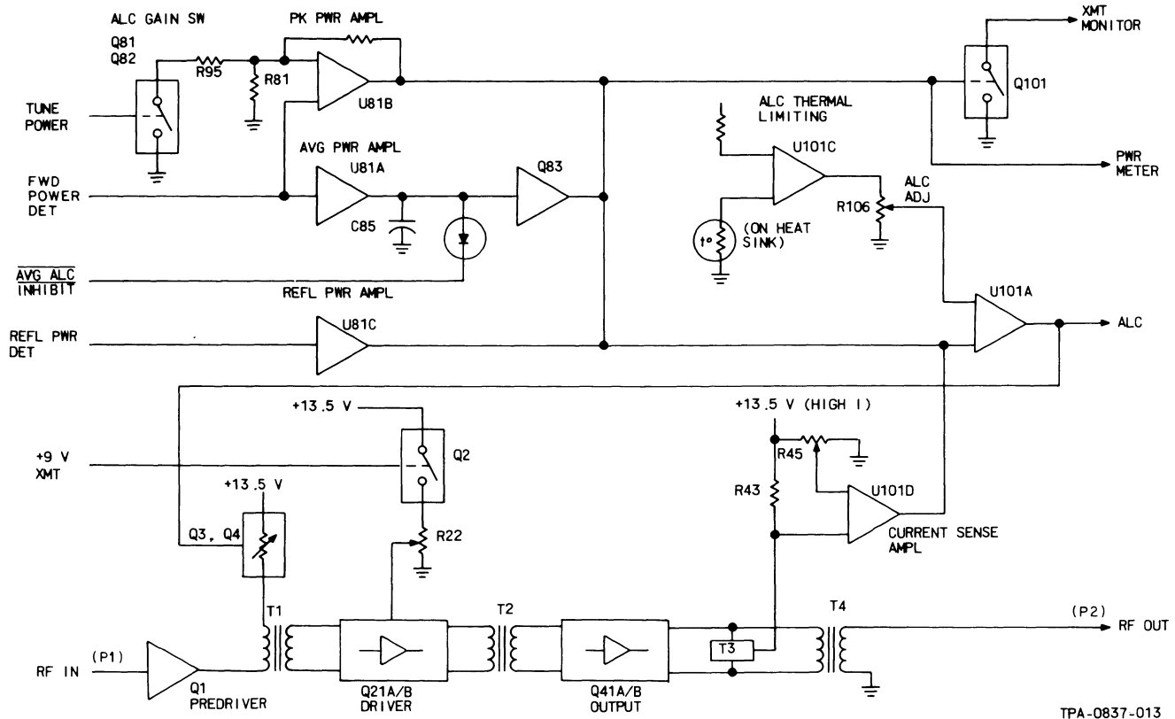
Figure 4-10. Power Amplifier and Block Diagram.
