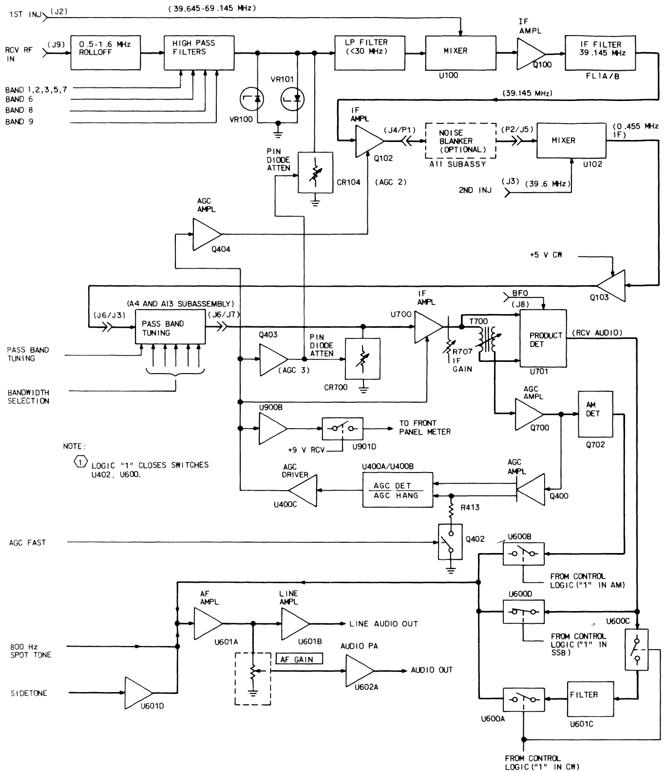
Figure 3-3. Receive Signal Path Block Diagram.
