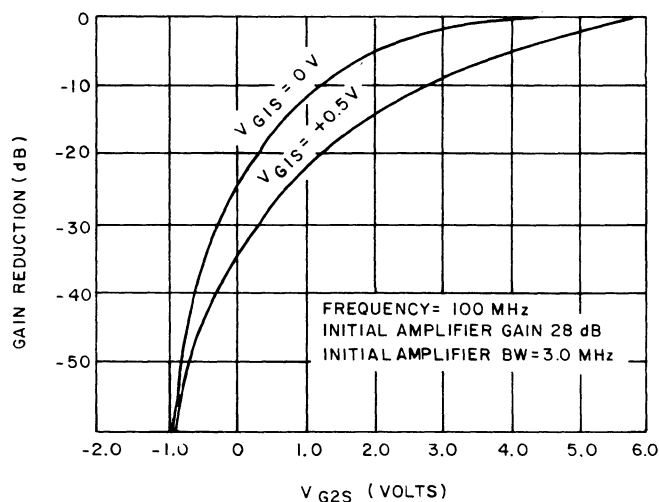
Figure 9-15.3. Gate 2 AGC Gain Reduction.
