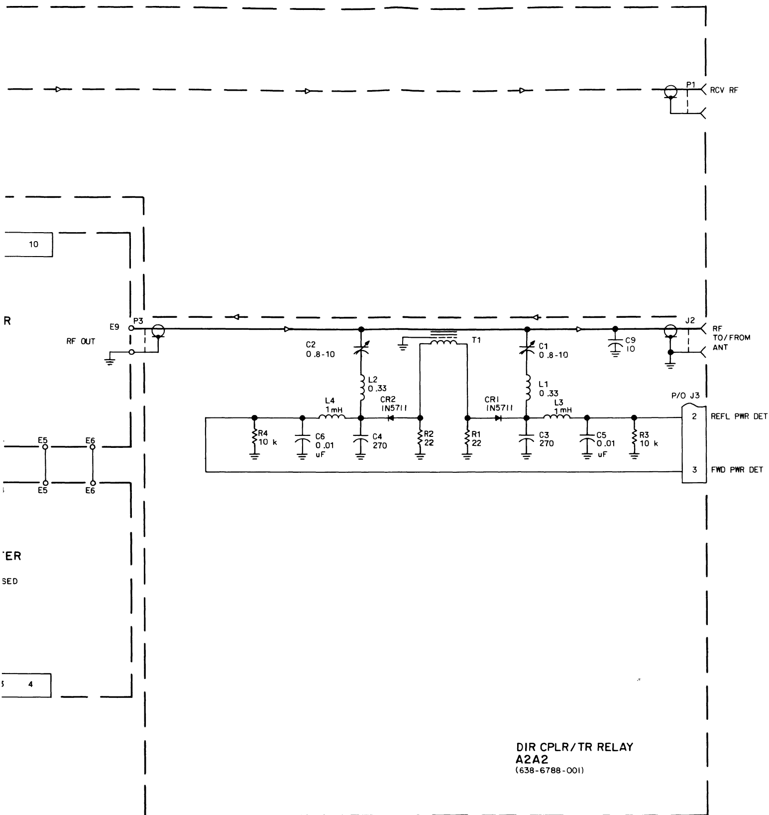
Figure 4-11. Low-Pass Filter Diagram.
