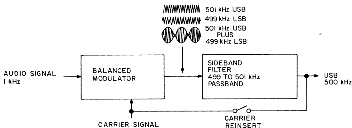
Figure 9-2.4. Filter-Type SSB Generator.
