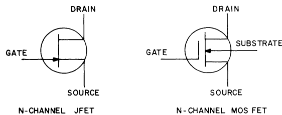
Figure 9-14.2. FJET and MOS FET Symbols.
