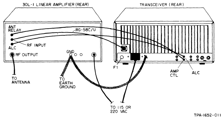
Figure 1-4. Interconnection for Transceiver and Linear Amplifier.
