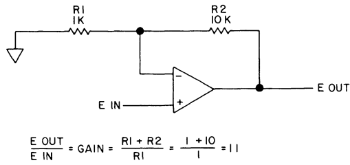
Figure 9-12.3. Noninverting Amplifier.
