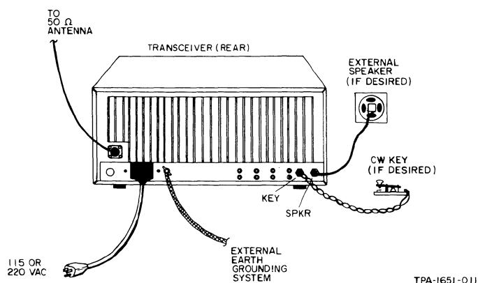
Figure 1-3. Interconnection for Transceiver Alone.
