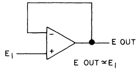
Figure 9-13.5. Unity Gain Amplifier.
