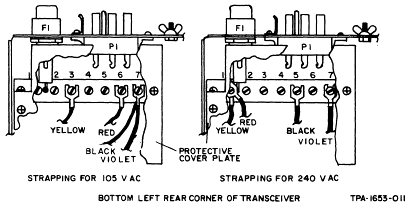
Figure 1-6. AC Input Strapping on TB1.
