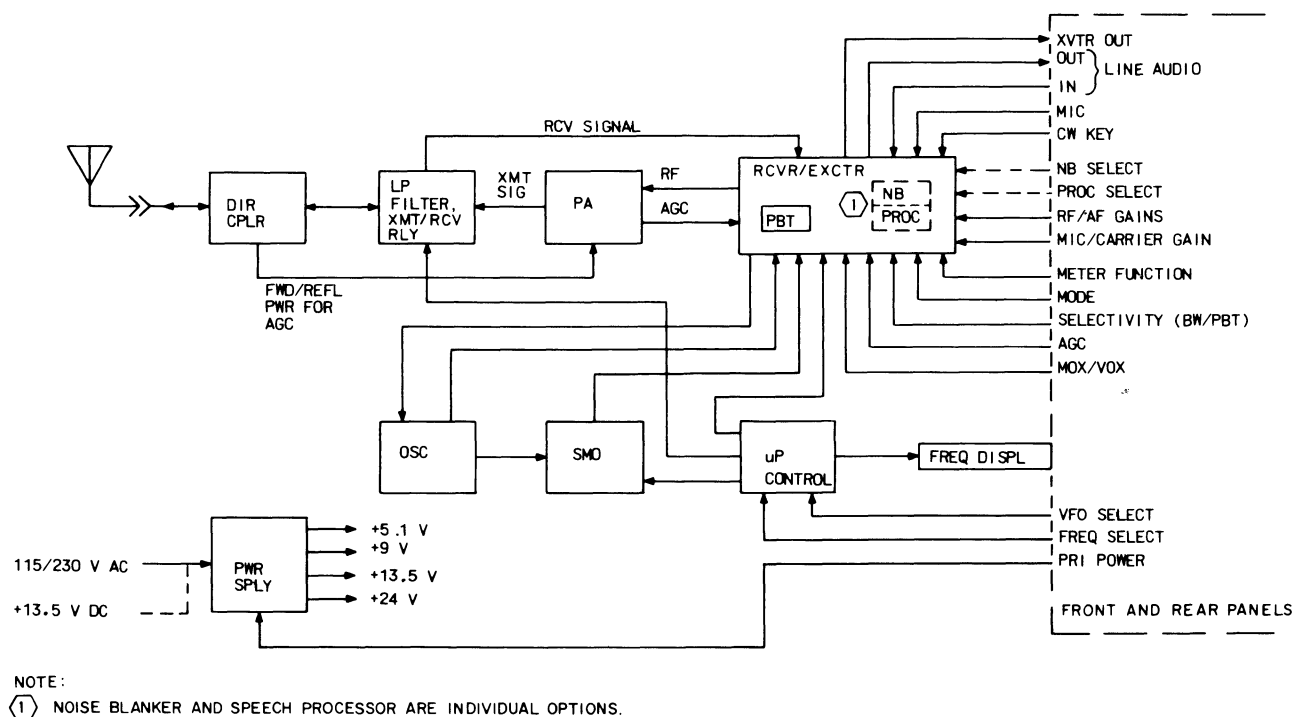
Figure 4-1. KWM-380 Simplified Block Diagram.
