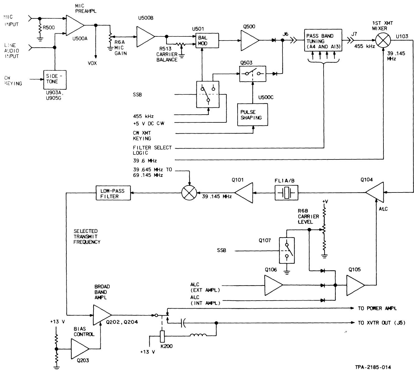
Figure 4-2. Transmit Signal Path Block Diagram.
