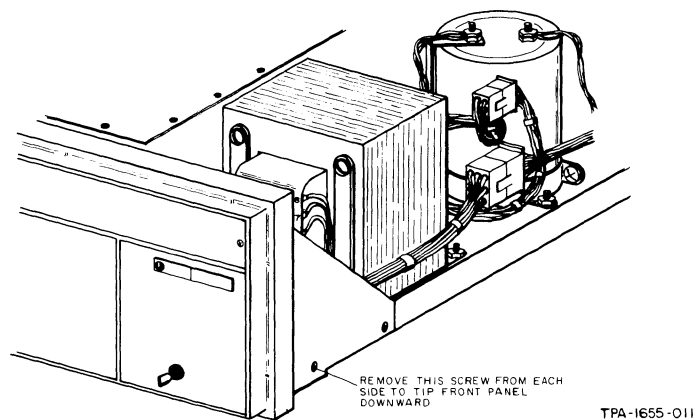
Figure 1-5. Power Transformer Installation.
