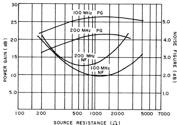
Figure 9-15.2. Dual-Gate Power Gain -- Source Resistance.
