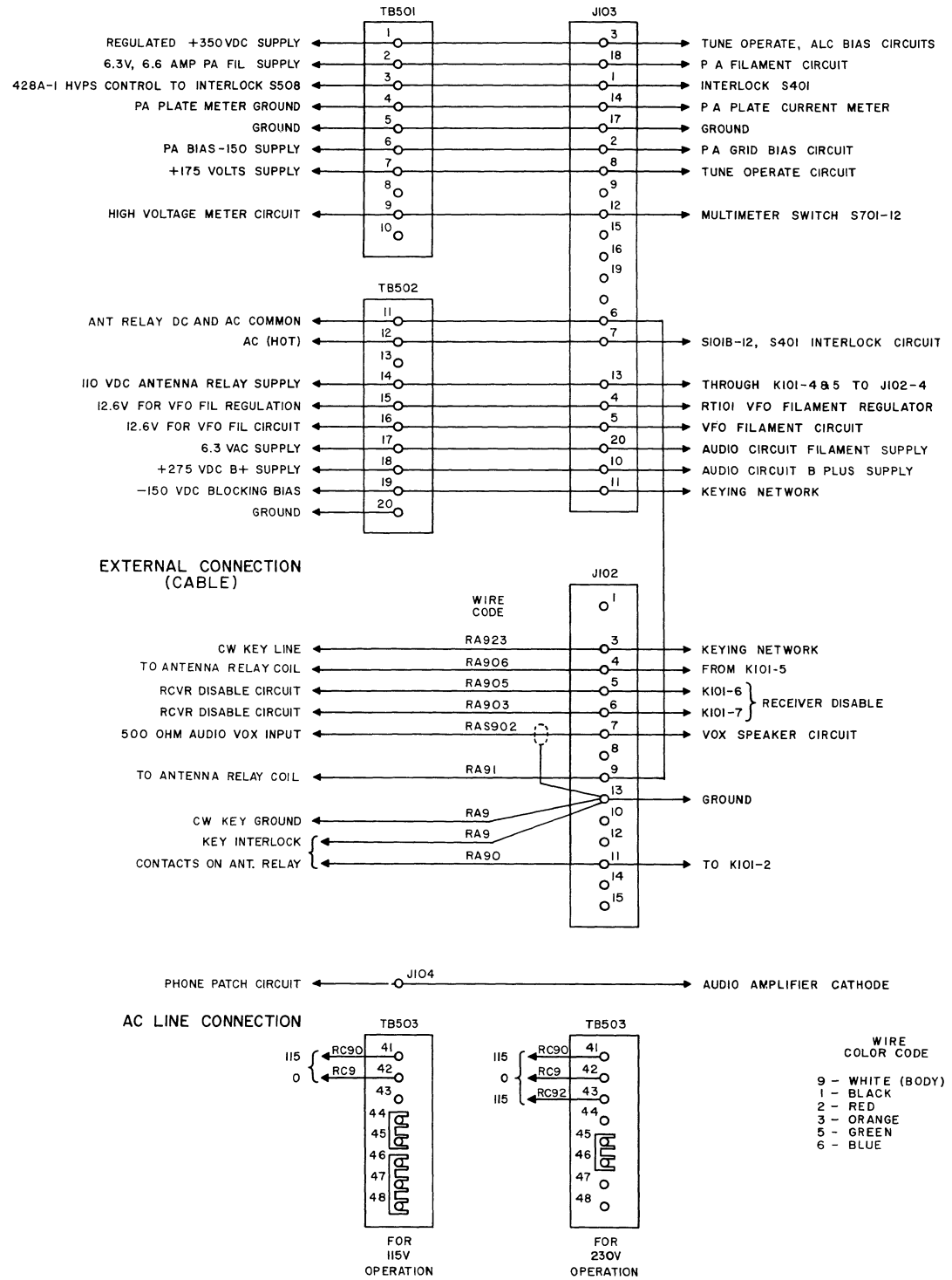
Figure 7-3. Interconnecting Cable Wiring Diagram
