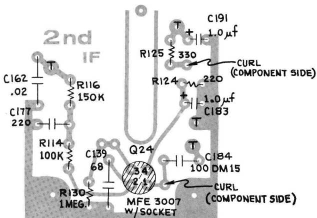
2nd IF AMPLIFIER CIRCUIT BOARD
