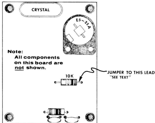
RY-4 CALIBRATION CONNECTION TO SPR-4
