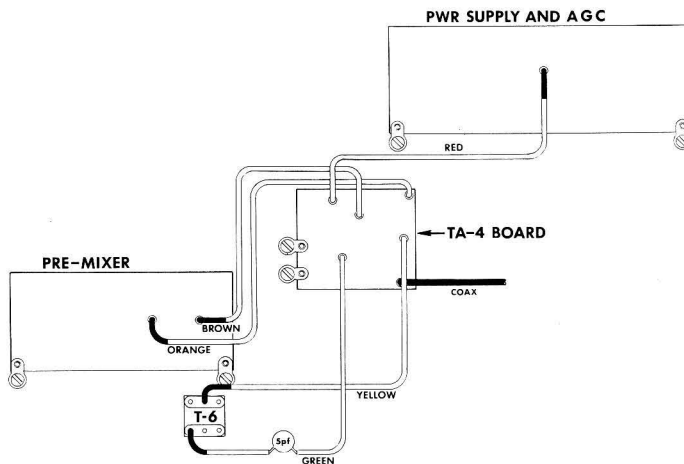
TA-4 PICTORIAL WIRING DIAGRAM
