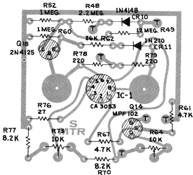
S-METER CIRCUIT BOARD
