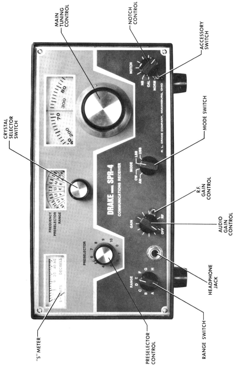
FRONT PANEL OPERATING CONTROLS
