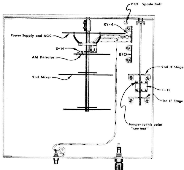
RY-4 CIRCUIT BOARD INSTALLATION DIAGRAM Figure 12
