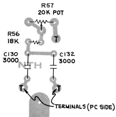
NOTCH FILTER CIRCUIT BOARD
