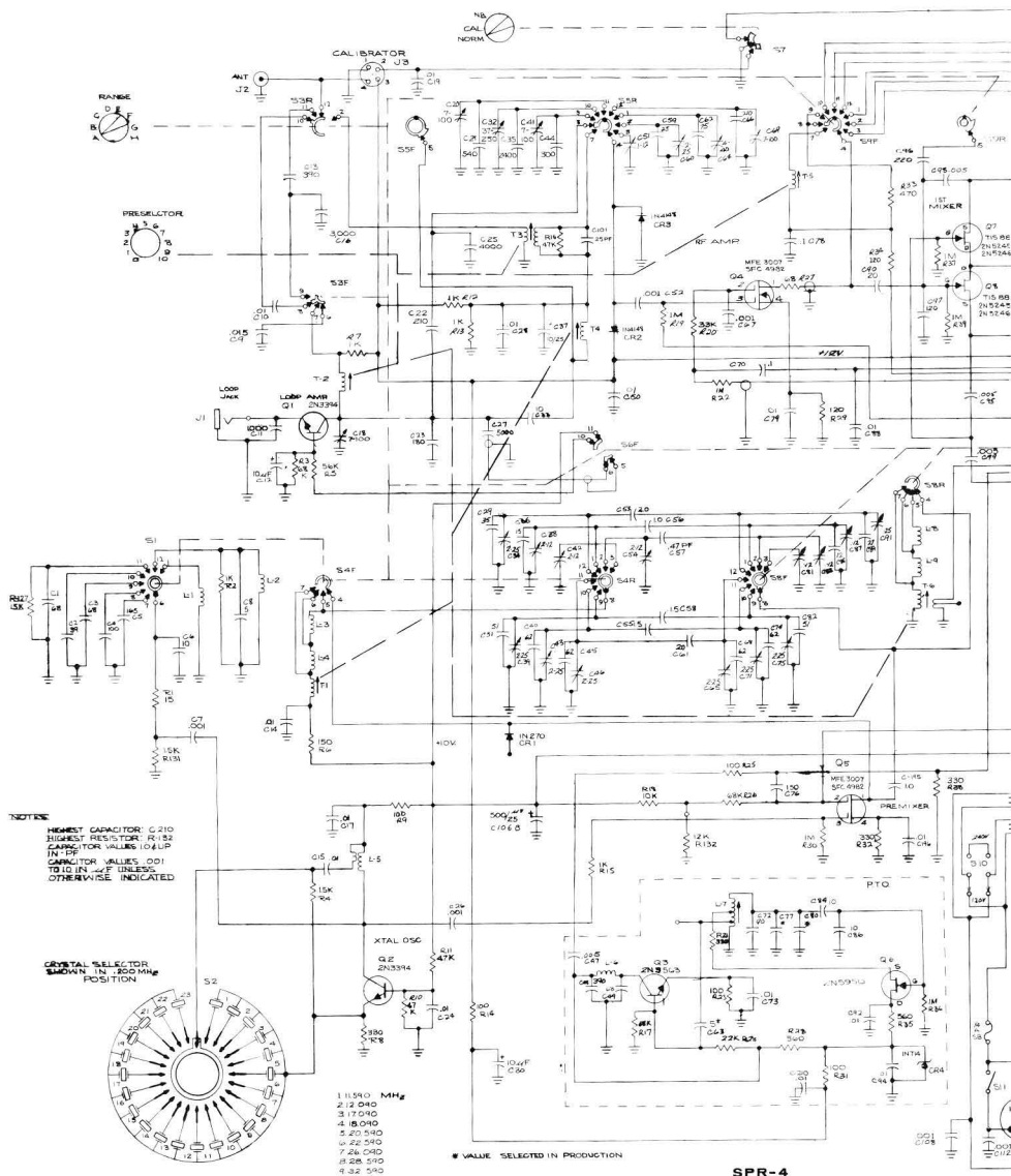
SPR-4 SCHEMATIC DIAGRAM
