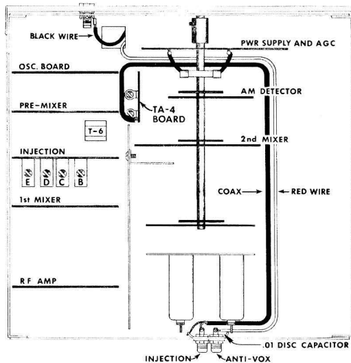
TA-4 CIRCUIT BOARD INSTALLATION DIAGRAM
