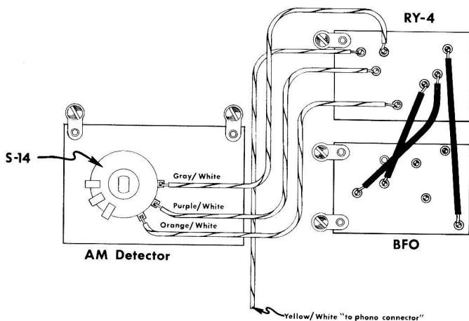
RY-4 PICTORIAL WIRING DIAGRAM Figure 13
