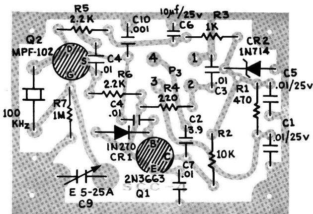
SCC-4 CIRCUIT BOARD
