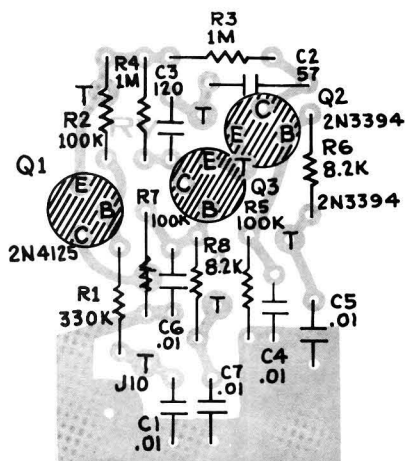
RY-4 CIRCUIT BOARD
