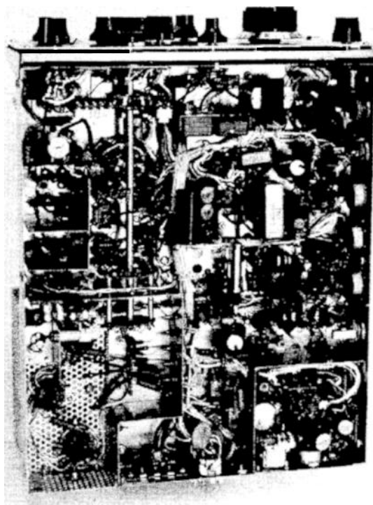
Bottom of the TR-6, with the final amplifier stage in the lower left corner. Jacks for phones, key and microphone are along the right side of the chassis, as are controls for VOX, antivoix and S-meter zero adjustment. The power source plugs onto a fitting on the rear wall. The socket in the upper right-center is for connecting the remote vfo, if used. Plug-in crystals and their range-selector switch are in the upper left-center.
