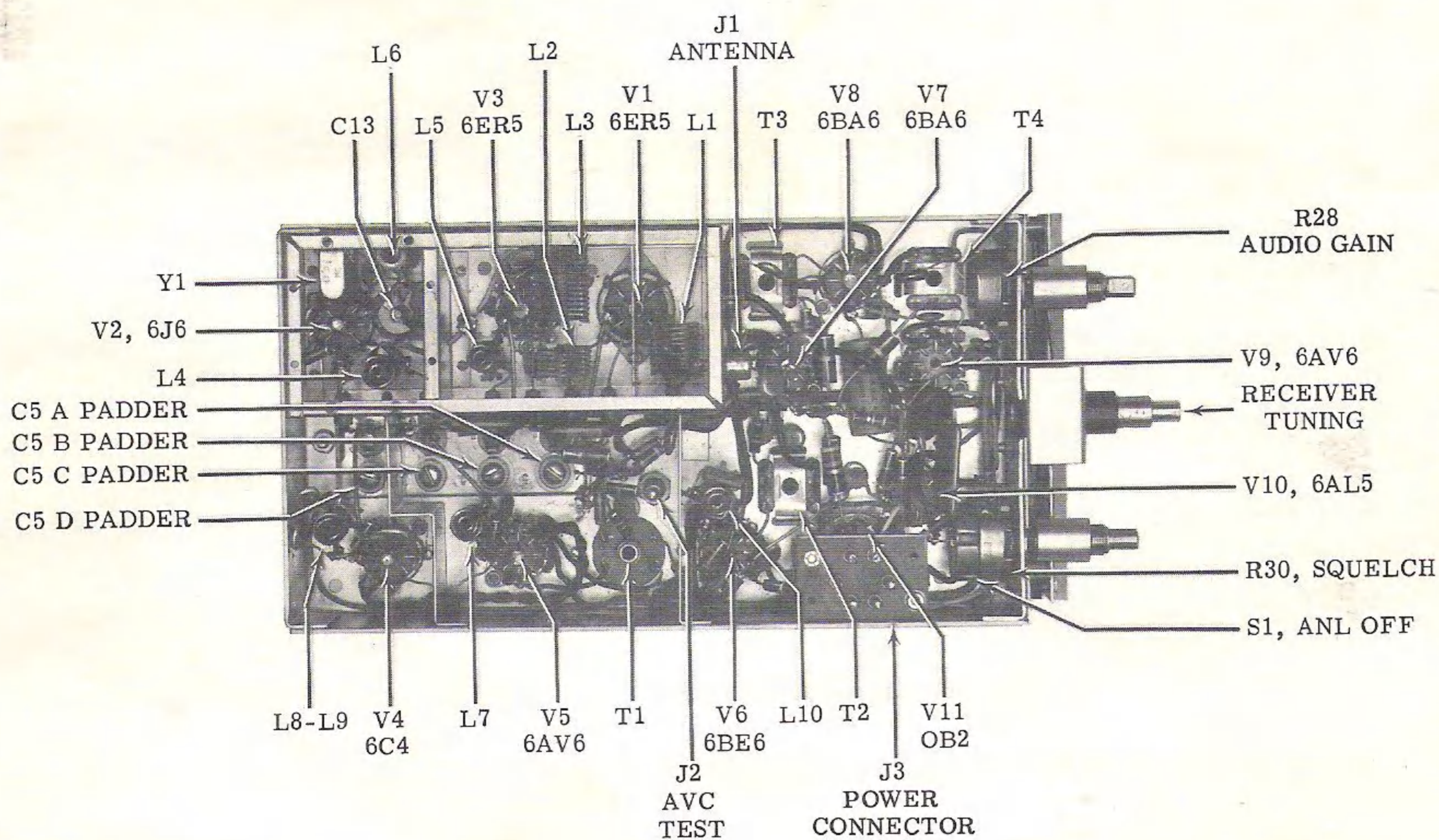
FIG. 5, RECEIVER SUB CHASSIS, BOTTOM VIEW
