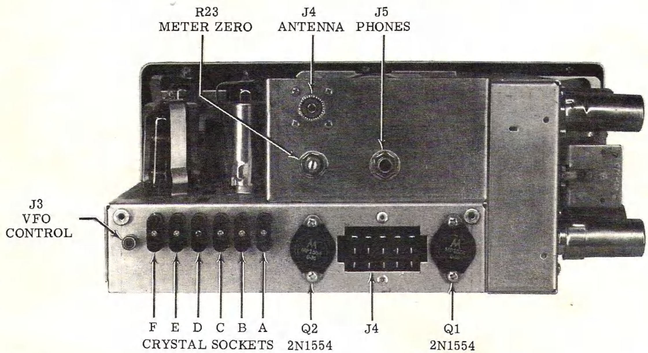
FIG. 2, CHASSIS, REAR VIEW
