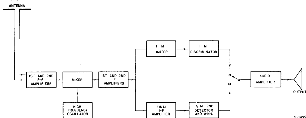
Fig. 4-1. Radio Receiver Model S-37, block diagram
