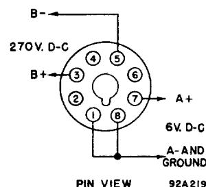
Fig. 2-1. Radio Receiver Model S-37, wiring diagram for d-c power plug.
